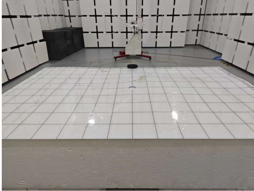
Set-up for Radiated Spurious Emission, Above 1GHz
