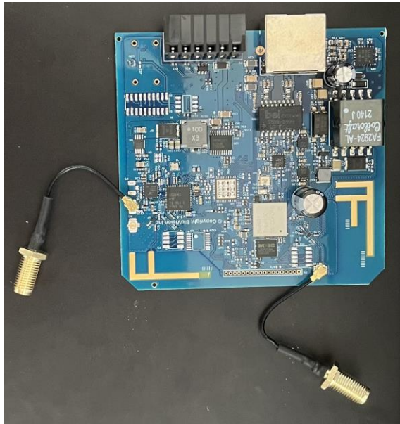
BluFi™ POE 5G PCB bottom view
