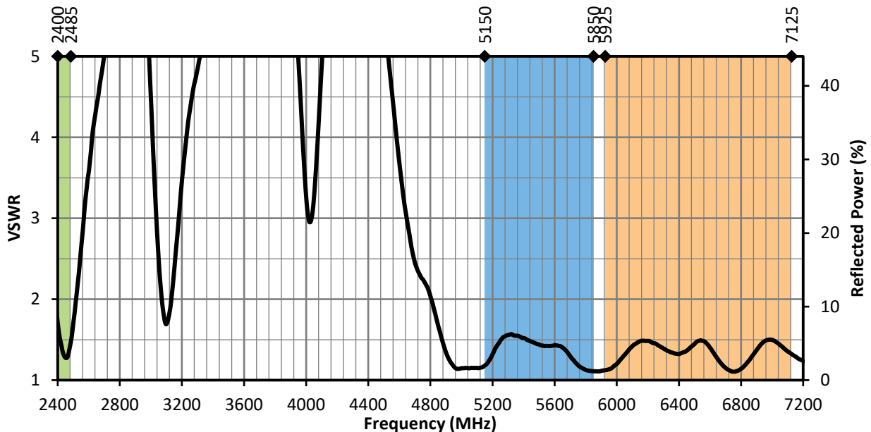
Figure 4. ANT-W63WS6-IPW1-ccc VSWR, Straight
