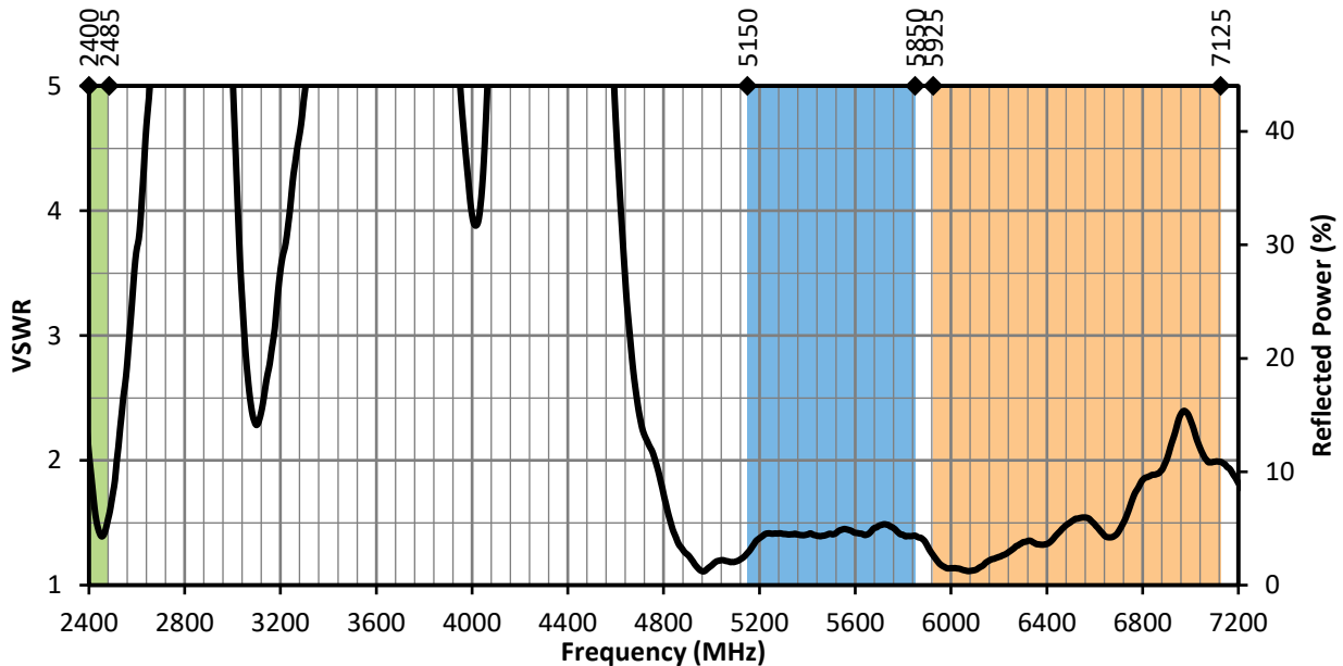
Figure 11. ANT-W63WS6-IPW1-ccc VSWR, Edge-Bent
