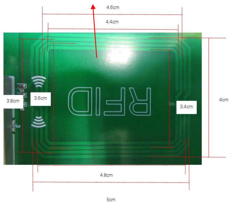
Antenna dimension design
