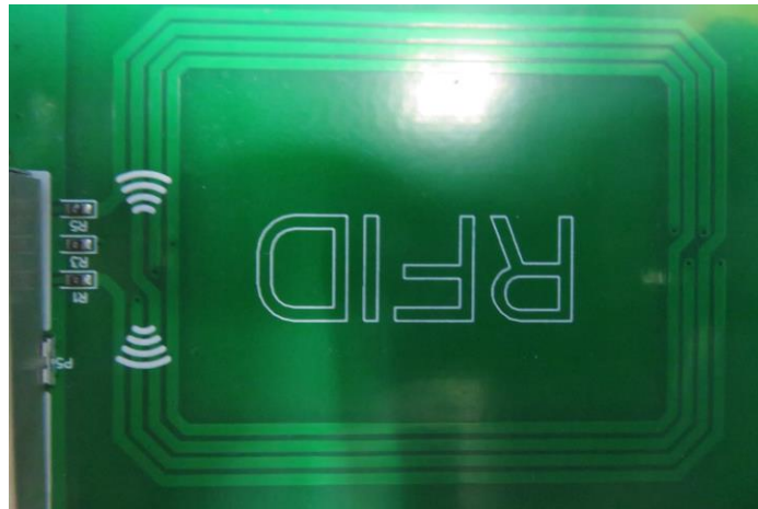
Antenna dimension design
