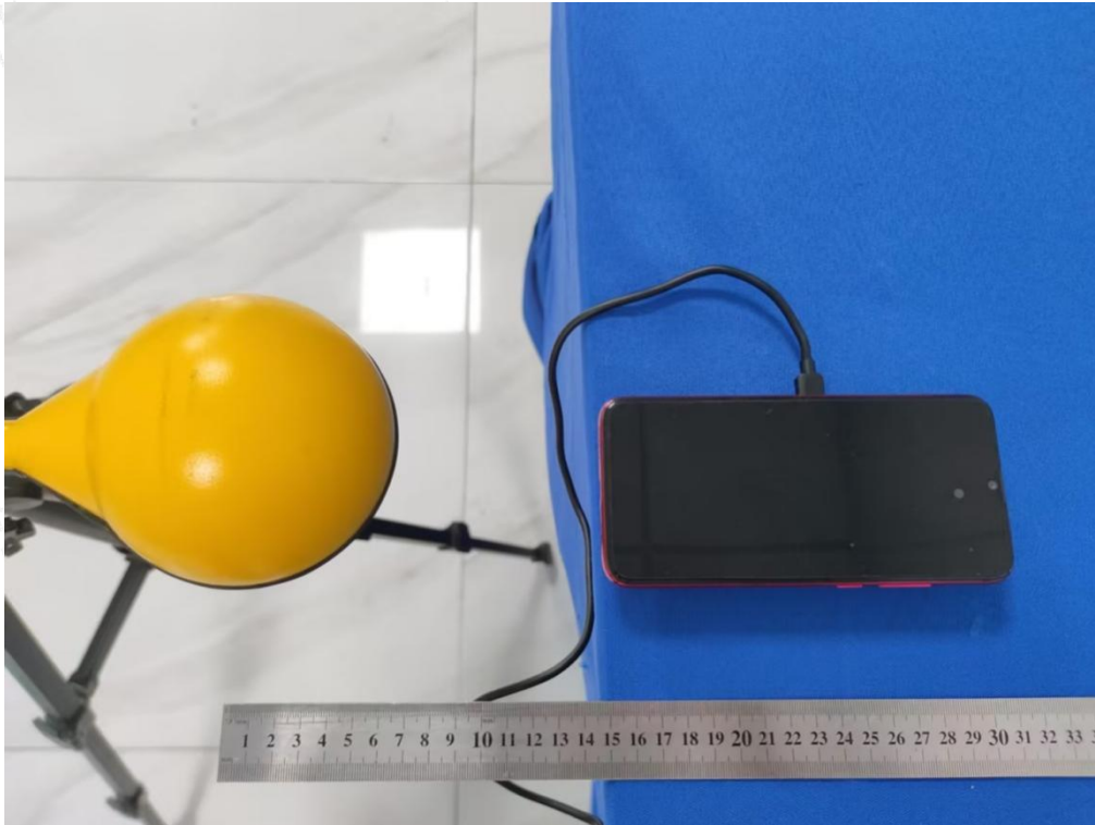
Test Position E(15cm) - Exposure photo from side edge surface-Right(TM1) H-Field Strength:
