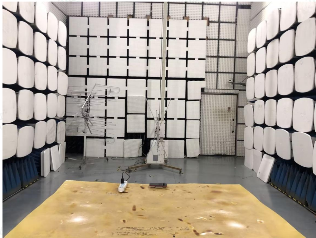
Radiated Emission below 1GHz-TM1
