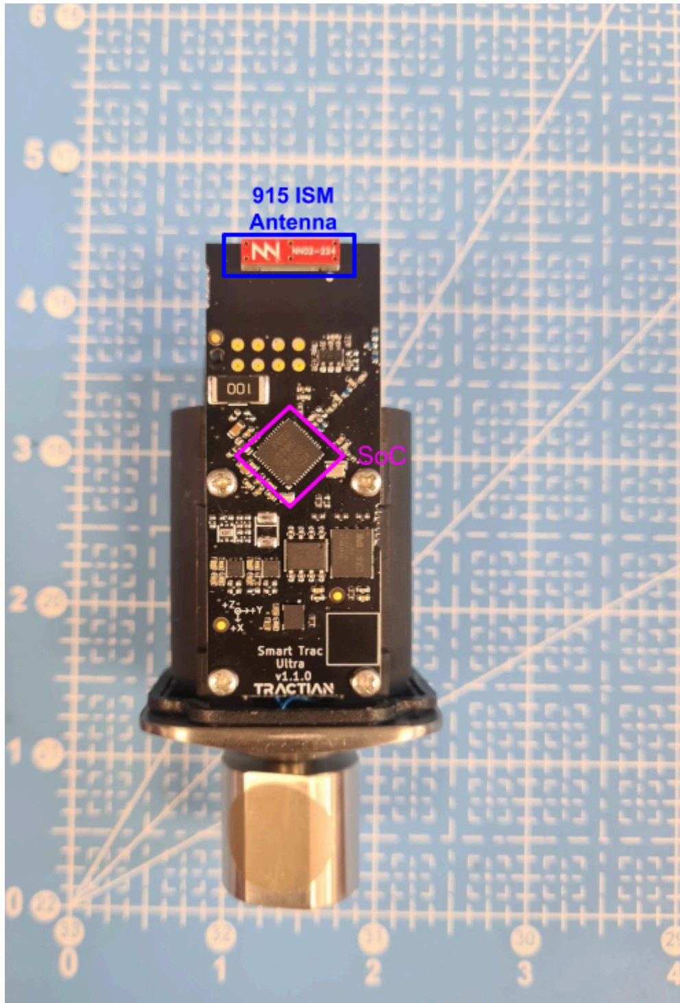
Figure 1 - Smart Trac Ultra - Internal - Front View
