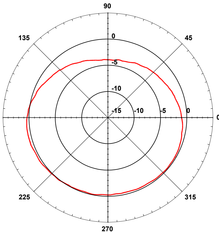
Total field (dBi)
