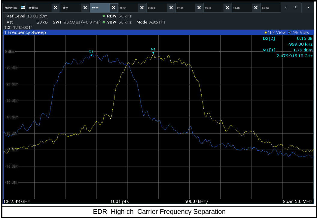
EDR_High ch_Carrier Frequency Separation
