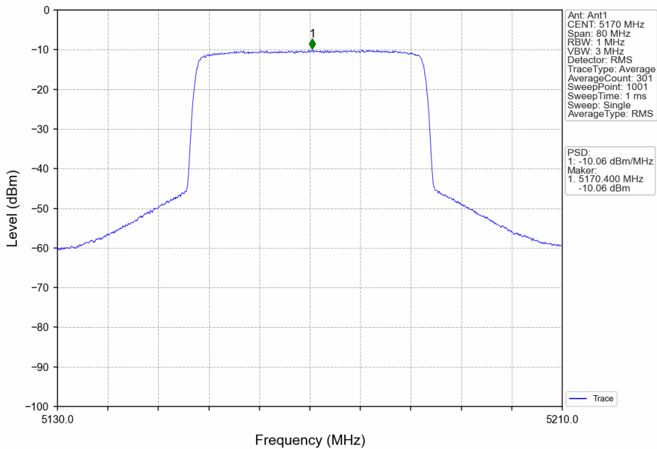
40M_LCH_5170MHz_Ant1_NTNV
