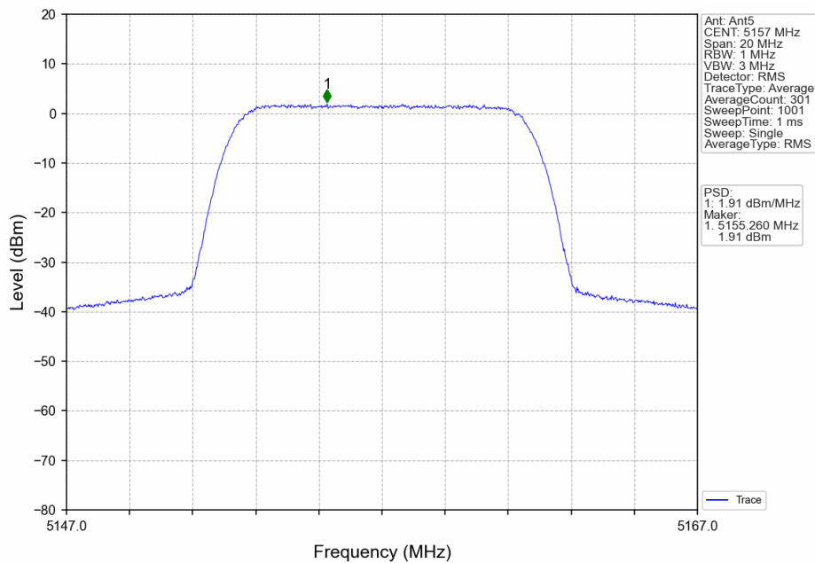
10M_LCH_5157MHz_Ant5_NTNV
