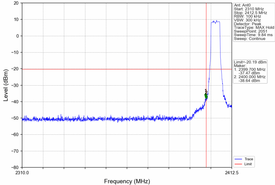
5M_LCH_2404.5MHz_Ant0_NTNV
