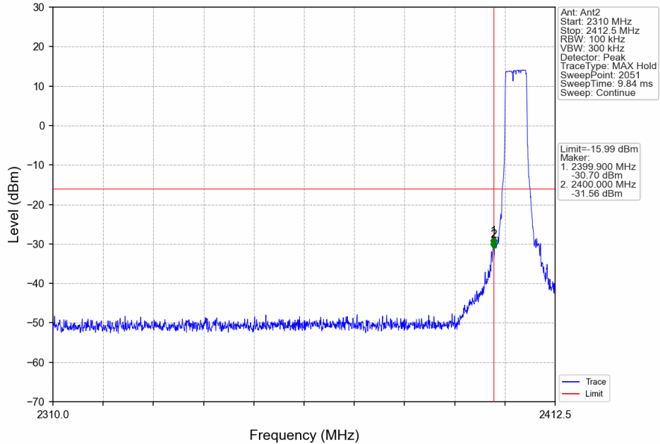
5M_LCH_2404.5MHz_Ant2_NTNV
