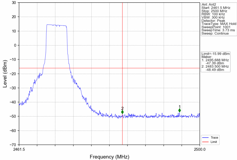
5M_HCH_2469.5MHz_Ant2_NTNV
