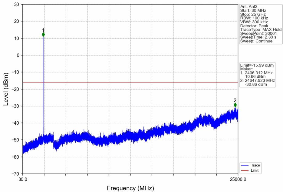
5M_LCH_2404.5MHz_Ant2_NTNV
