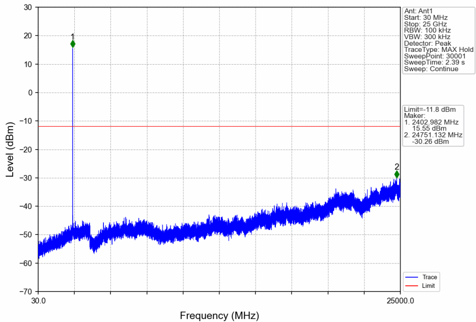
1.4M_LCH_2403.5MHz_Ant1_NTNV
