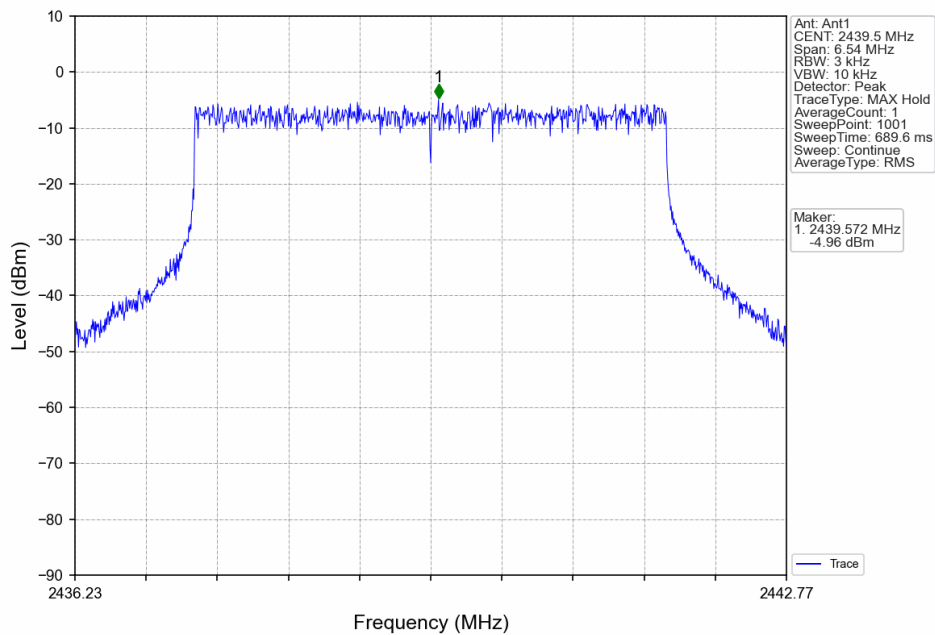
5M_MCH_2439.5MHz_Ant1_NTNV
