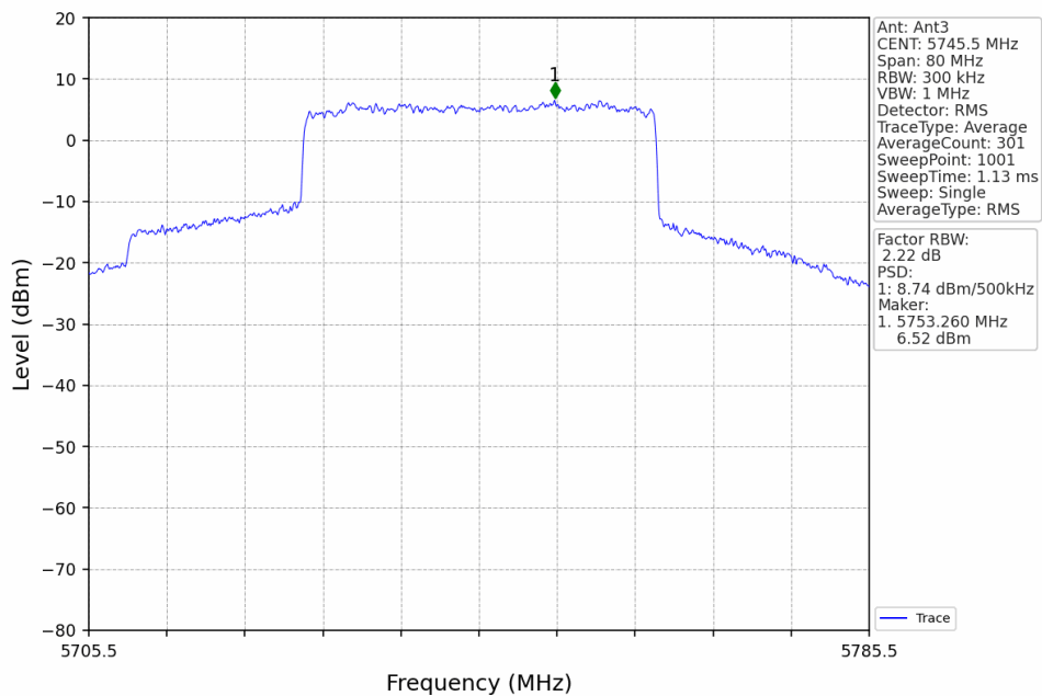
40M_LCH_5745.5MHz_Ant3_NTNV
