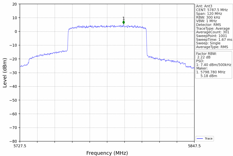
60M_MCH_5787.5MHz_Ant3_NTNV
