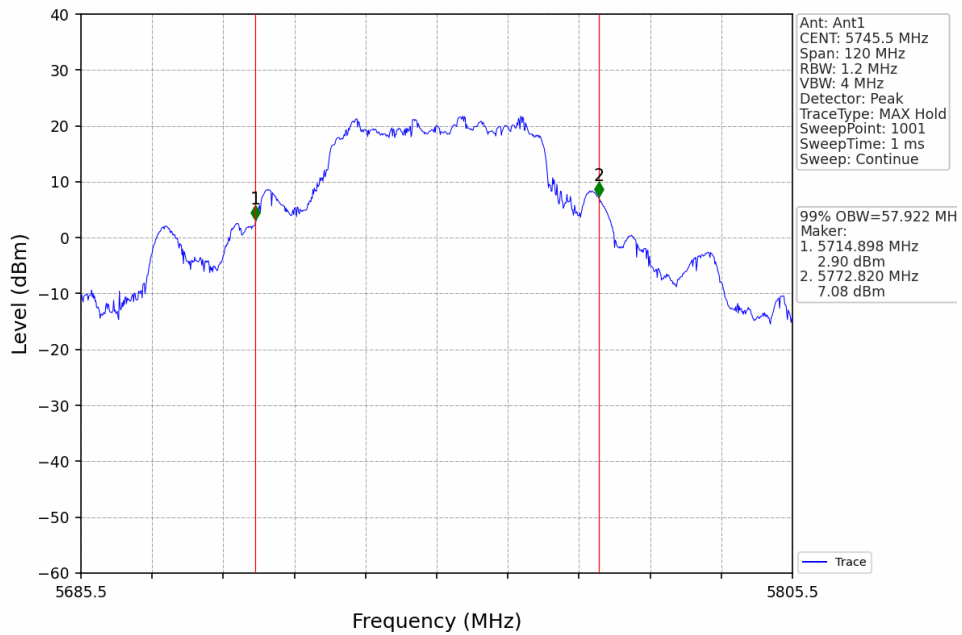
40M_LCH_5745.5MHz_Ant1_NTNV
