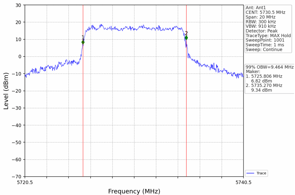
10M_LCH_5730.5MHz_Ant1_NTNV
