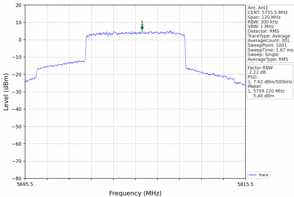
60M_LCH_5755.5MHz_Ant1_NTNV
