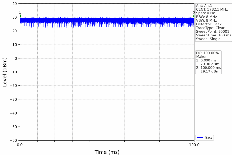
5M_MCH_5782.5MHz_Ant1_NTNV
