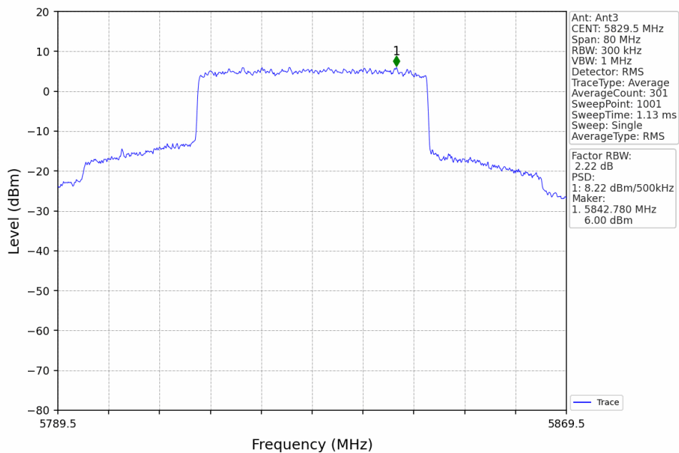
40M_HCH_5829.5MHz_Ant3_NTNV
