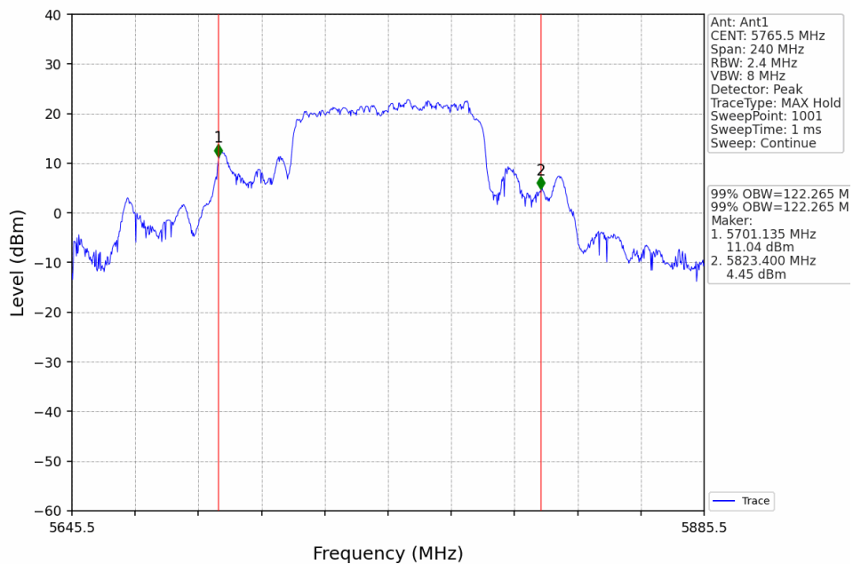
80M_LCH_5765.5MHz_Ant1_NTNV
