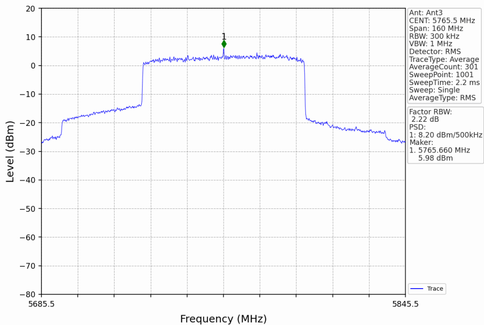
80M_LCH_5765.5MHz_Ant3_NTNV
