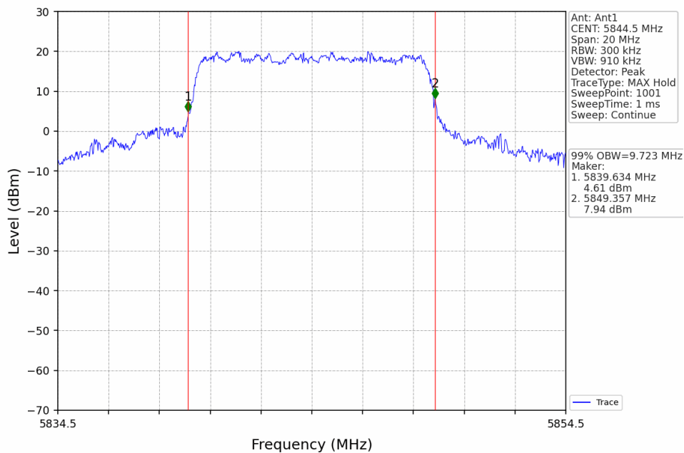
10M_HCH_5844.5MHz_Ant1_NTNV
