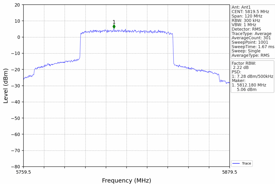
60M_HCH_5819.5MHz_Ant1_NTNV
