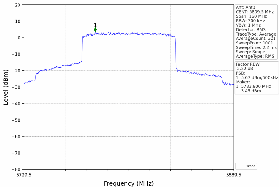
80M_HCH_5809.5MHz_Ant3_NTNV
