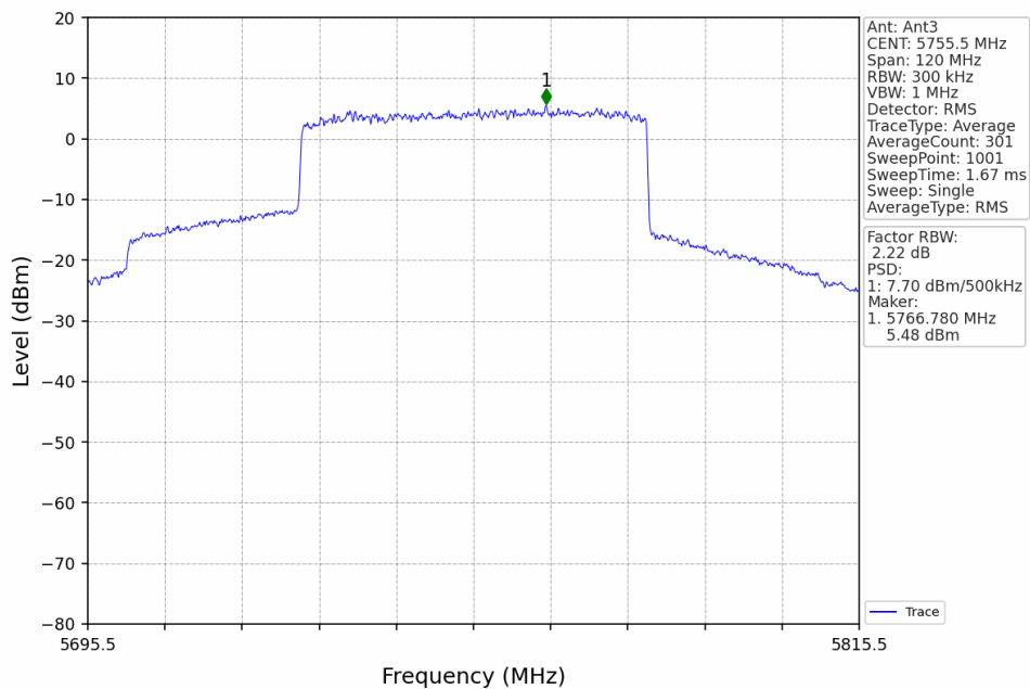
60M_LCH_5755.5MHz_Ant3_NTNV
