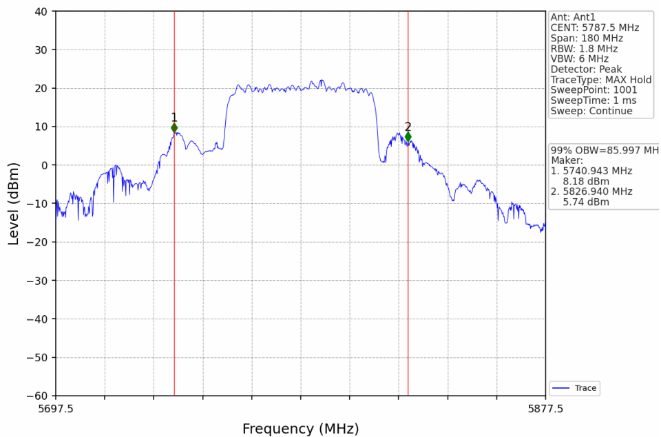
60M_MCH_5787.5MHz_Ant1_NTNV
