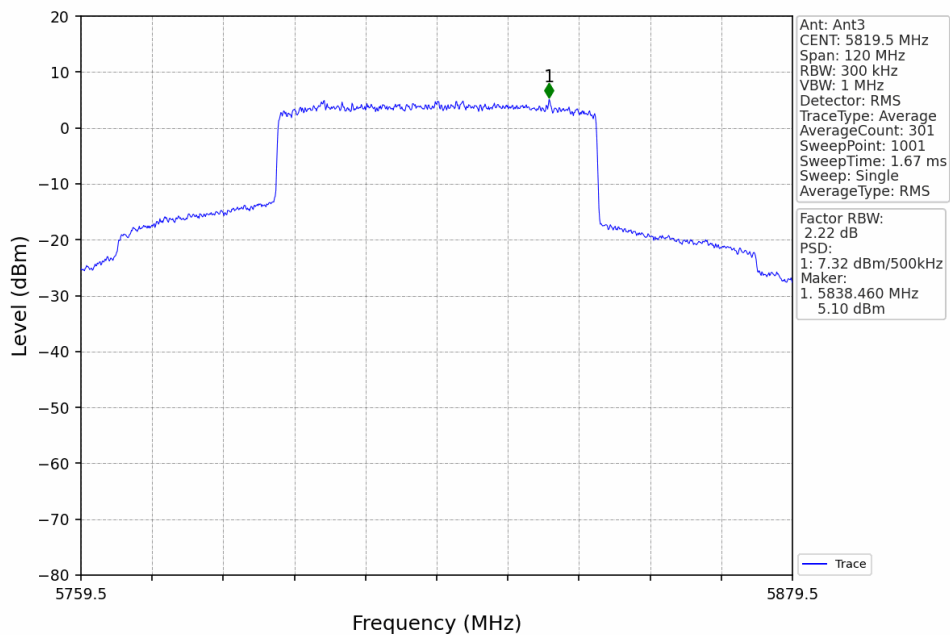
60M_HCH_5819.5MHz_Ant3_NTNV
