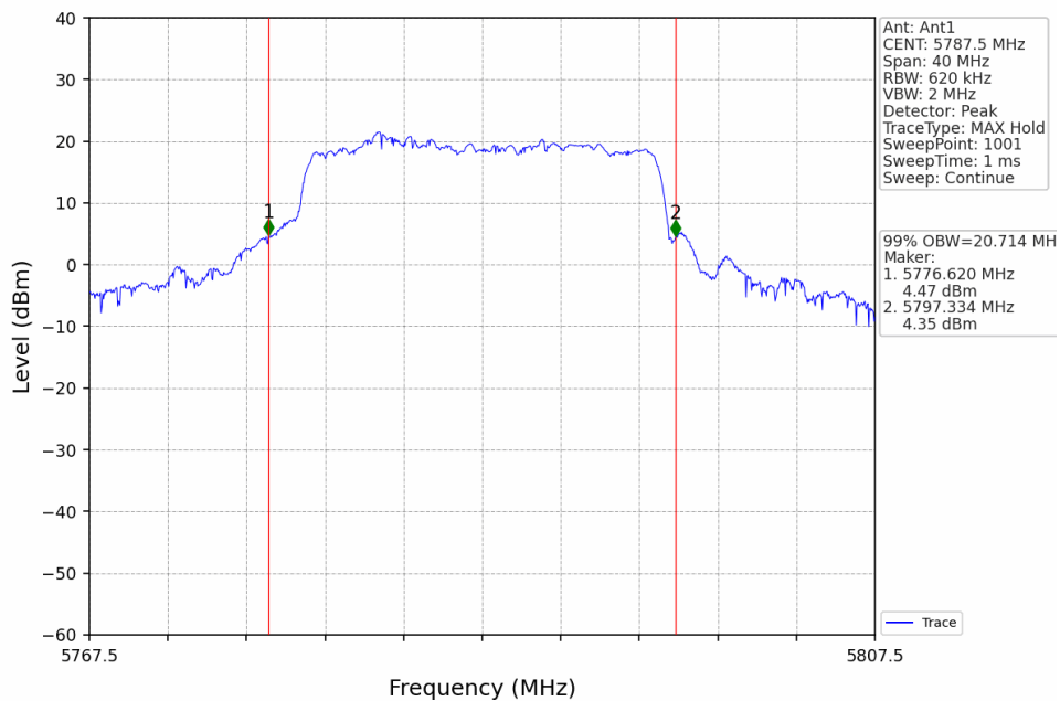
20M_MCH_5787.5MHz_Ant1_NTNV
