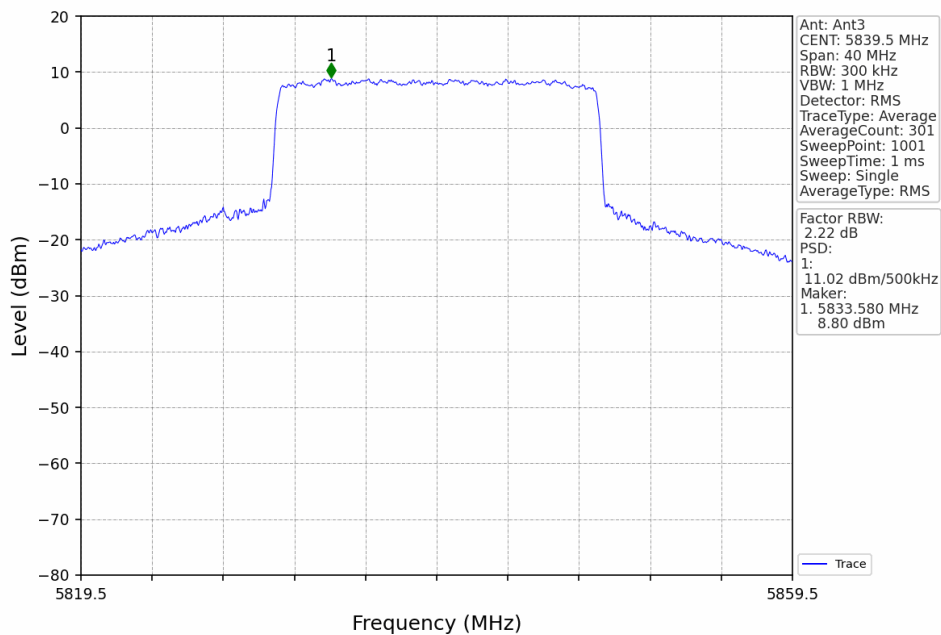
20M_HCH_5839.5MHz_Ant3_NTNV
