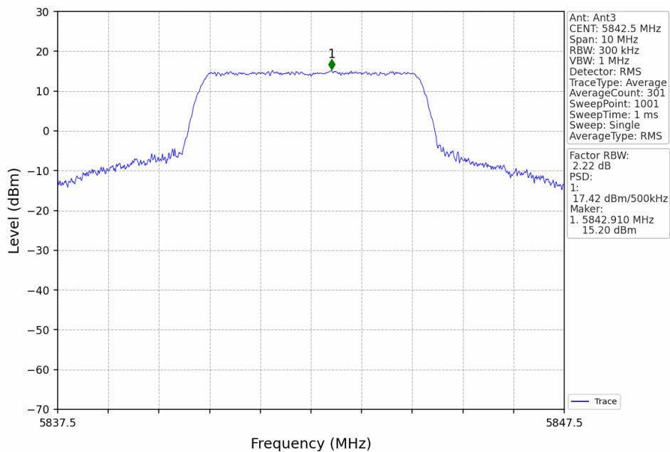
5M_HCH_5842.5MHz_Ant3_NTNV
