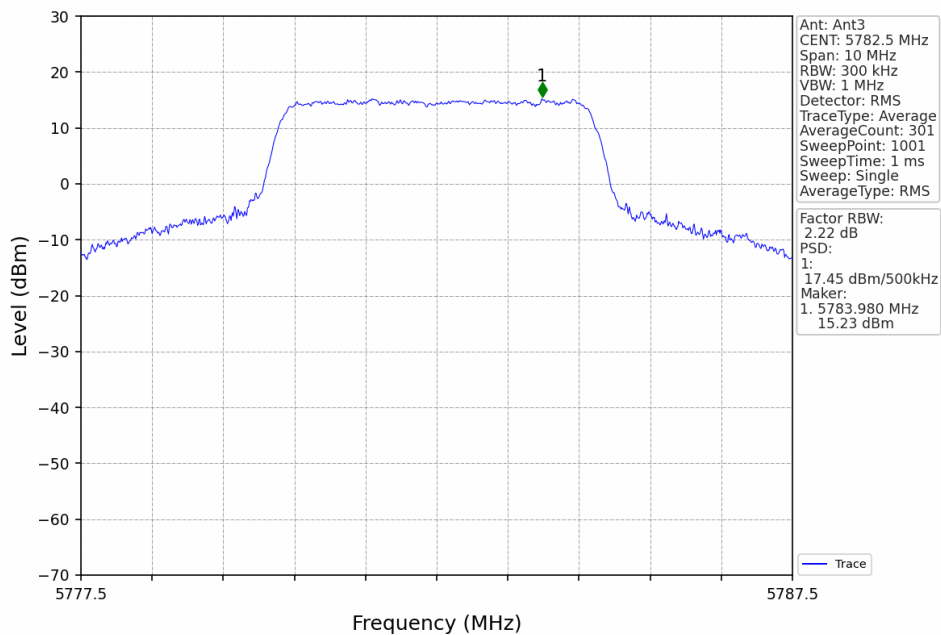
5M_MCH_5782.5MHz_Ant3_NTNV
