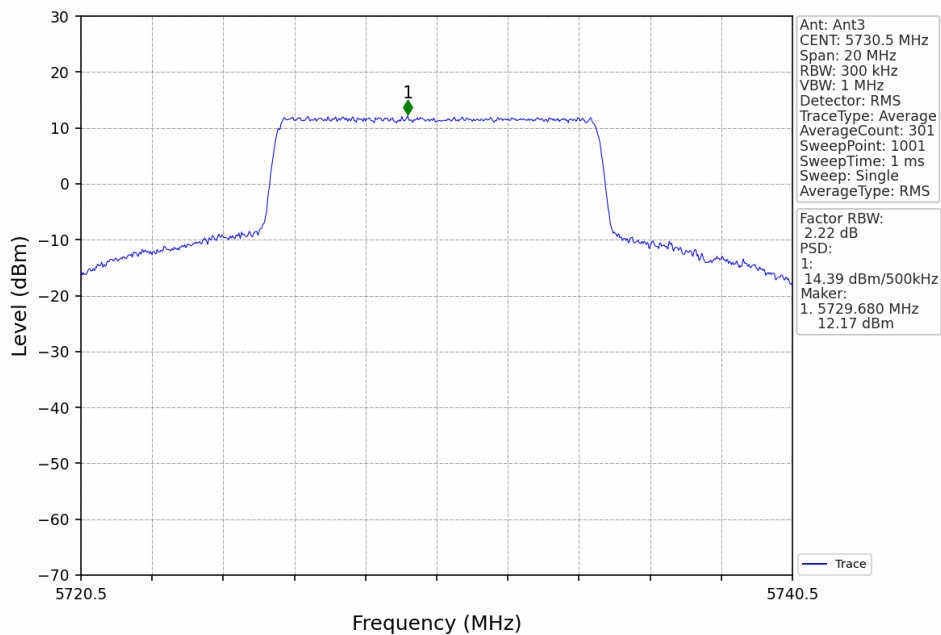
10M_LCH_5730.5MHz_Ant3_NTNV
