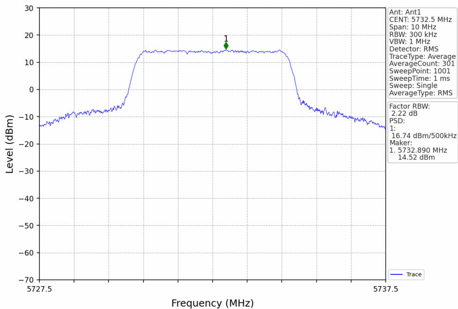
5M_LCH_5732.5MHz_Ant1_NTNV
