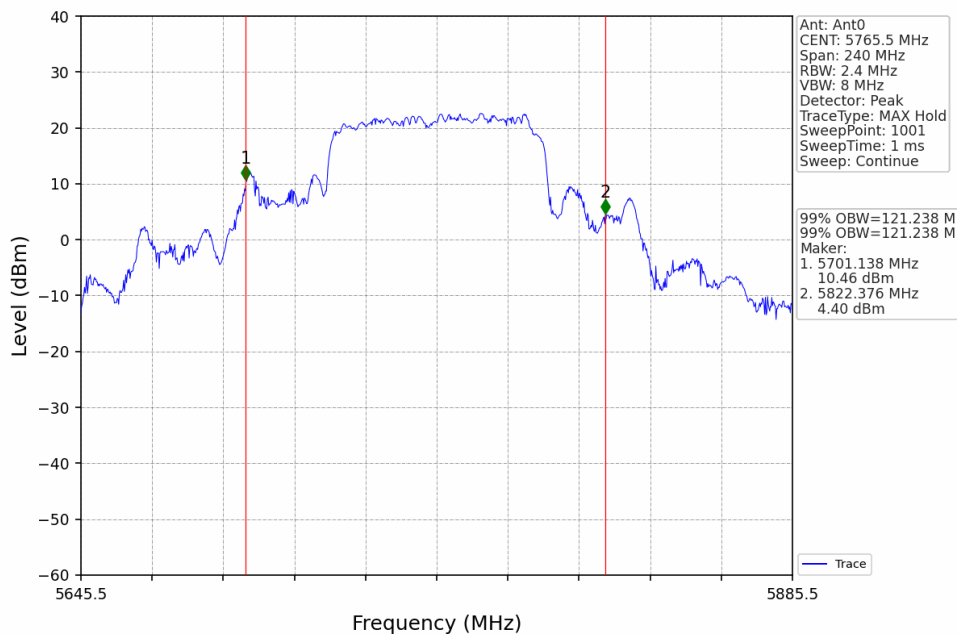
80M_LCH_5765.5MHz_Ant0_NTNV
