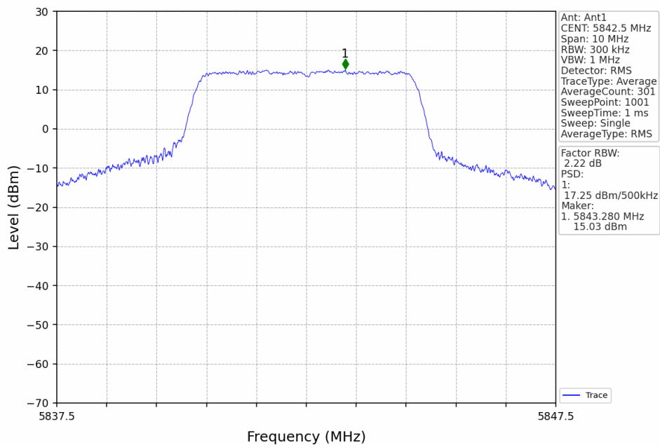
5M_HCH_5842.5MHz_Ant1_NTNV
