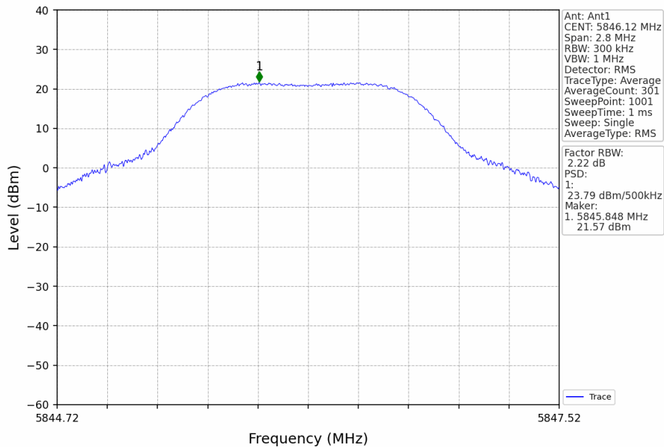
1.4M_HCH_5846.12MHz_Ant1_NTNV
