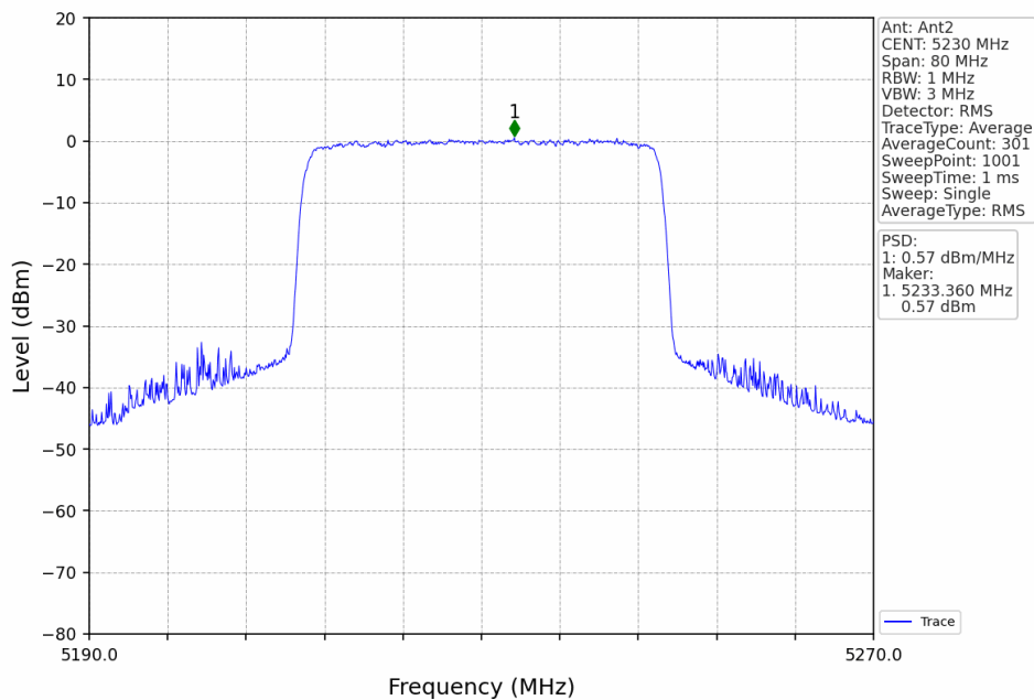
40M_HCH_5230MHz_Ant2_NTNV
