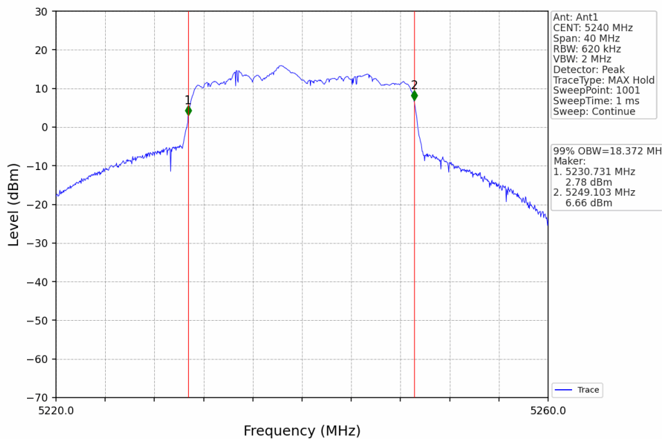
20M_HCH_5240MHz_Ant1_NTNV
