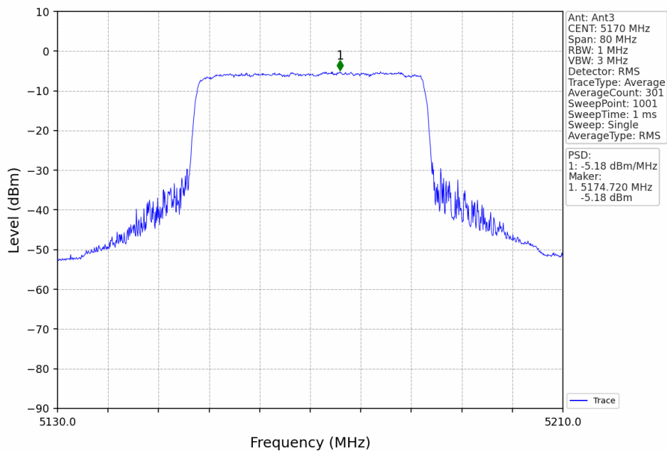
40M_LCH_5170MHz_Ant3_NTNV
