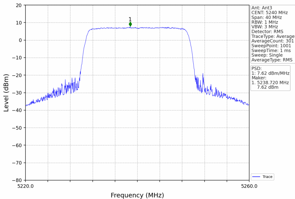
20M_HCH_5240MHz_Ant3_NTNV
