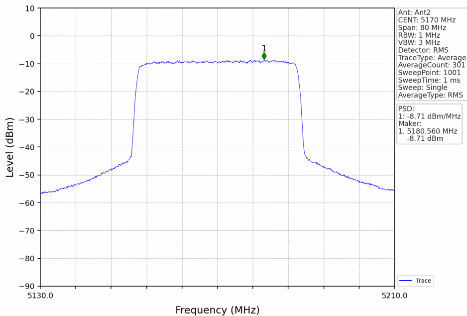
40M_LCH_5170MHz_Ant2_NTNV
