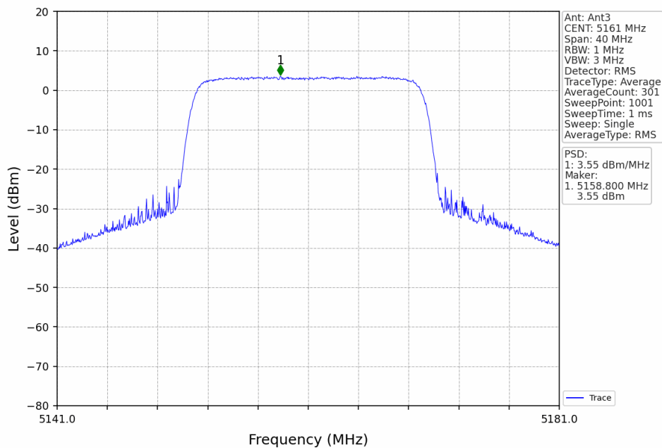
20M_LCH_5161MHz_Ant3_NTNV
