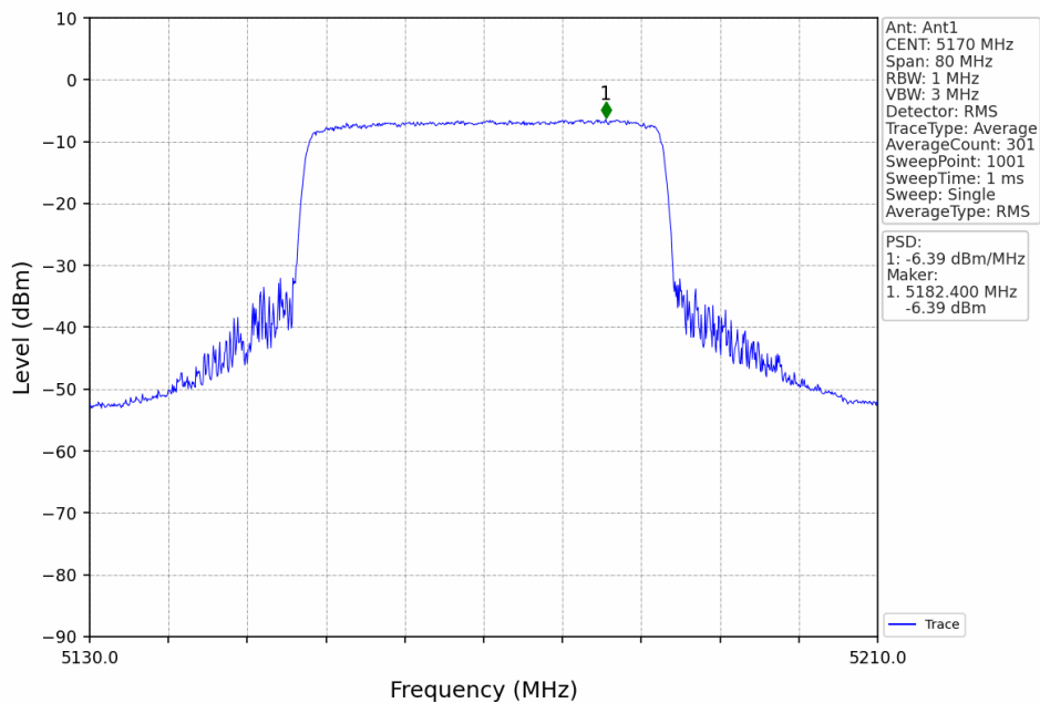
40M_LCH_5170MHz_Ant1_NTNV
