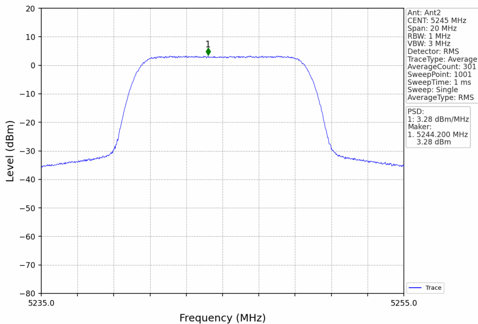
10M_HCH_5245MHz_Ant2_NTNV
