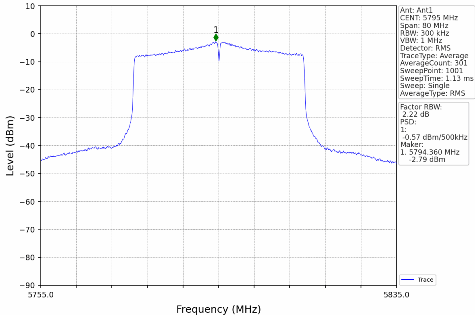
802.11ax(HEW40)_HCH_5795MHz_RU484_Left_MIMO_NTNV
