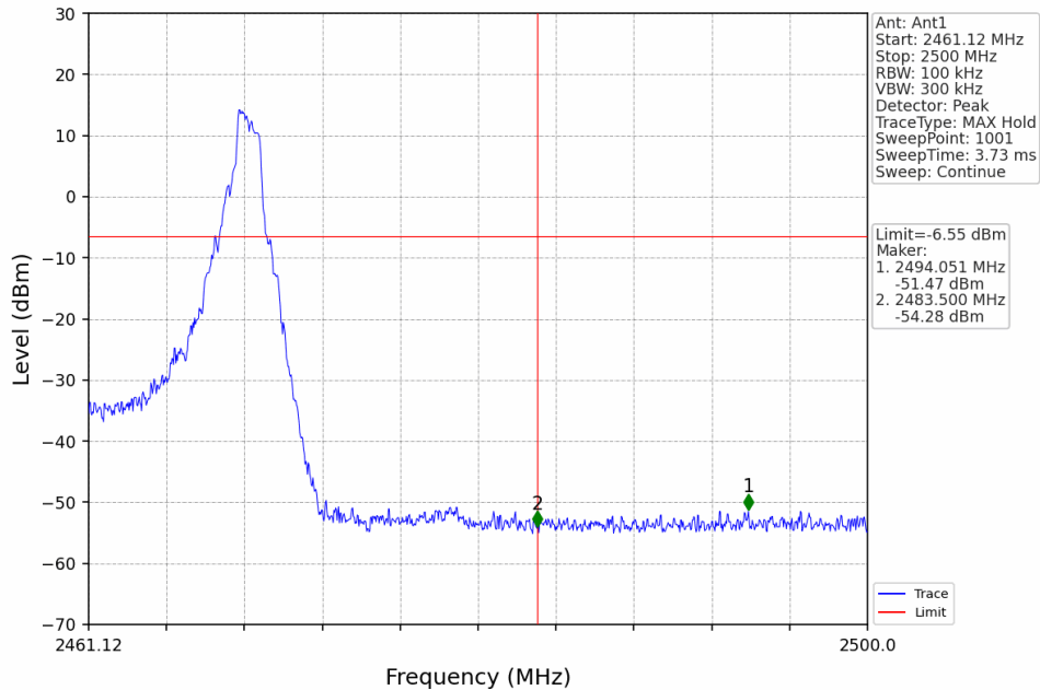
1.4M_HCH_2469.12MHz_Ant1_NTNV
