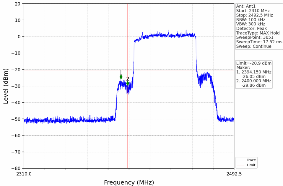
60M_LCH_2432.5MHz_Ant1_NTNV
