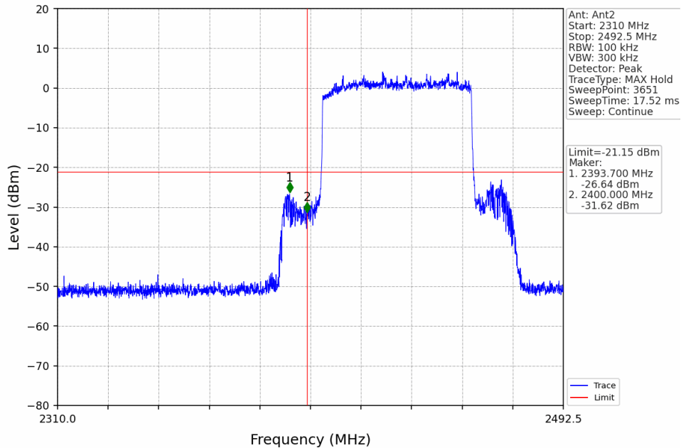
60M_LCH_2432.5MHz_Ant2_NTNV
