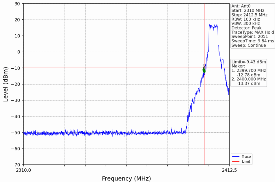
5M_LCH_2404.5MHz_Ant0_NTNV
