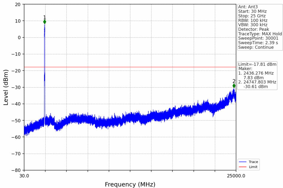
60M_LCH_2432.5MHz_Ant3_NTNV
