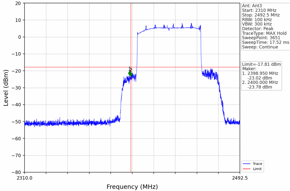
60M_LCH_2432.5MHz_Ant3_NTNV
