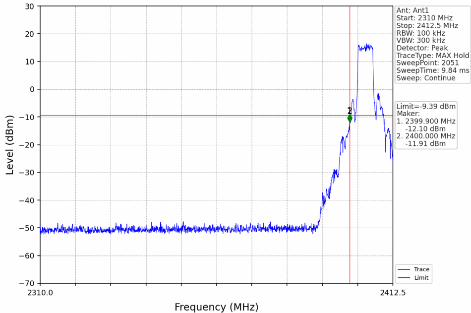
5M_LCH_2404.5MHz_Ant1_NTNV
