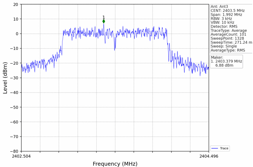
1.4M_LCH_2403.5MHz_Ant3_NTNV
