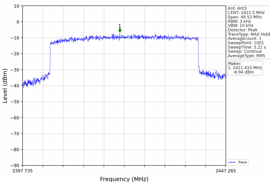
40M_LCH_2422.5MHz_Ant3_NTNV
