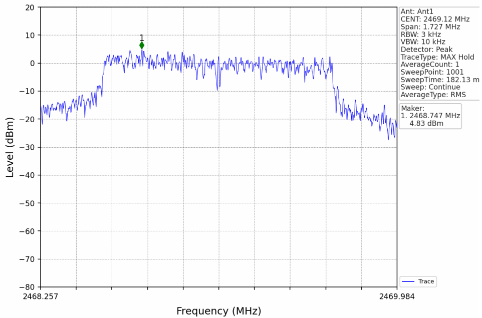
1.4M_HCH_2469.12MHz_Ant1_NTNV
