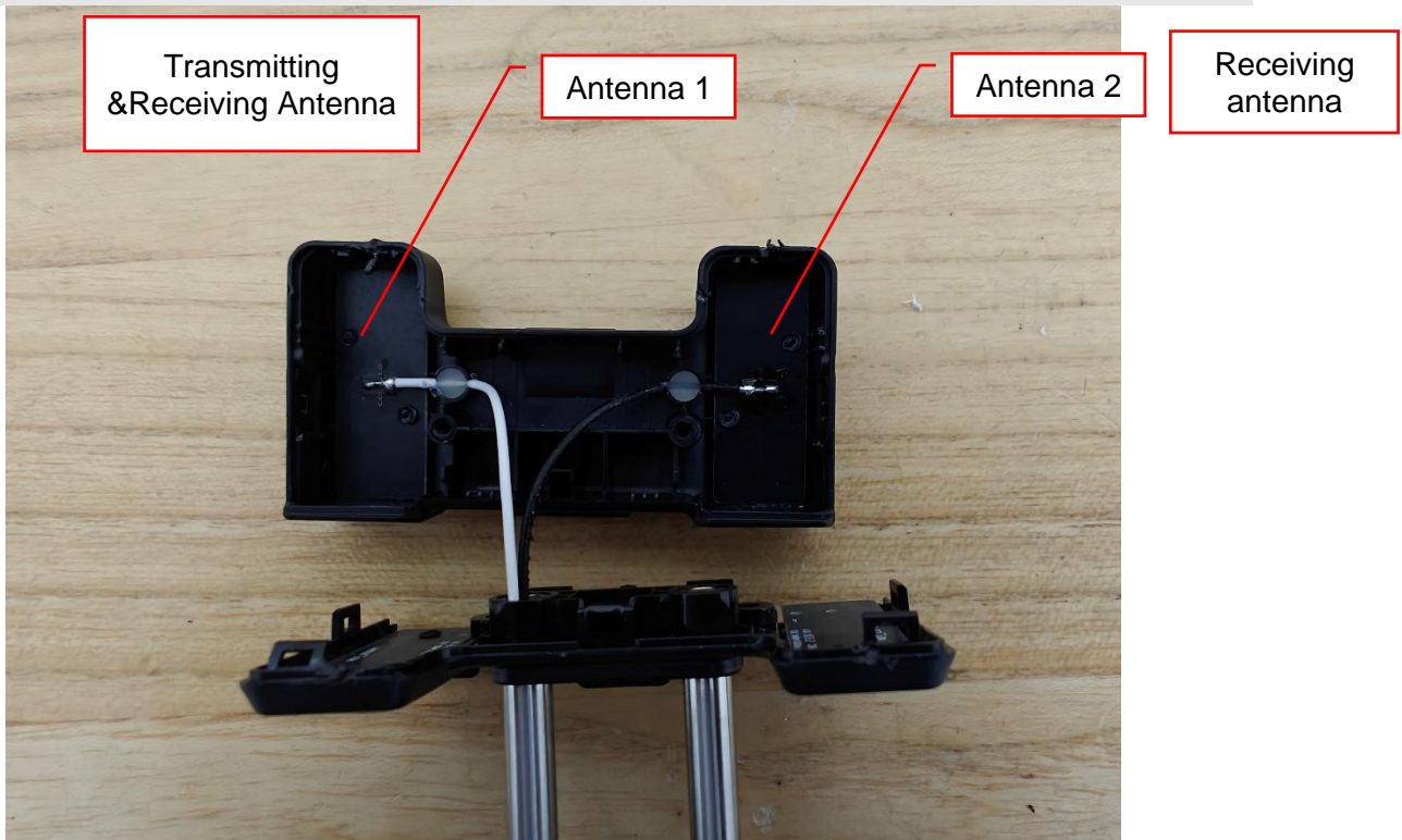
Internal View of EUT-4
