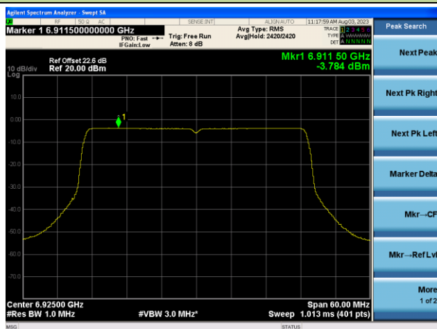
Channel 195 (6925MHz)
