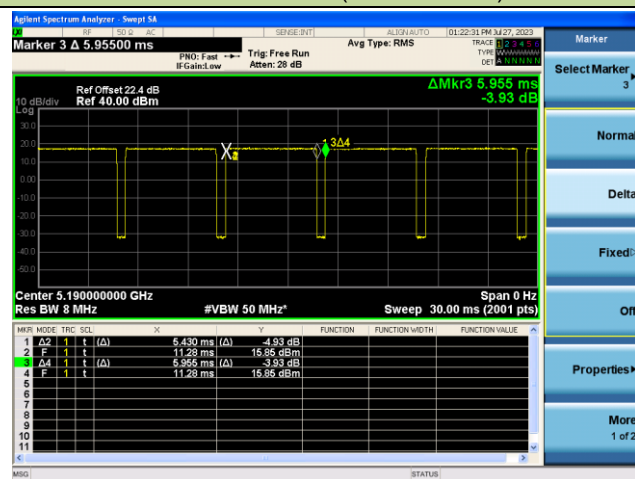
802.11ax-HE40 (T = 5.430ms)
