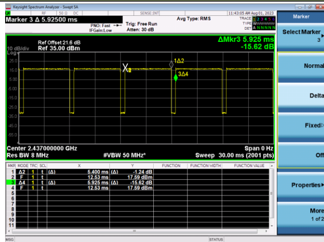
802.11ax-HE20 (T = 5.400ms)
