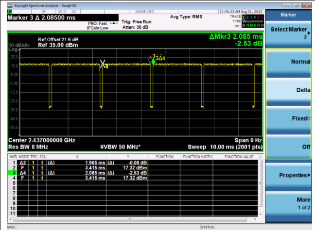
802.11n-HT40 (T = 5.385ms)
