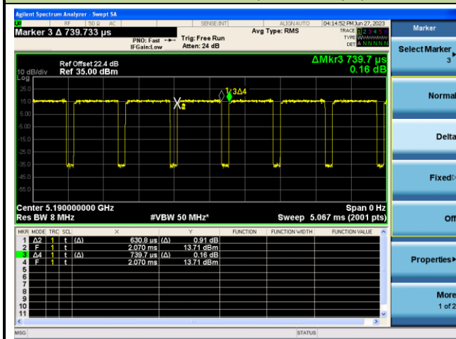
802.11ac-VHT40 (T = 630.8μs)
