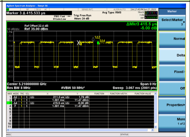
802.11ac-VHT80 (T = 311.3μs)
