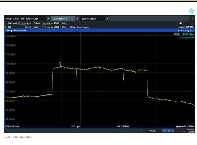
Channel 191 (6905MHz)
