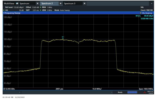
Channel 199 (6945MHz)
