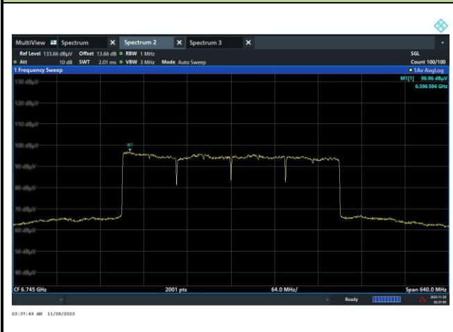
Channel 159 (6745MHz)
