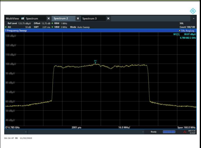
Channel 167 (6785MHz)
