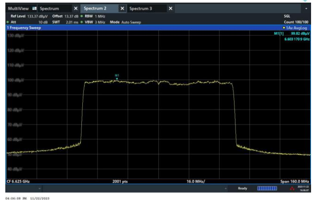
Channel 135 (6625MHz)
