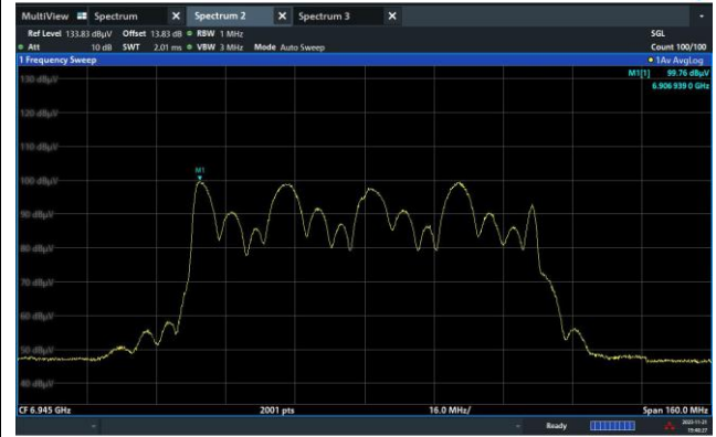
Channel 199 (6945MHz)
