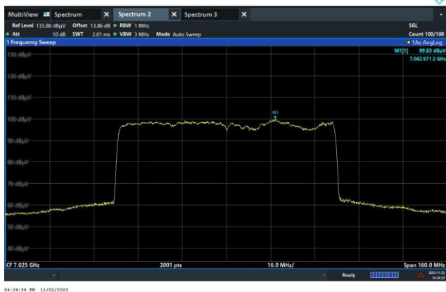
Channel 215 (7025MHz)
