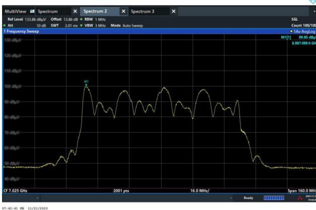
Channel 215 (7025MHz)
