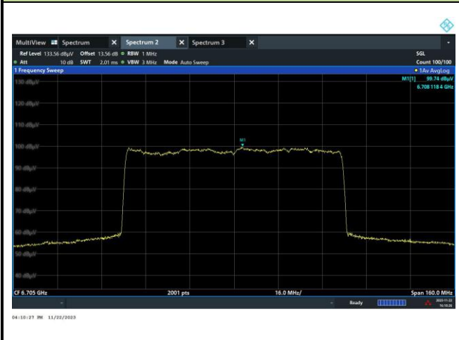
Channel 151 (6705MHz)
