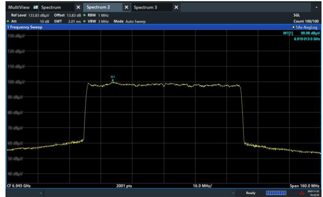
Channel 199 (6945MHz)
