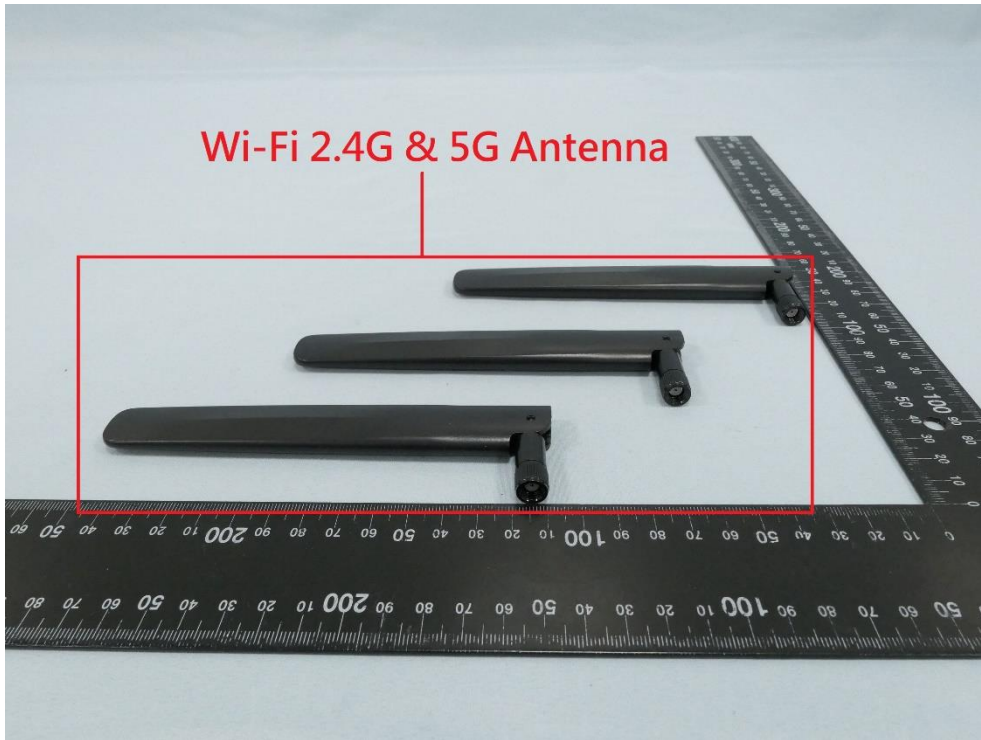
(7) Antenna Photo
