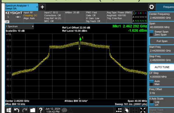
Channel 11 (2462MHz)
