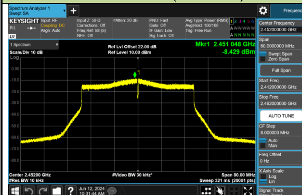
Channel 09 (2452MHz)
