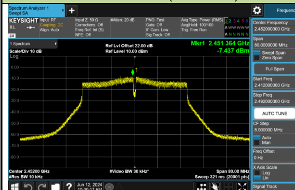
Channel 09 (2452MHz)
