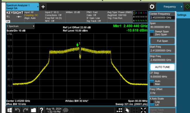
Channel 09 (2452MHz)
