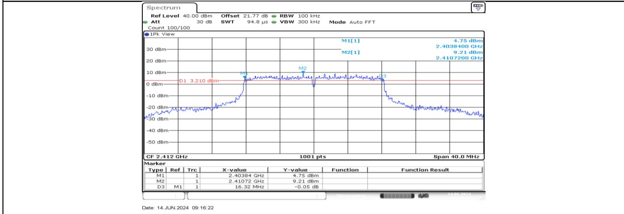
11G-CDD_Ant4_2412
