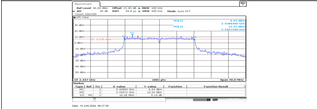
11G-CDD_Ant3_2437
