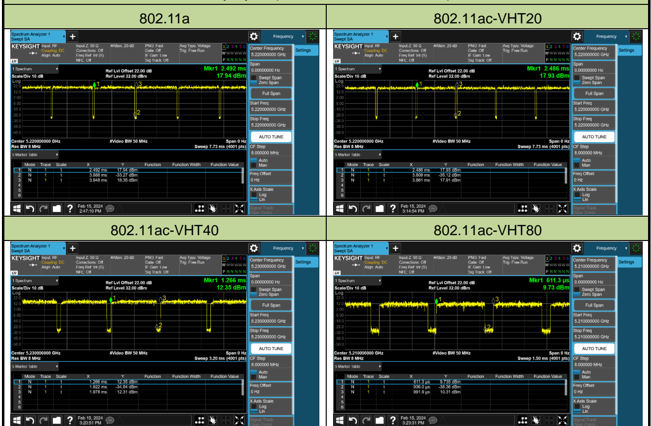
Duty Cycle (T = Transmission Duration)
