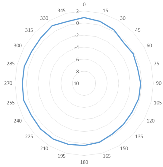
theta90° (XOY) Radiation Pattern at 2.45GHz
