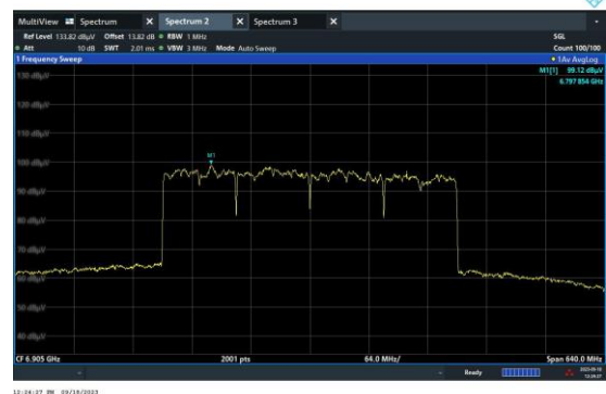
Channel 191 (6905MHz)
