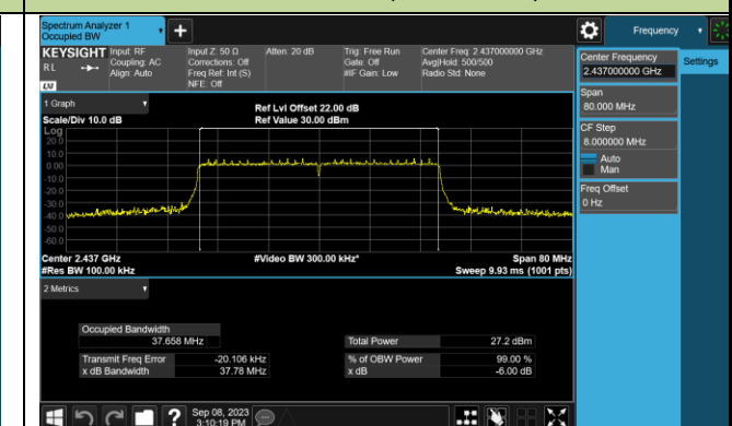
Channel 06 (2437MHz)
