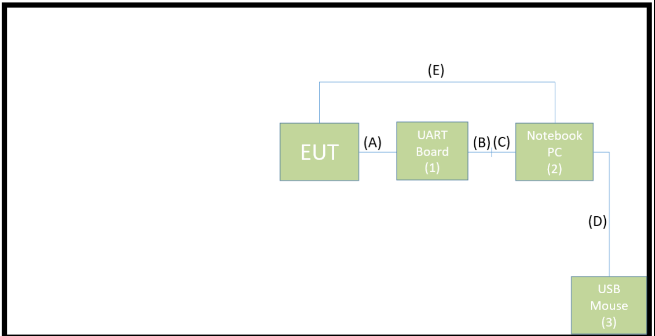
Connection Diagram
