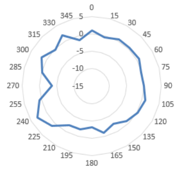
5750MHz-theta90
