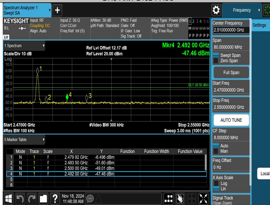
DH5-Ant1-2480-PASS
