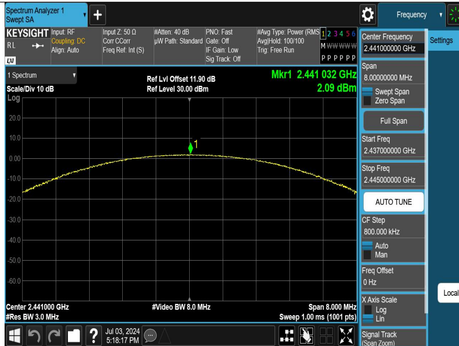
2DH5-Ant1-2441-PASS
