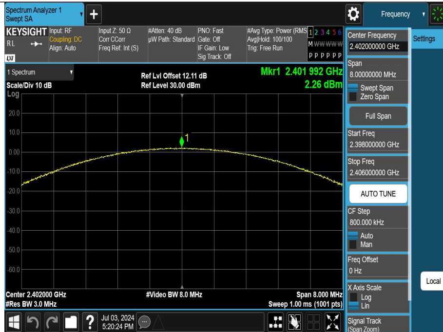
3DH5-Ant1-2402-PASS
