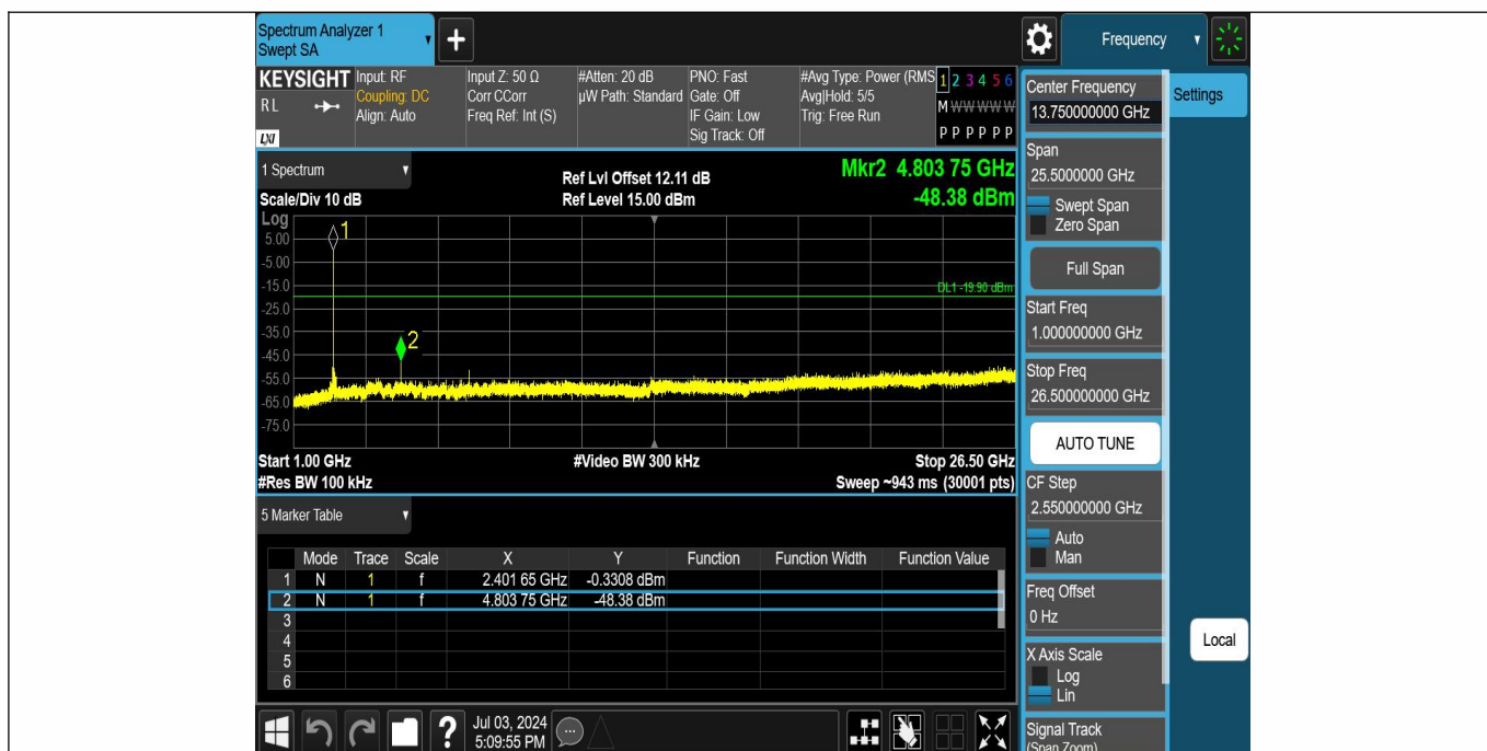
DH5-Ant1-2402-1000~26500-PASS
