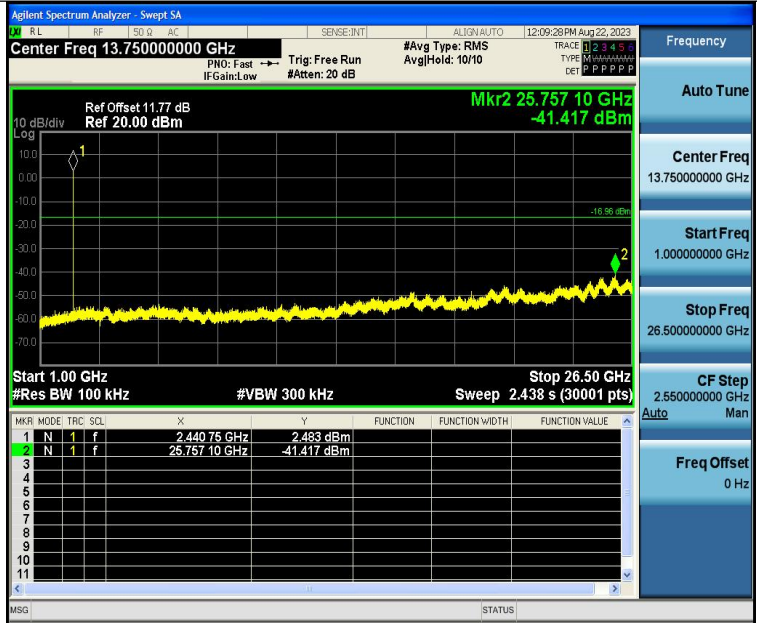
BLE_2M-Ant1-2440-1000~26500-PASS
