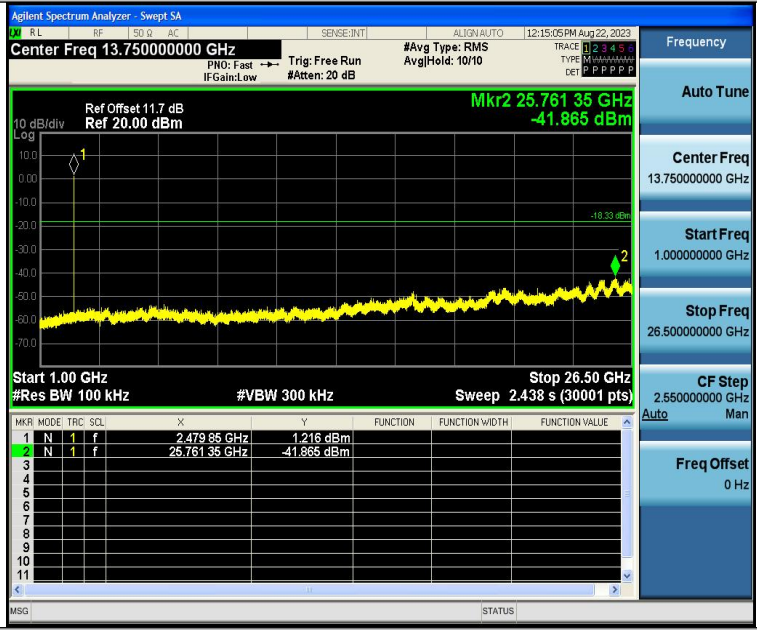
BLE_2M-Ant1-2480-1000~26500-PASS
