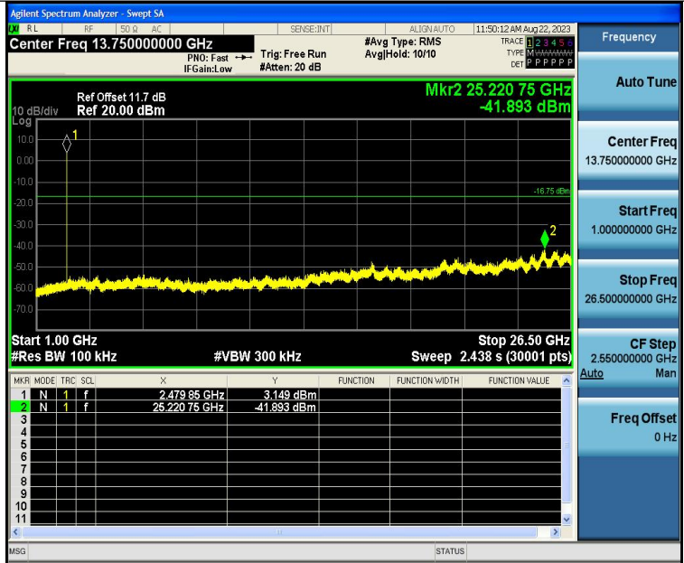
BLE_1M-Ant1-2480-1000~26500-PASS
