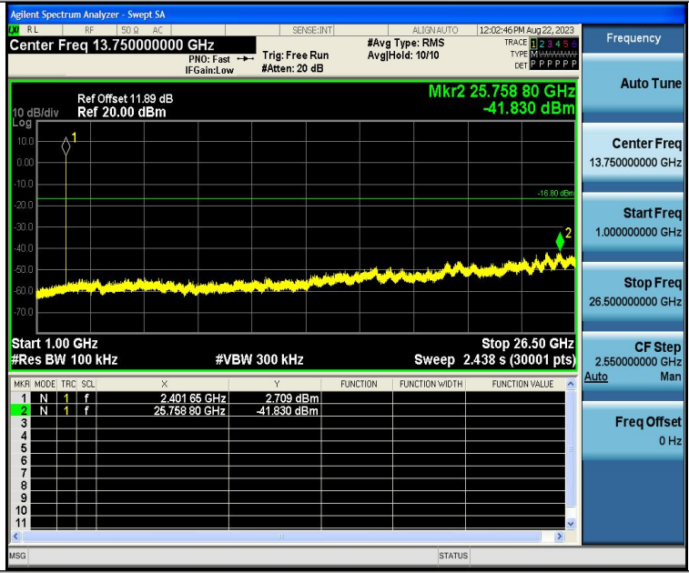
BLE_2M-Ant1-2402-1000~26500-PASS
