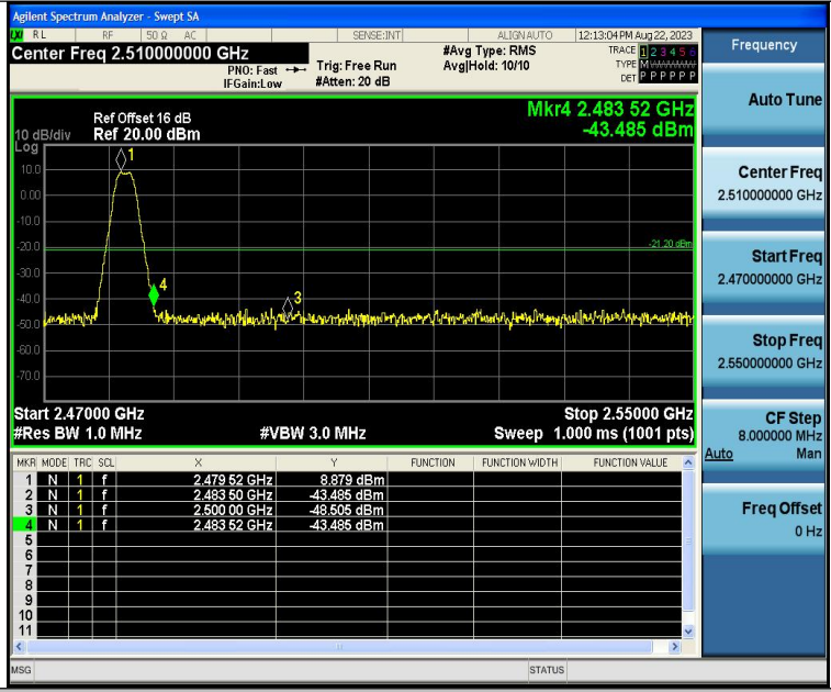
BLE_2M-Ant1-2480-PASS
