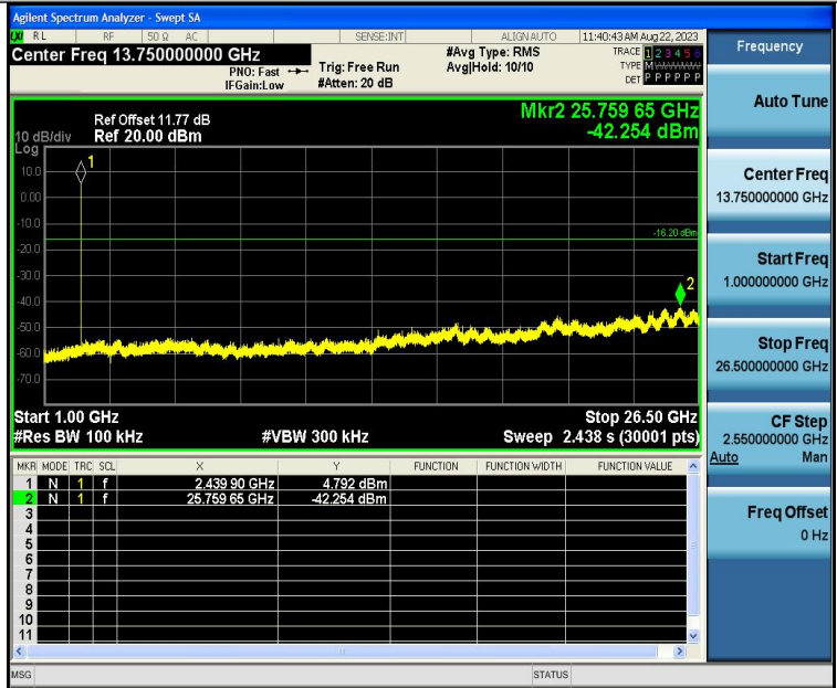
BLE_1M-Ant1-2440-1000~26500-PASS
