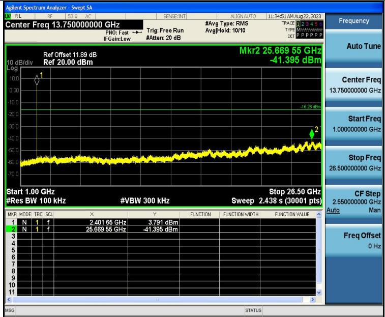
BLE_1M-Ant1-2402-1000~26500-PASS
