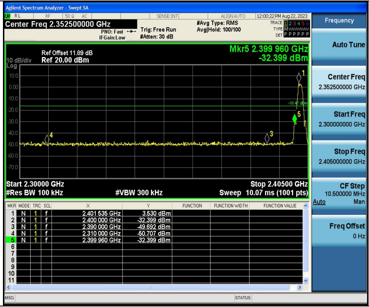
BLE_2M-Ant1-2402-PASS
