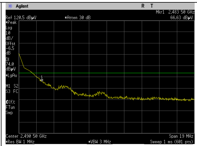
BLE_High Ch_2480MHz_1MBit_15.209_Upper Band Edge Peak_Port 1.gif
