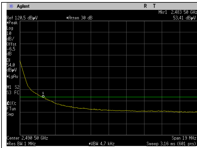
BLE_High Ch_2480MHz_1MBit_15.209_Upper Band Edge Avg_Port 1.gif
