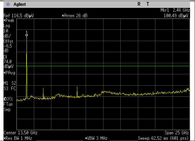
BLE_Mid Ch_2440MHz_1MBit_15.209_1-26GHz peak_Port 1.gif
