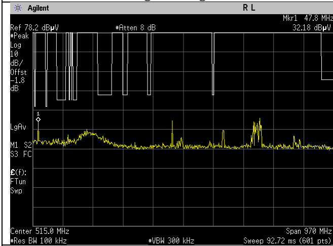
BLE_Mid Ch_2440MHz_1MBit_15.209_30- 1000MHz_Peak_Port 1.gif
