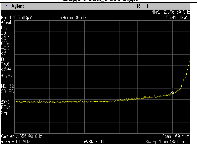
BLE_Low Ch_2402MHz_1MBit_15.209_Lower Band Edge Peak_Port 1.gif
