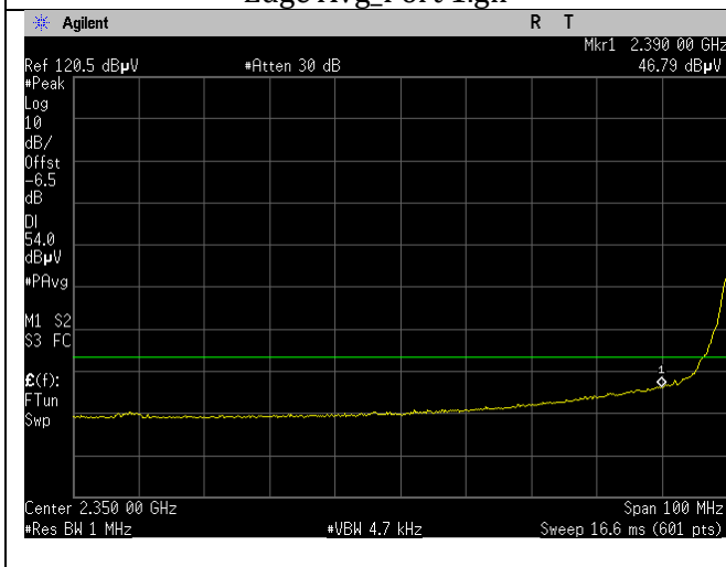
BLE_Low Ch_2402MHz_1MBit_15.209_Lower Band Edge Avg_Port 1.gif
