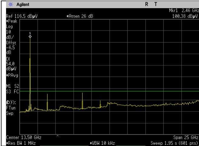
BLE_Mid Ch_2440MHz_1MBit_15.209_1-26GHz avg_Port 1.gif
