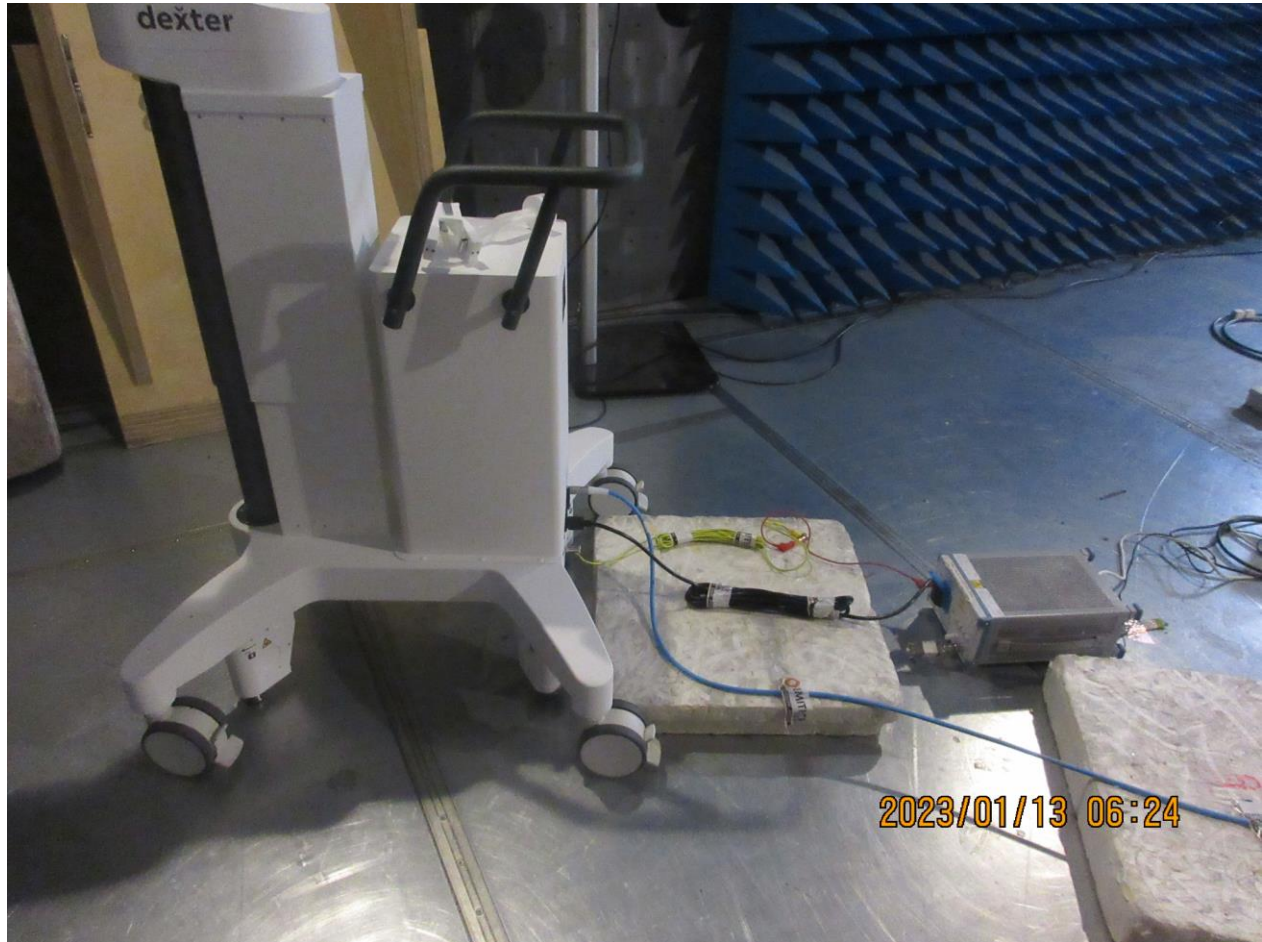
Conducted measurement setup
