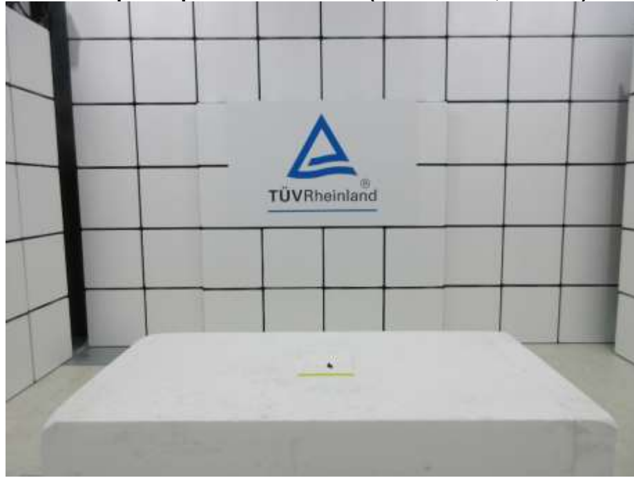
Photograph 2: Test Setup for Spurious Emissions (Front View 2, Left Ear)
