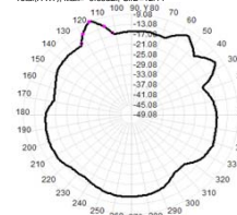
Total(E+YZ), Max=-13.38dB
