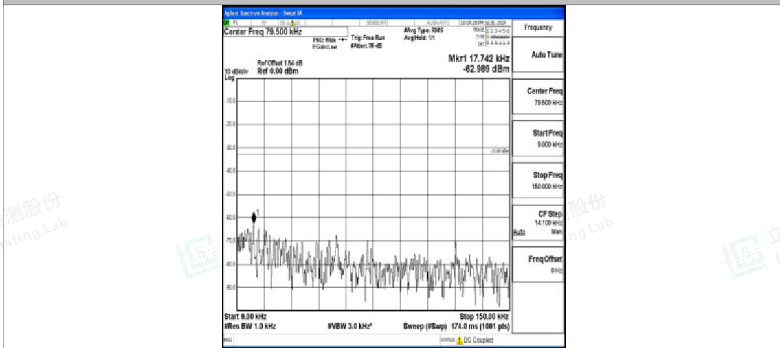
Band5-5MHz-QPSK-20525-1RB#0-0.009~0.15-PASS
