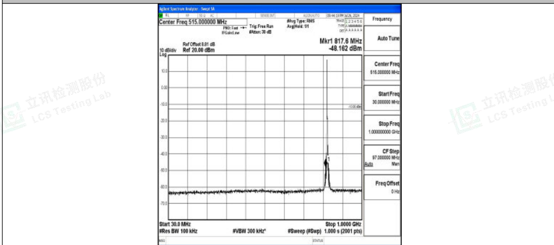
Band5-3MHz-QPSK-20415-1RB#0-30~1000-PASS
