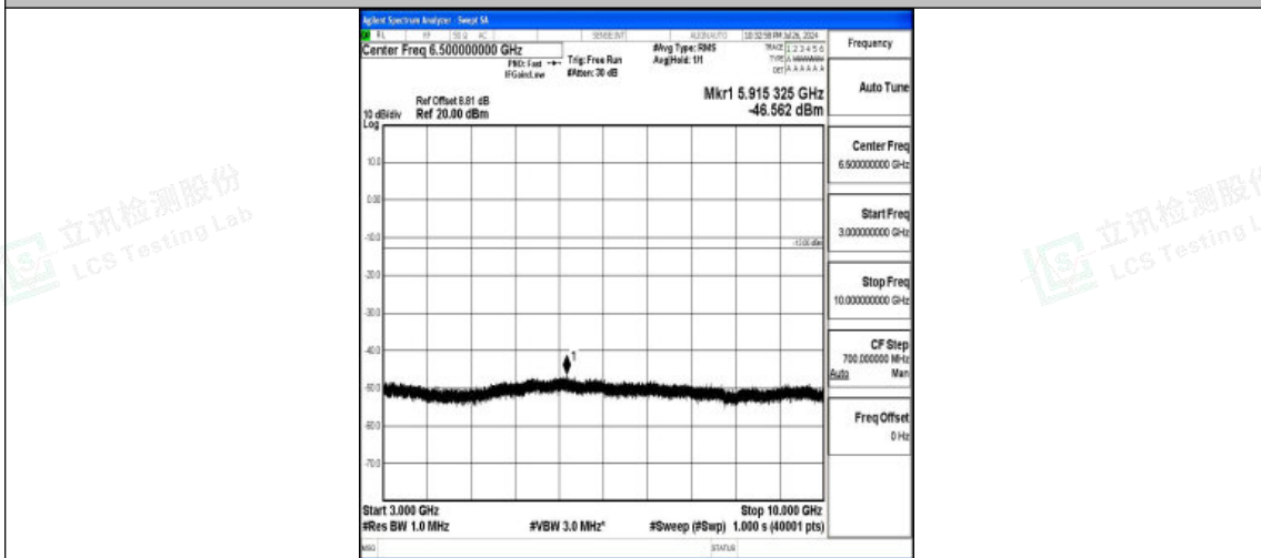
Band5-10MHz-QPSK-20525-1RB#0-3000~10000-PASS
