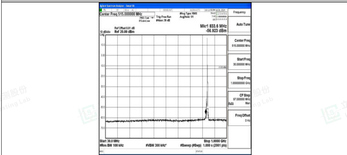
Band5-5MHz-QPSK-20625-1RB#0-30~1000-PASS
