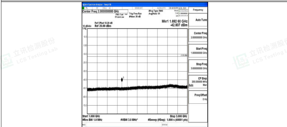
Band5-3MHz-QPSK-20635-1RB#0-1000~3000-PASS
