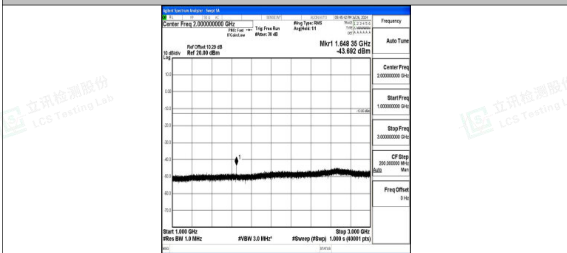
Band5-3MHz-16QAM-20415-1RB#0-1000~3000-PASS
