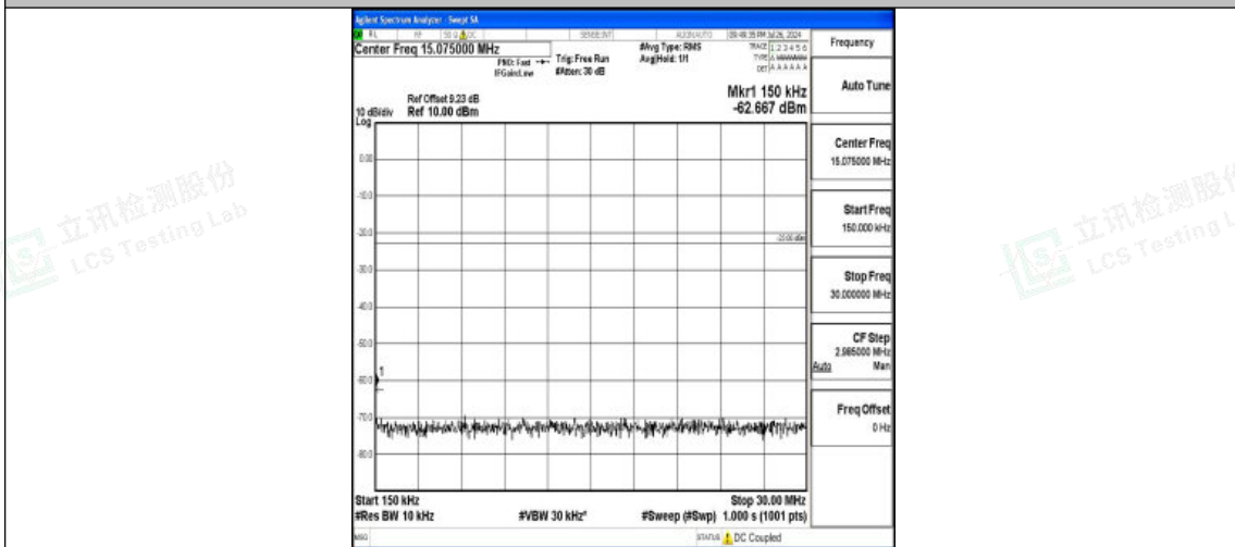
Band5-3MHz-16QAM-20635-1RB#0-0.15~30-PASS
