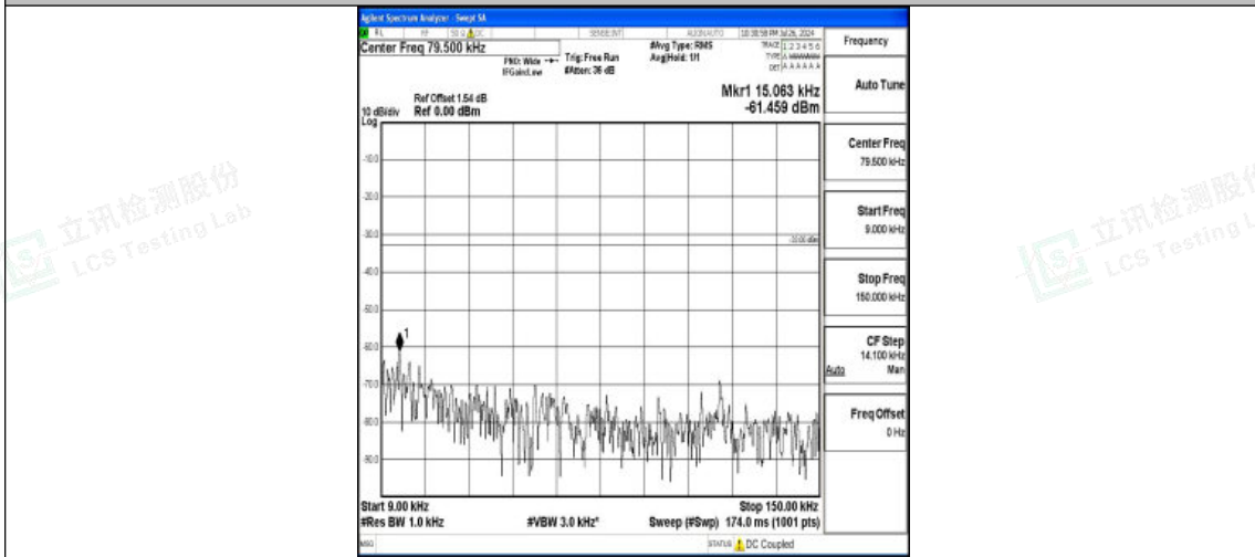
Band5-10MHz-16QAM-20450-1RB#0-0.009~0.15-PASS
