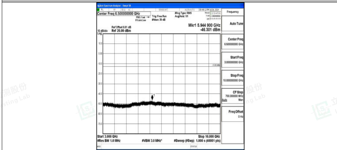
Band5-3MHz-16QAM-20525-1RB#0-3000~10000-PASS
