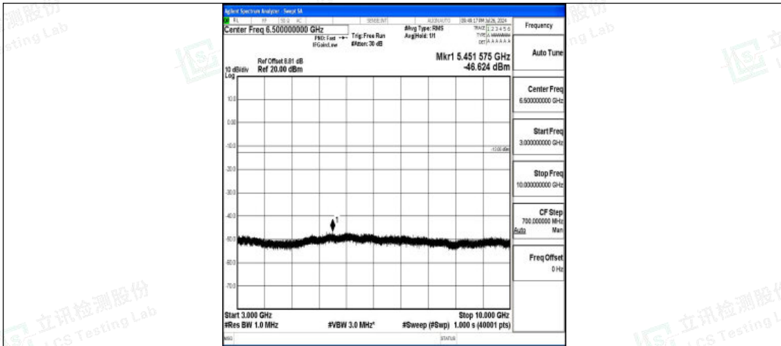
Band5-3MHz-QPSK-20635-1RB#0-3000~10000-PASS
