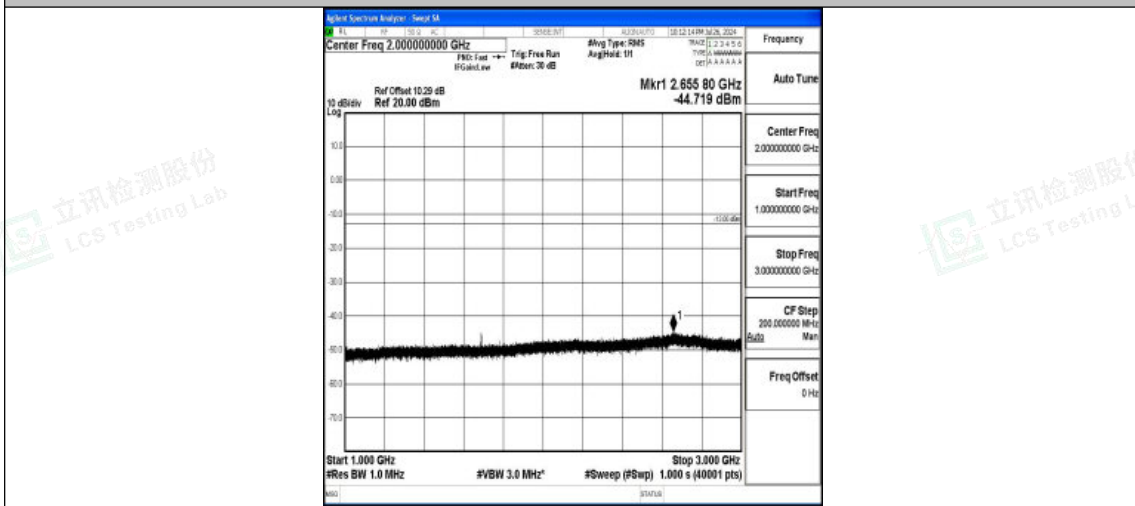
Band5-5MHz-QPSK-20625-1RB#0-1000~3000-PASS
