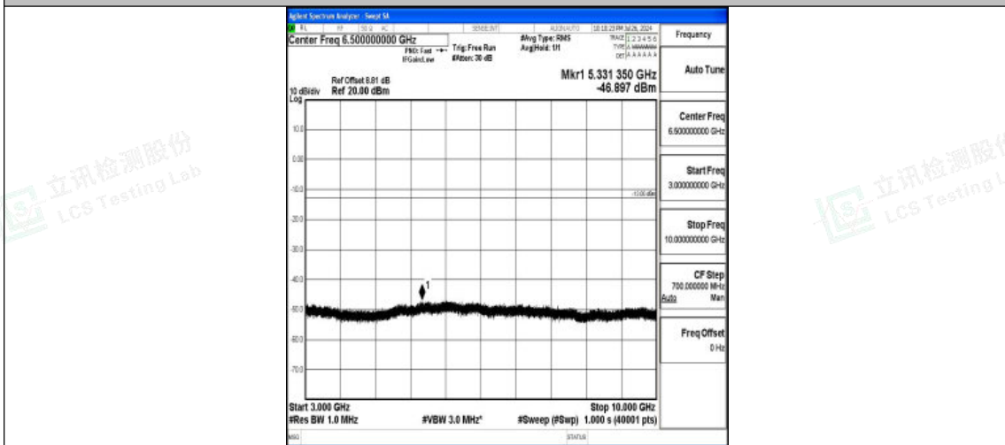
Band5-5MHz-QPSK-20525-1RB#0-3000~10000-PASS
