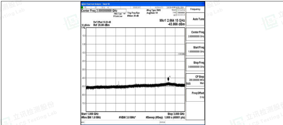
Band5-10MHz-16QAM-20525-1RB#0-1000~3000-PASS
