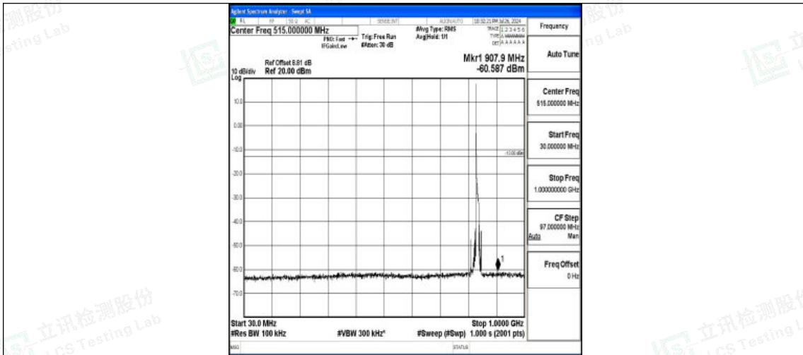
Band5-10MHz-QPSK-20525-1RB#0-30~1000-PASS
