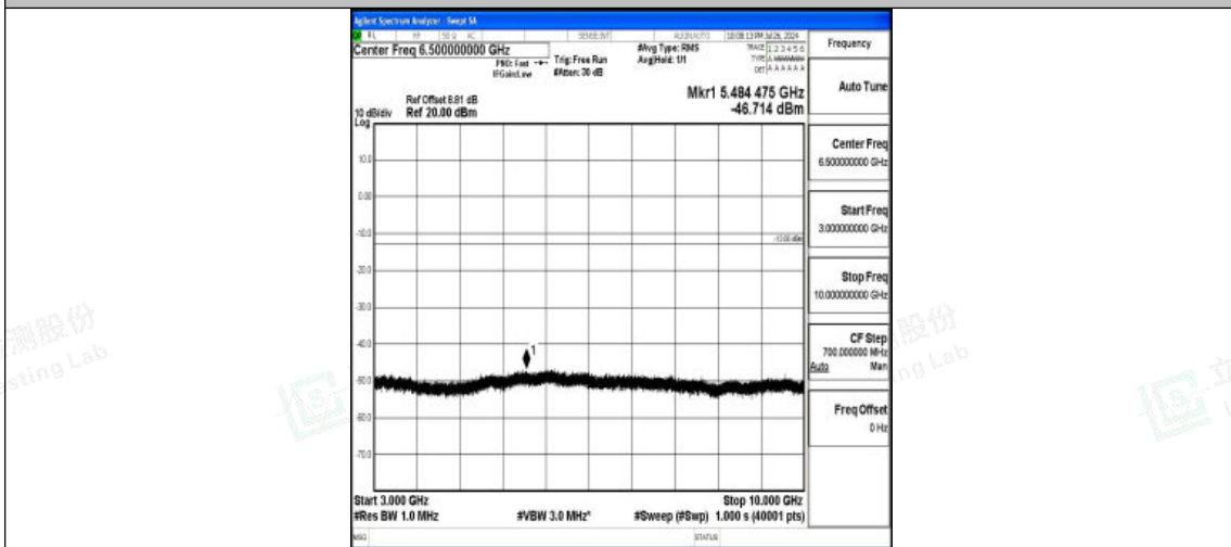
Band5-5MHz-QPSK-20425-1RB#0-3000~10000-PASS
