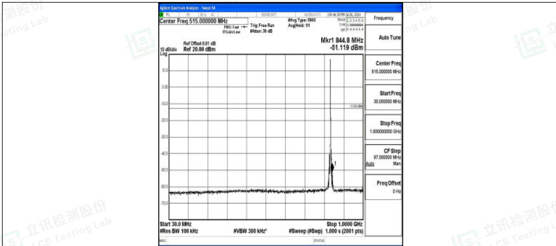
Band5-3MHz-QPSK-20525-1RB#0-30~1000-PASS
