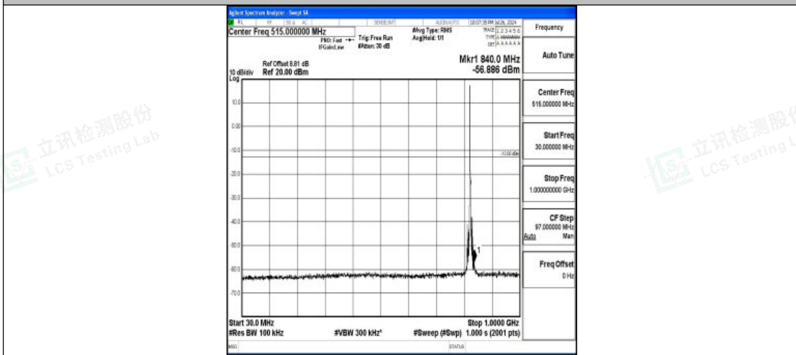
Band5-5MHz-QPSK-20425-1RB#0-30~1000-PASS
