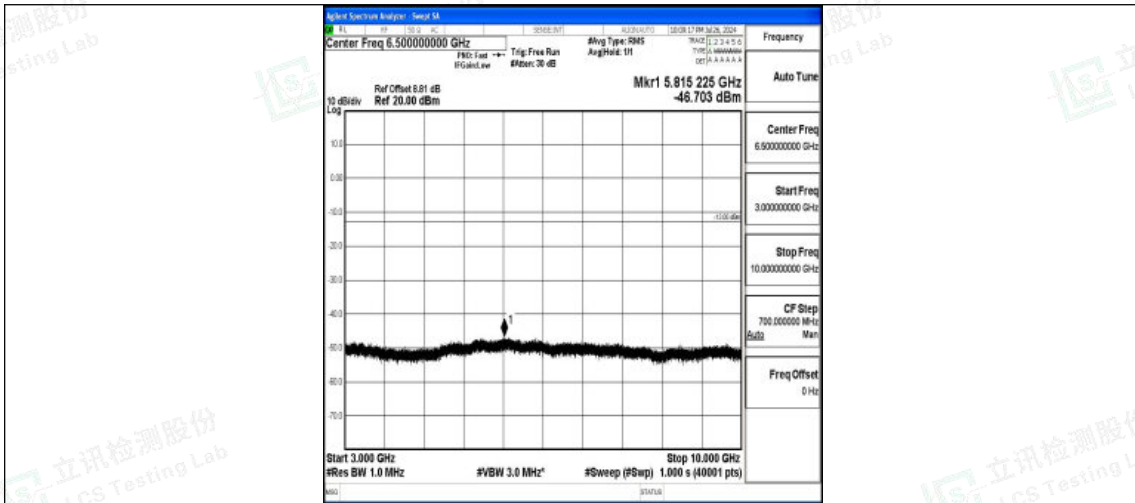
Band5-5MHz-16QAM-20425-1RB#0-3000~10000-PASS
