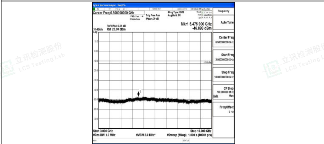
Band5-3MHz-16QAM-20635-1RB#0-3000~10000-PASS
