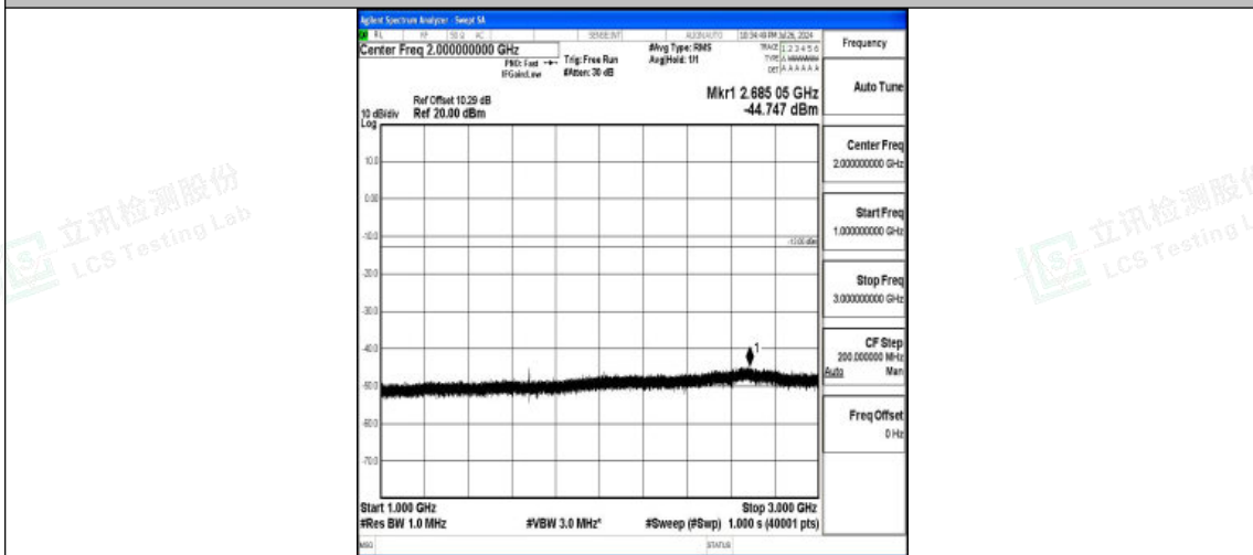
Band5-10MHz-QPSK-20600-1RB#0-1000~3000-PASS
