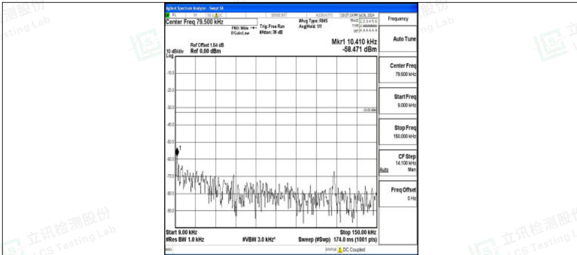
Band5-5MHz-QPSK-20425-1RB#0-0.009~0.15-PASS
