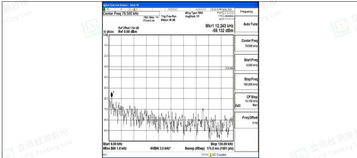
Band5-5MHz-16QAM-20525-1RB#0-0.009~0.15-PASS
