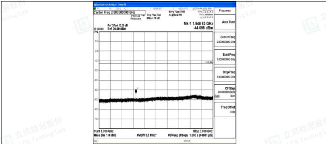
Band5-5MHz-QPSK-20425-1RB#0-1000~3000-PASS
