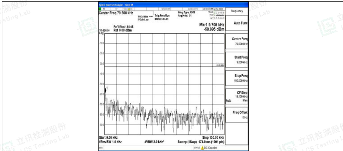
Band5-10MHz-16QAM-20525-1RB#0-0.009~0.15-PASS
