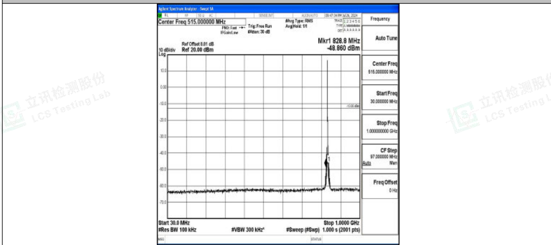
Band5-3MHz-16QAM-20525-1RB#0-30~1000-PASS
