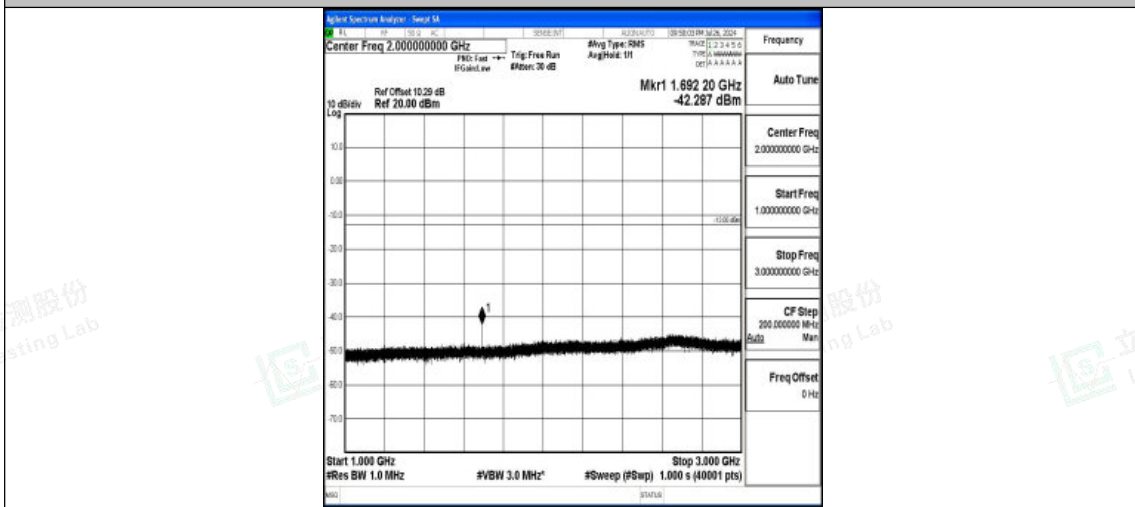
Band5-3MHz-16QAM-20635-1RB#0-1000~3000-PASS
