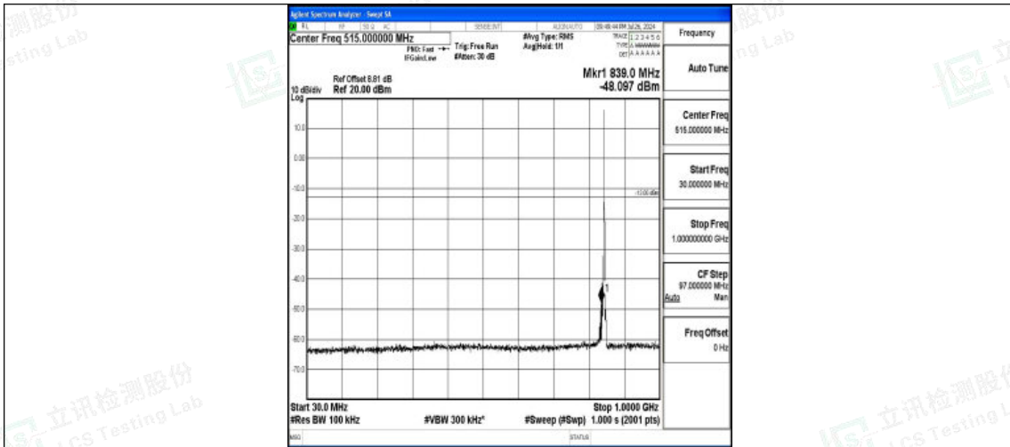
Band5-3MHz-16QAM-20635-1RB#0-30~1000-PASS
