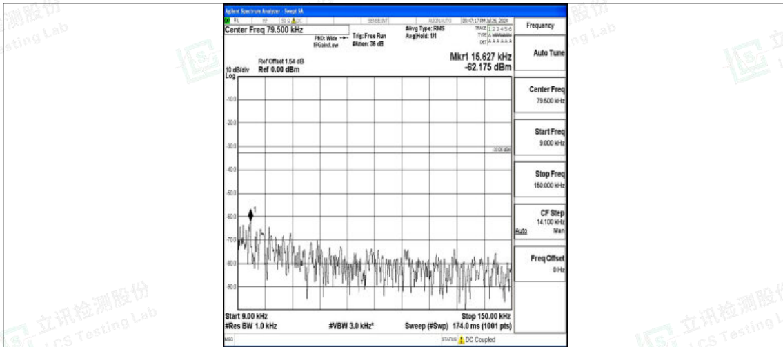
Band5-3MHz-16QAM-20525-1RB#0-0.009~0.15-PASS
