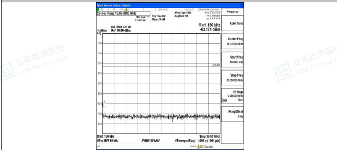
Band5-5MHz-QPSK-20525-1RB#0-0.15~30-PASS
