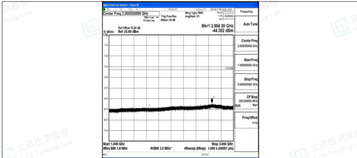
Band5-3MHz-QPSK-20415-1RB#0-1000~3000-PASS
