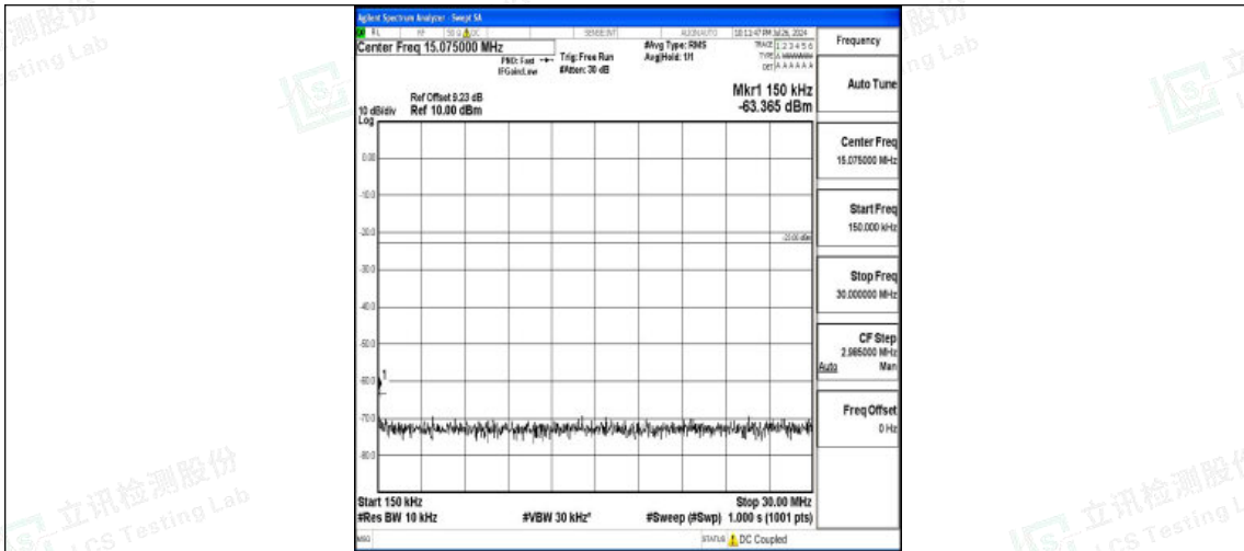
Band5-5MHz-QPSK-20625-1RB#0-0.15~30-PASS
