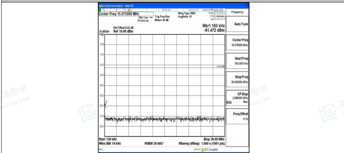
Band5-5MHz-QPSK-20425-1RB#0-0.15~30-PASS
