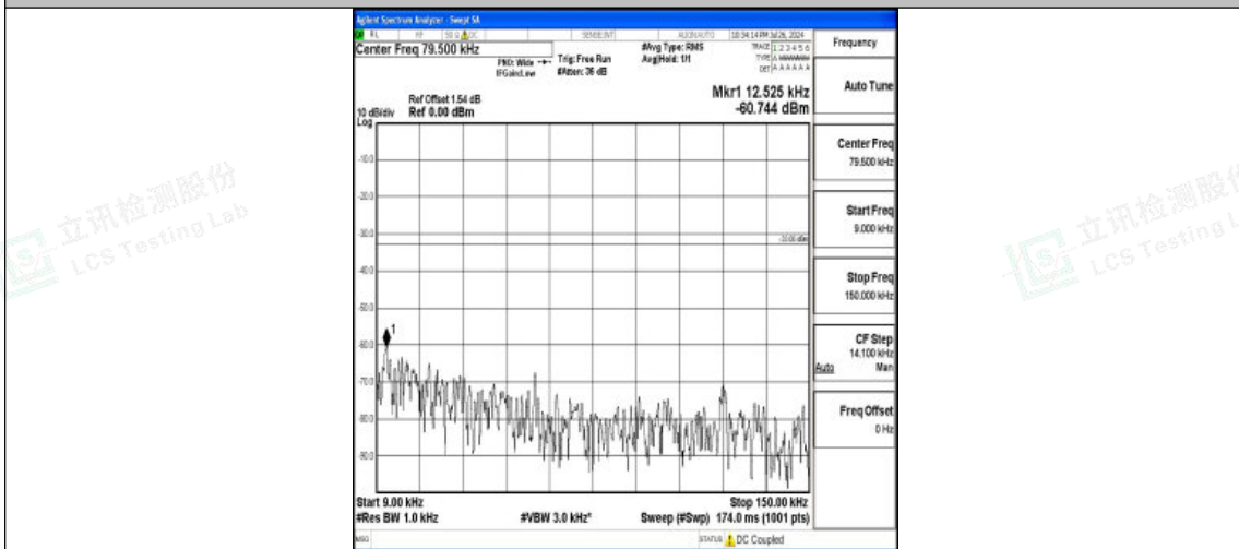
Band5-10MHz-QPSK-20600-1RB#0-0.009~0.15-PASS
