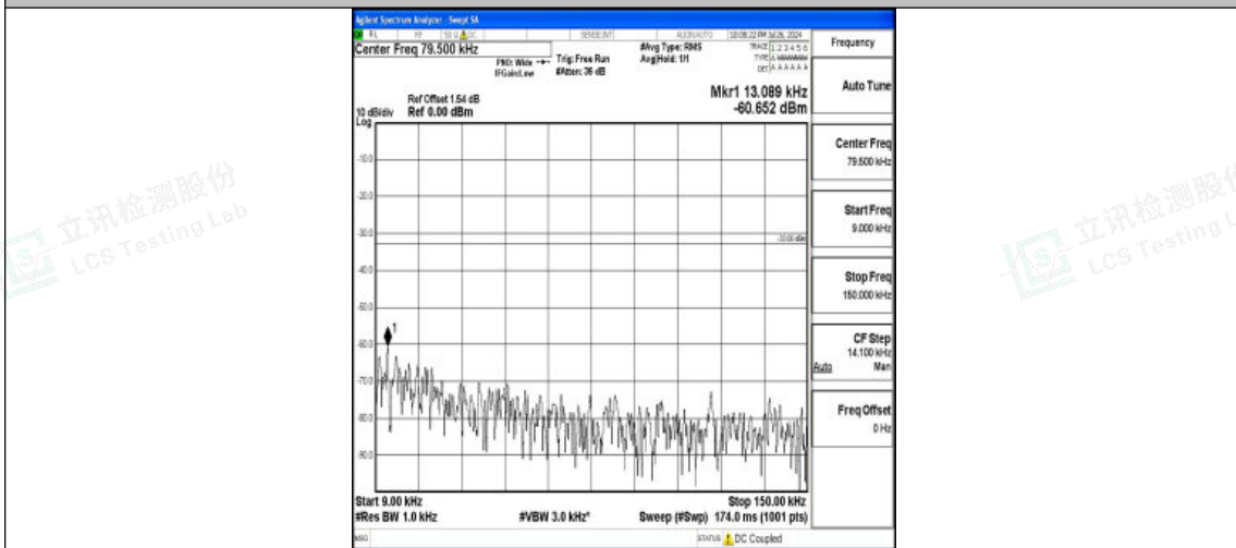
Band5-5MHz-16QAM-20425-1RB#0-0.009~0.15-PASS
