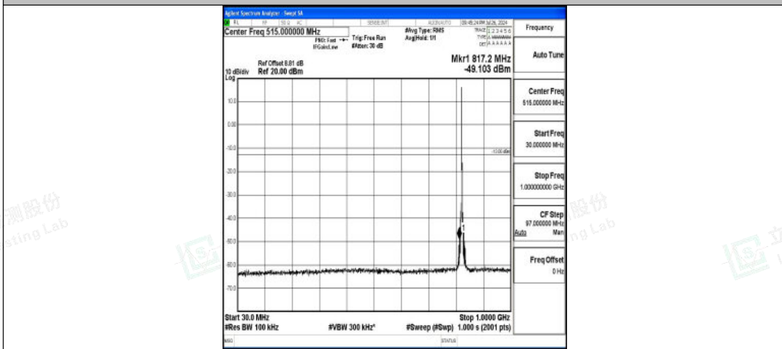
Band5-3MHz-16QAM-20415-1RB#0-30~1000-PASS
