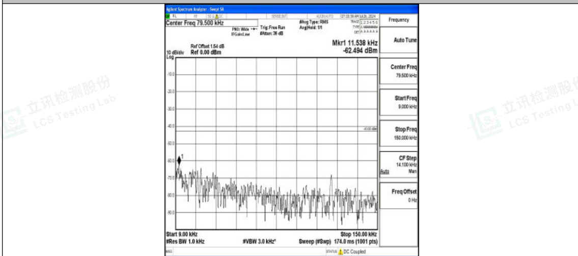
Band4-20MHz-16QAM-20050-1RB#0-0.009~0.15-PASS
