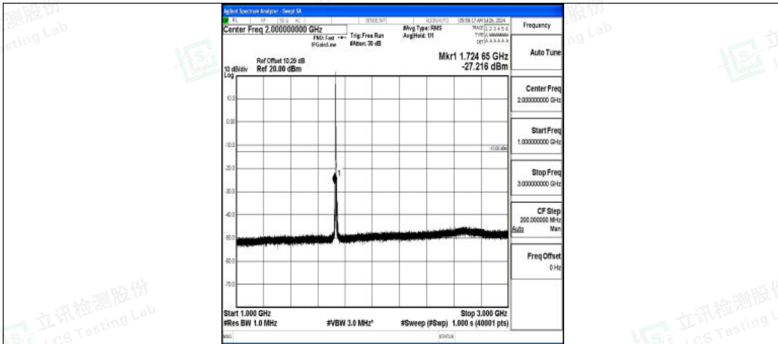
Band4-3MHz-16QAM-20175-1RB#0-1000~3000-PASS
