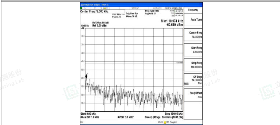
Band4-3MHz-16QAM-20385-1RB#0-0.009~0.15-PASS
