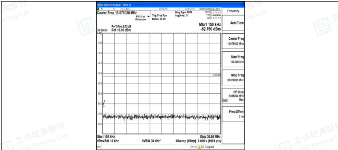
Band4-5MHz-16QAM-19975-1RB#0-0.15~30-PASS
