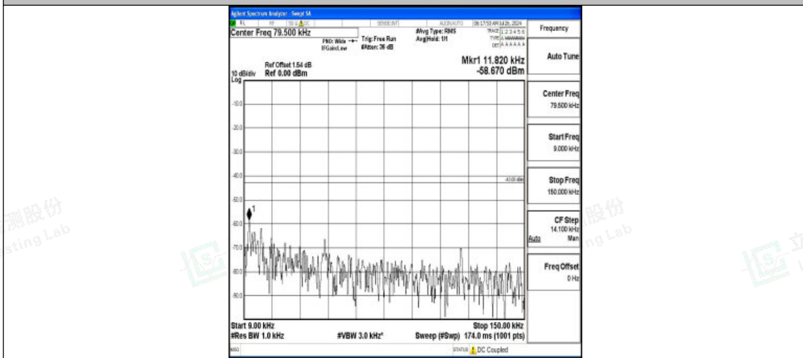
Band4-5MHz-QPSK-20175-1RB#0-0.009~0.15-PASS
