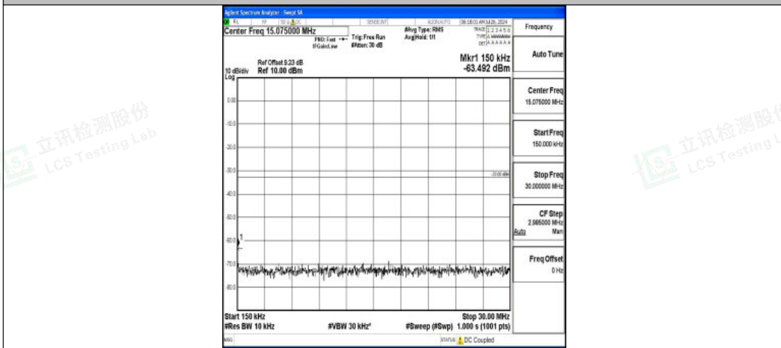
Band4-5MHz-QPSK-20175-1RB#0-0.15~30-PASS
