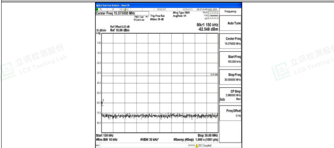
Band4-10MHz-QPSK-20175-1RB#0-0.15~30-PASS
