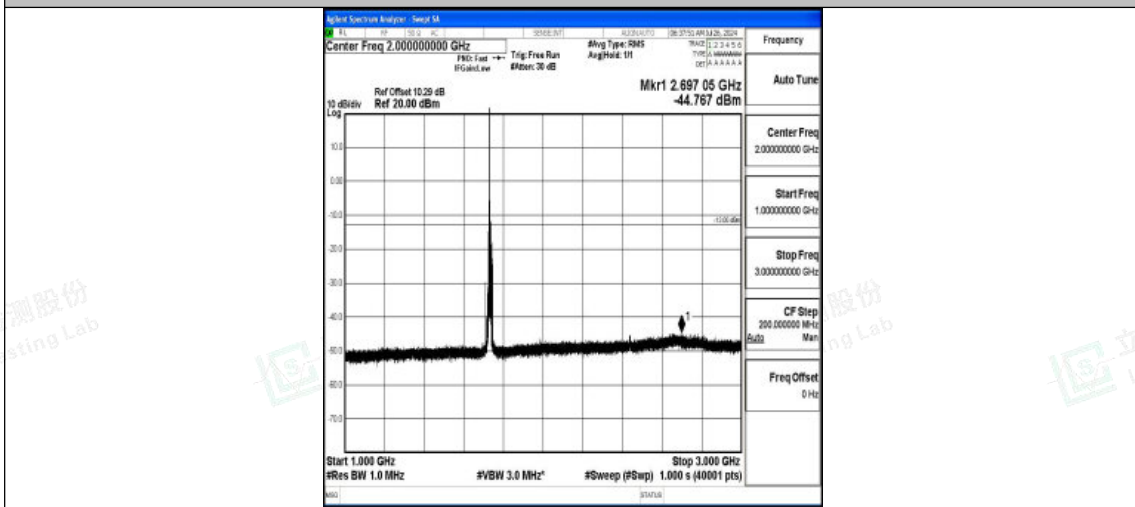
Band4-10MHz-QPSK-20175-1RB#0-1000~3000-PASS
