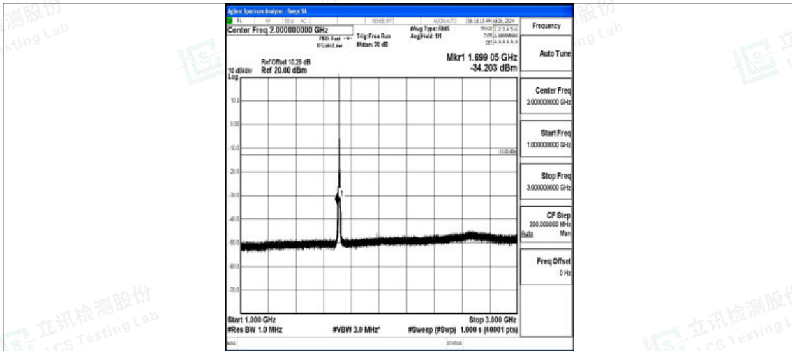
Band4-5MHz-QPSK-19975-1RB#0-1000~3000-PASS
