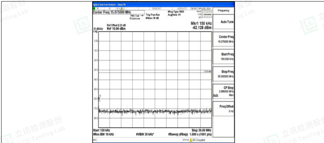
Band4-10MHz-16QAM-20000-1RB#0-0.15~30-PASS
