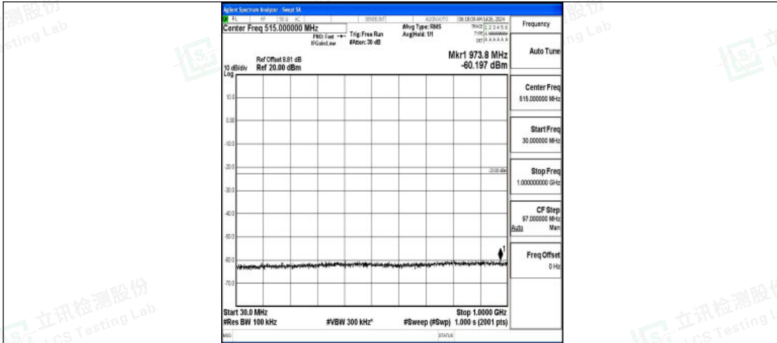
Band4-5MHz-QPSK-20175-1RB#0-30~1000-PASS
