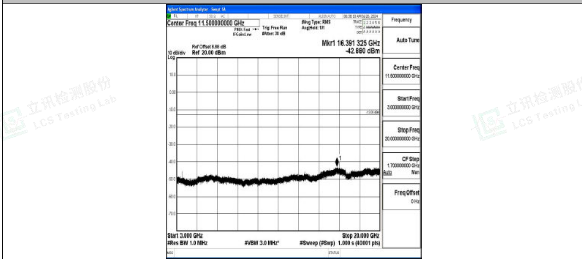
Band4-10MHz-QPSK-20175-1RB#0-3000~20000-PASS
