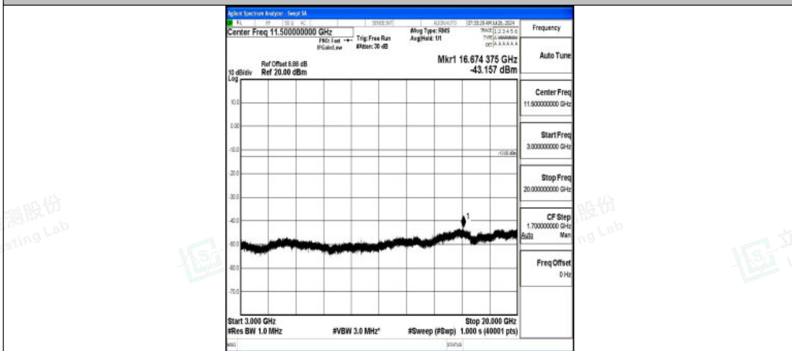
Band4-20MHz-QPSK-20050-1RB#0-3000~20000-PASS
