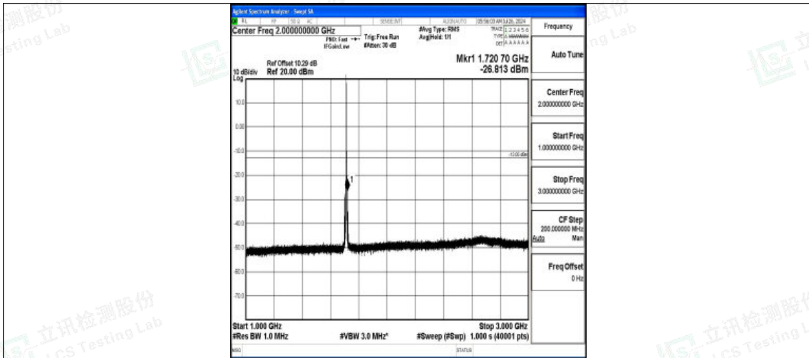
Band4-3MHz-QPSK-19965-1RB#0-1000~3000-PASS
