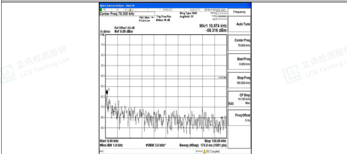
Band4-3MHz-QPSK-20385-1RB#0-0.009~0.15-PASS
