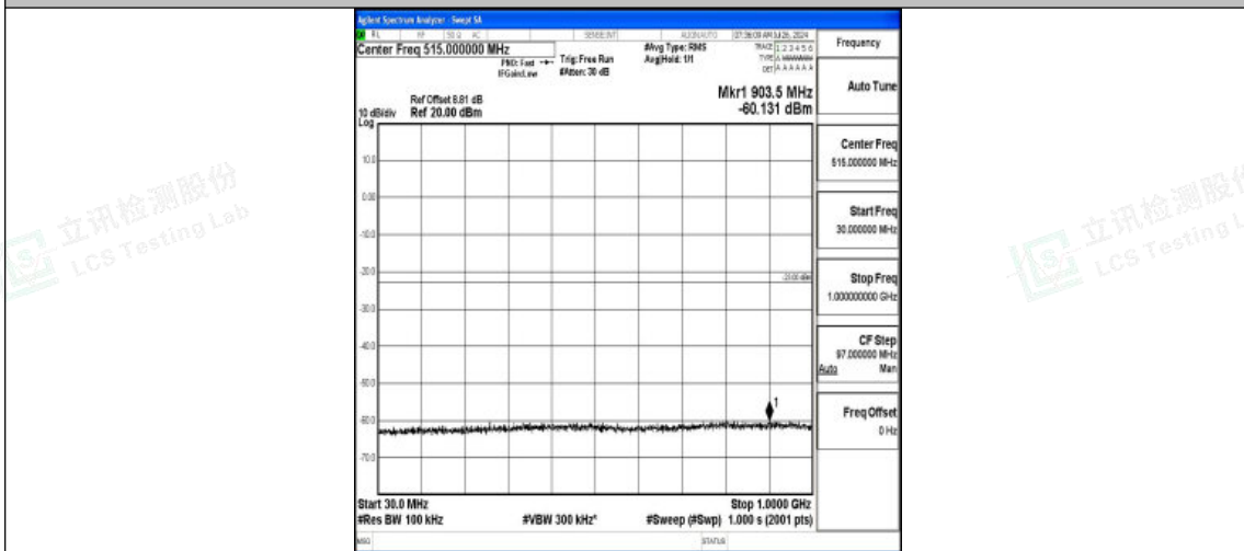
Band4-20MHz-16QAM-20175-1RB#0-30~1000-PASS
