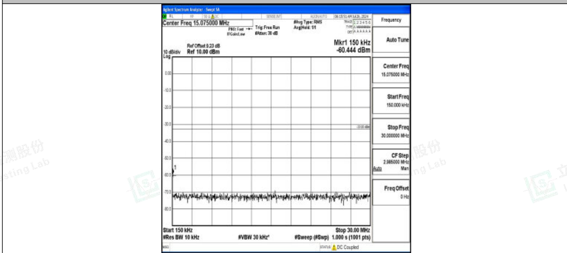
Band4-5MHz-QPSK-19975-1RB#0-0.15~30-PASS
