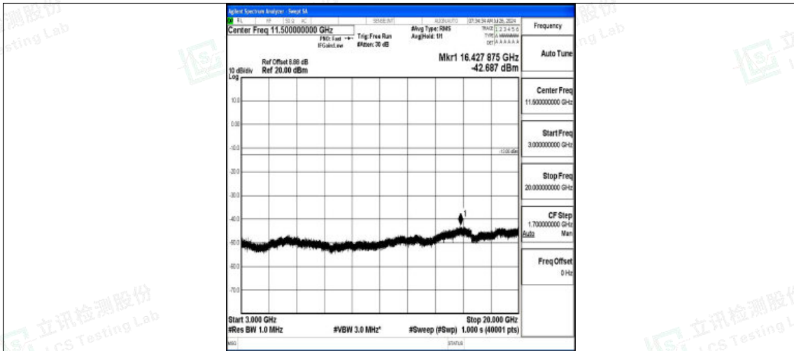
Band4-20MHz-16QAM-20050-1RB#0-3000~20000-PASS
