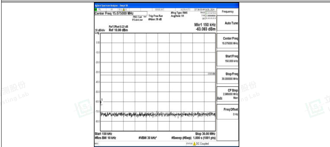
Band4-20MHz-16QAM-20175-1RB#0-0.15~30-PASS
