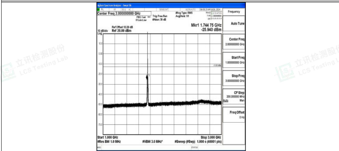
Band4-3MHz-QPSK-20385-1RB#0-1000~3000-PASS
