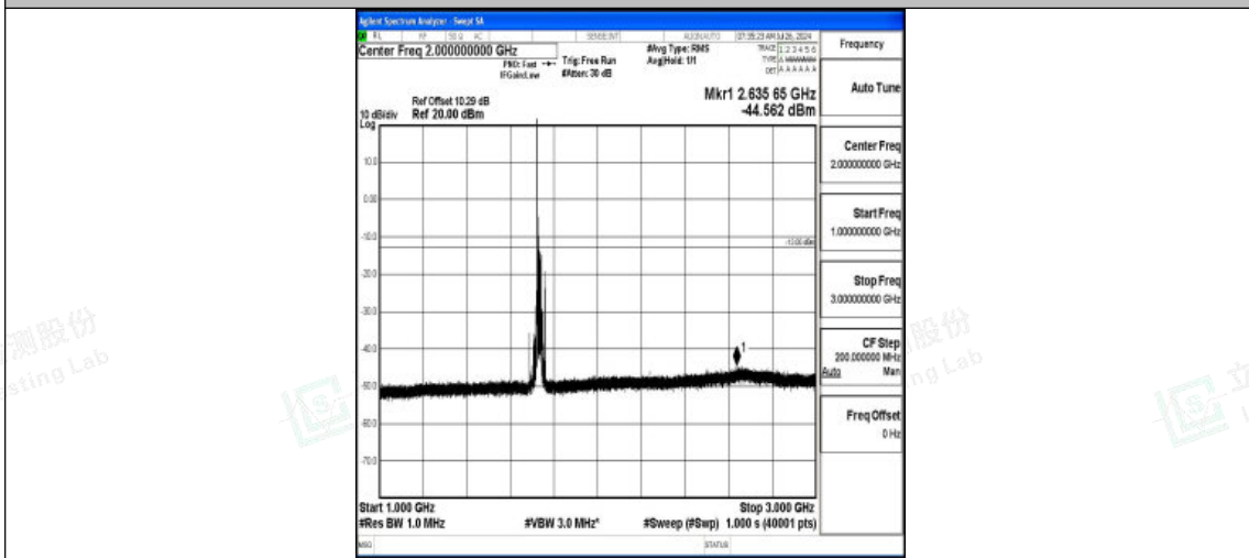
Band4-20MHz-QPSK-20175-1RB#0-1000~3000-PASS
