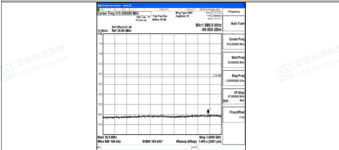
Band4-3MHz-QPSK-19965-1RB#0-30~1000-PASS
