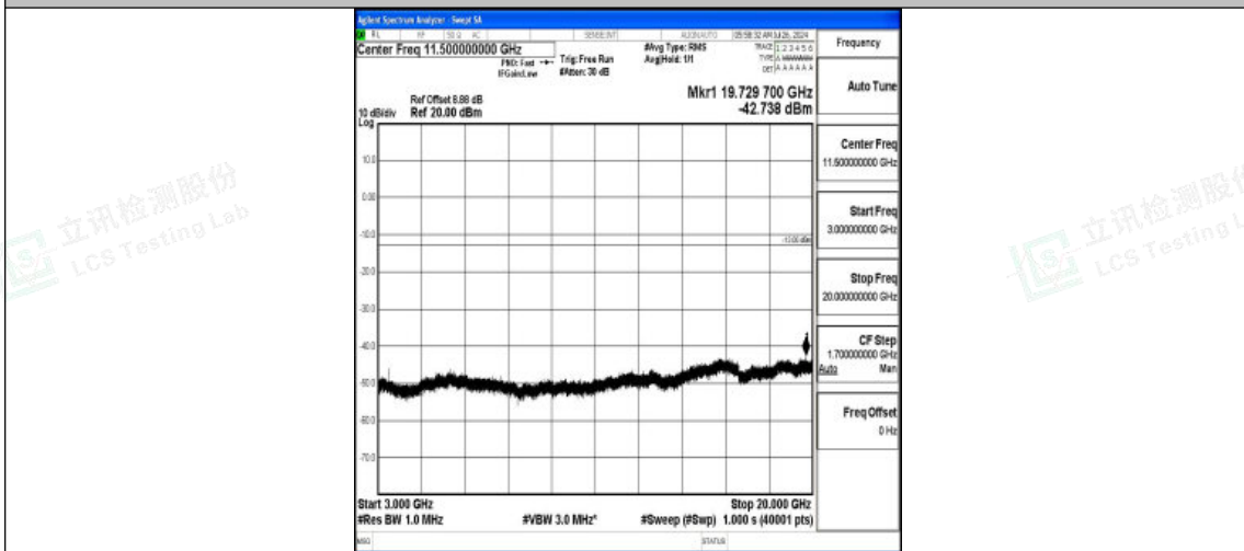
Band4-3MHz-QPSK-20175-1RB#0-3000~20000-PASS
