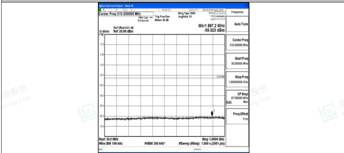
Band4-5MHz-QPSK-20375-1RB#0-30~1000-PASS
