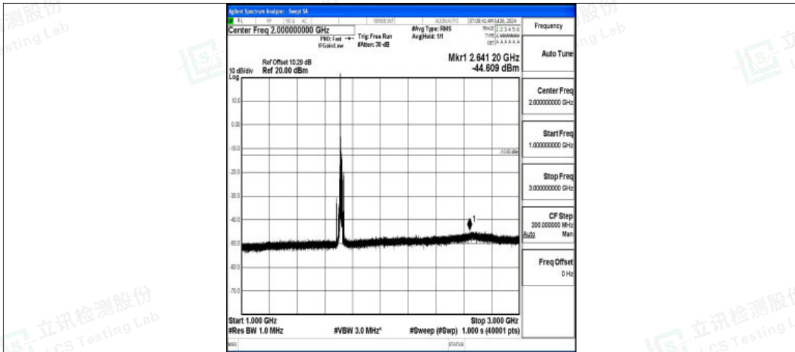
Band4-15MHz-QPSK-20025-1RB#0-1000~3000-PASS
