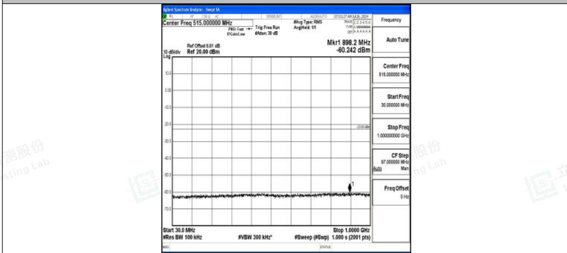
Band4-15MHz-16QAM-20025-1RB#0-30~1000-PASS
