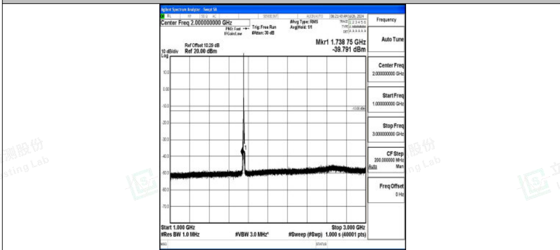
Band4-5MHz-16QAM-20375-1RB#0-1000~3000-PASS
