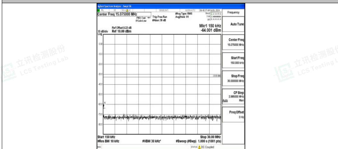
Band4-10MHz-16QAM-20350-1RB#0-0.15~30-PASS
