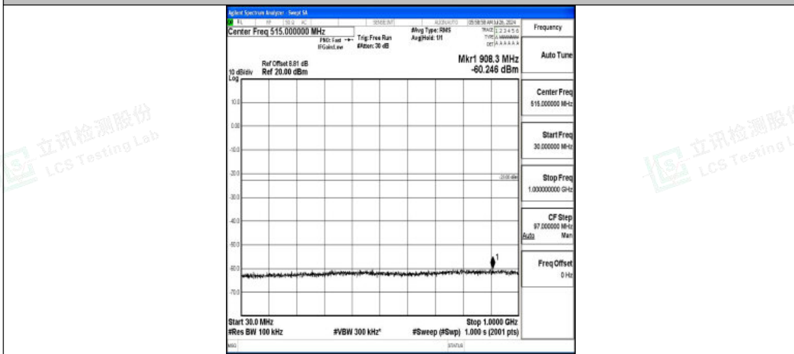
Band4-3MHz-16QAM-20175-1RB#0-30~1000-PASS
