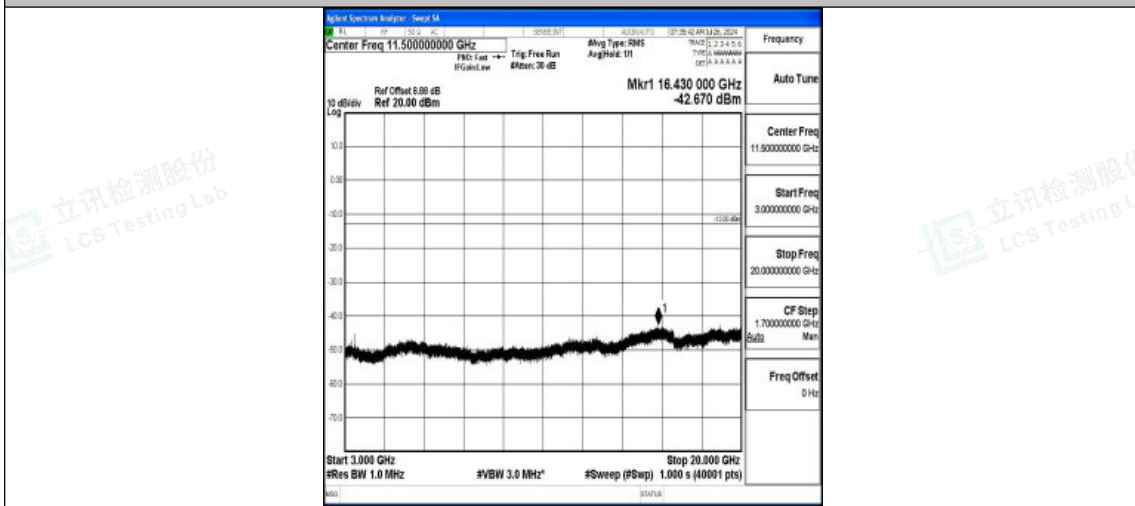
Band4-20MHz-QPSK-20175-1RB#0-3000~20000-PASS
