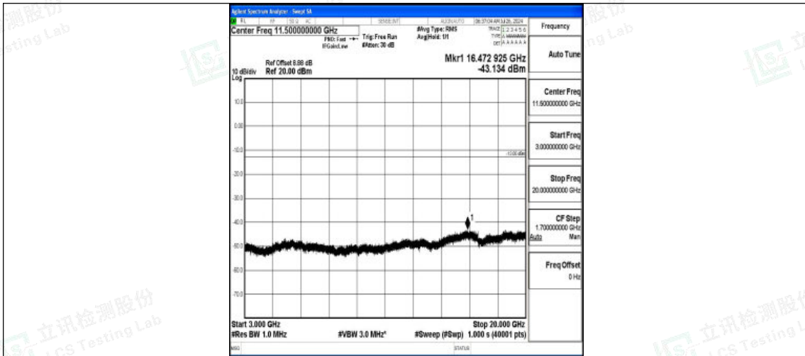
Band4-10MHz-16QAM-20000-1RB#0-3000~20000-PASS
