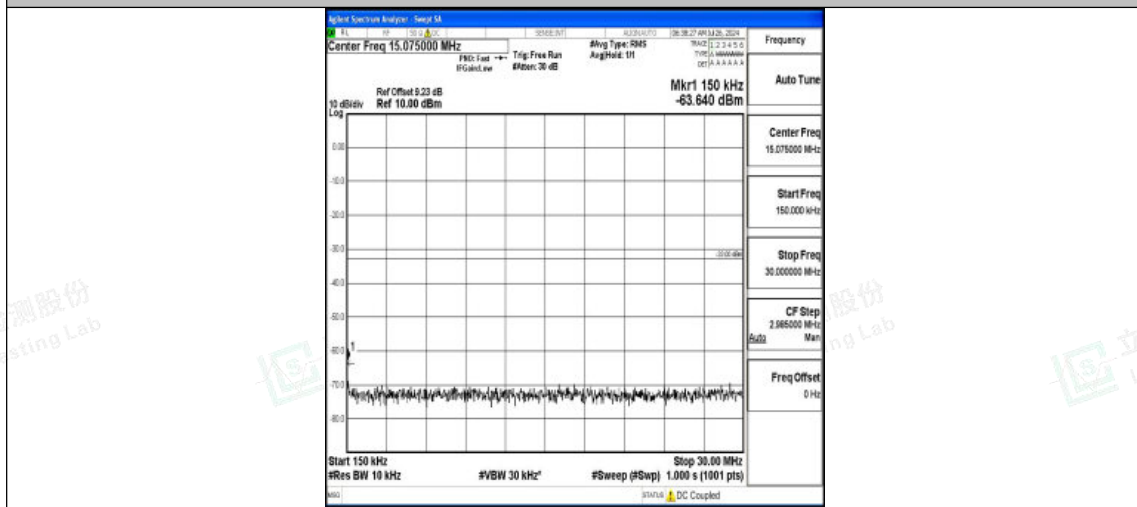
Band4-10MHz-16QAM-20175-1RB#0-0.15~30-PASS
