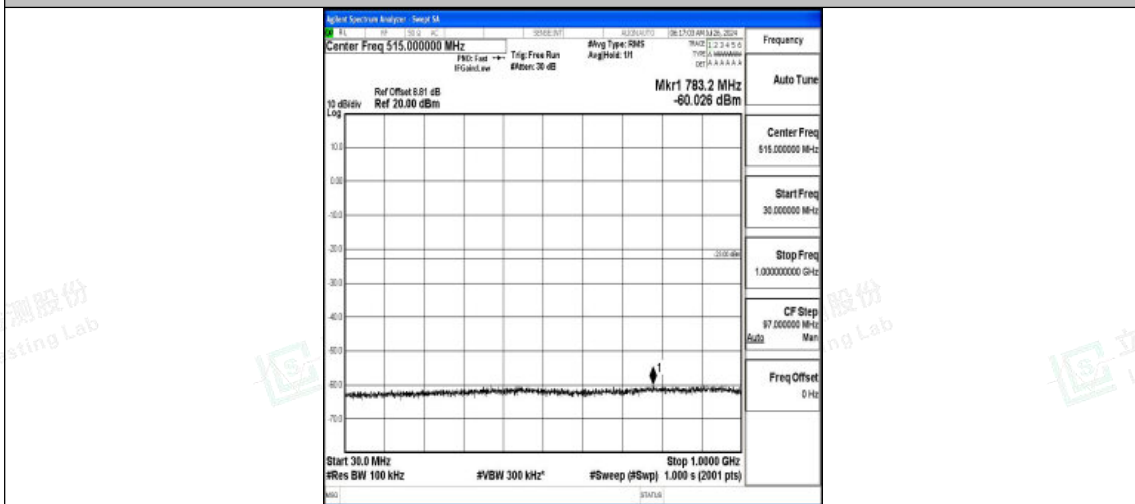
Band4-5MHz-16QAM-19975-1RB#0-30~1000-PASS
