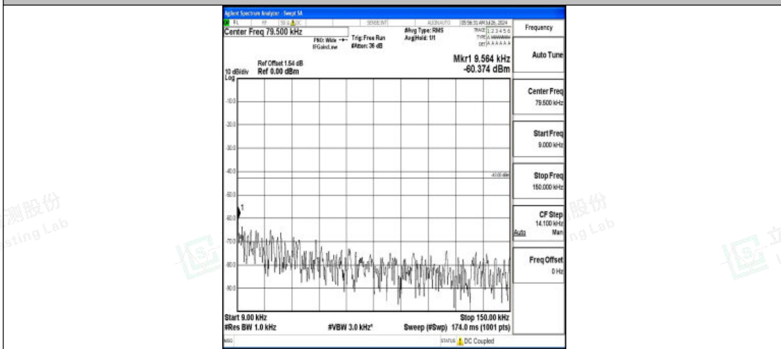
Band4-3MHz-16QAM-19965-1RB#0-0.009~0.15-PASS
