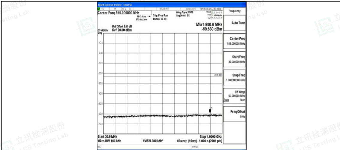
Band4-20MHz-QPSK-20175-1RB#0-30~1000-PASS
