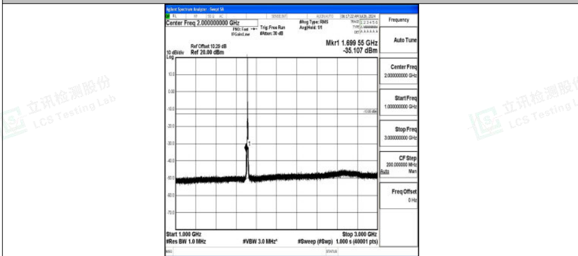
Band4-5MHz-16QAM-19975-1RB#0-1000~3000-PASS
