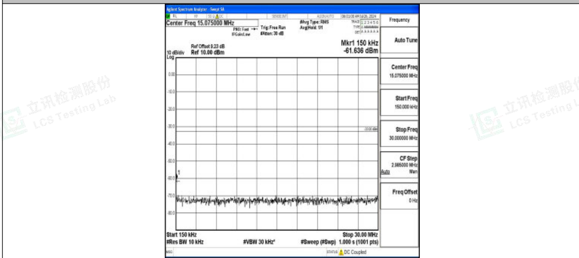
Band4-3MHz-16QAM-20385-1RB#0-0.15~30-PASS
