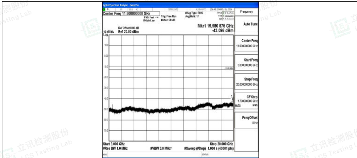
Band4-10MHz-QPSK-20350-1RB#0-3000~20000-PASS
