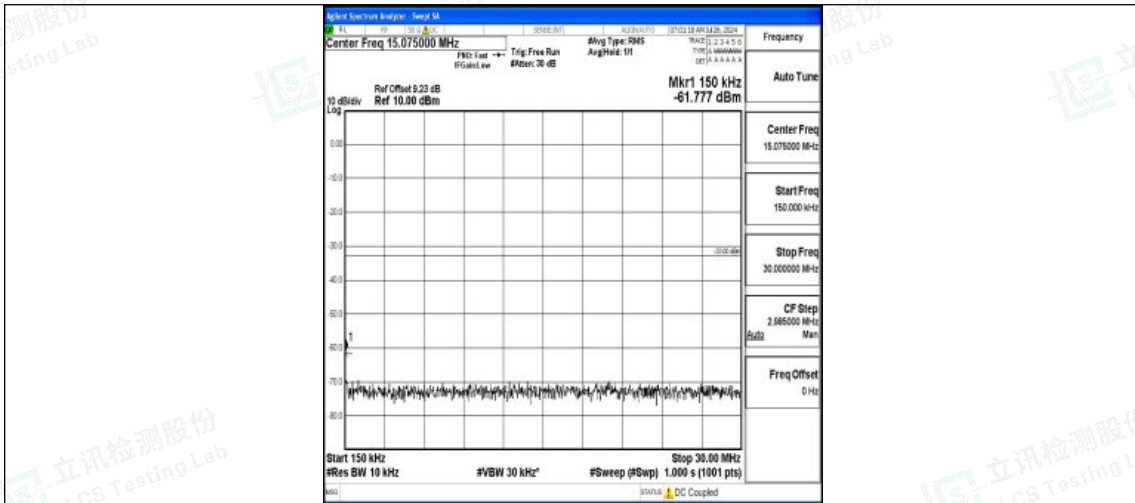
Band4-15MHz-16QAM-20025-1RB#0-0.15~30-PASS
