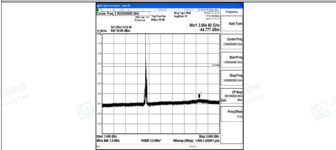
Band4-15MHz-16QAM-20325-1RB#0-1000~3000-PASS
