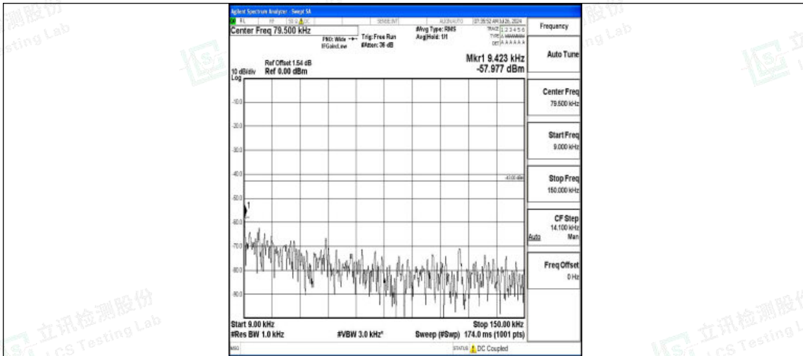
Band4-20MHz-16QAM-20175-1RB#0-0.009~0.15-PASS
