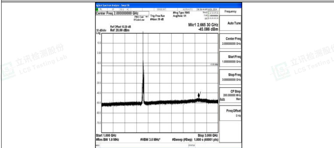
Band4-10MHz-16QAM-20000-1RB#0-1000~3000-PASS
