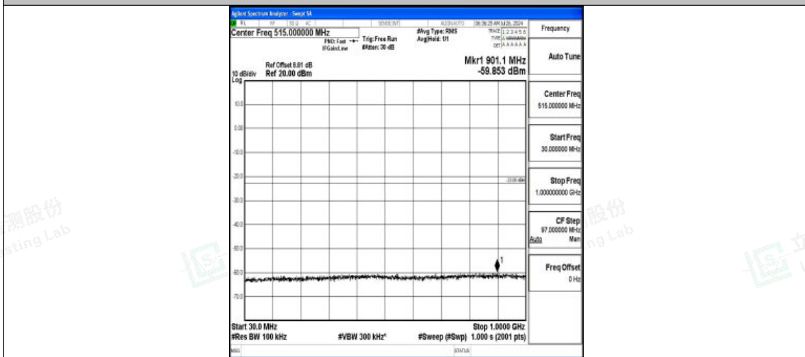
Band4-10MHz-16QAM-20000-1RB#0-30~1000-PASS
