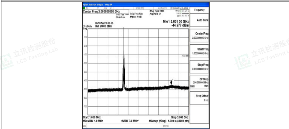
Band4-15MHz-16QAM-20025-1RB#0-1000~3000-PASS
