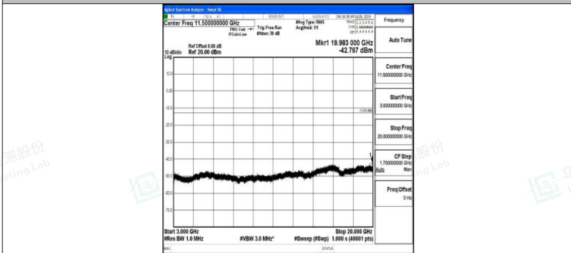
Band4-5MHz-QPSK-19975-1RB#0-3000~20000-PASS
