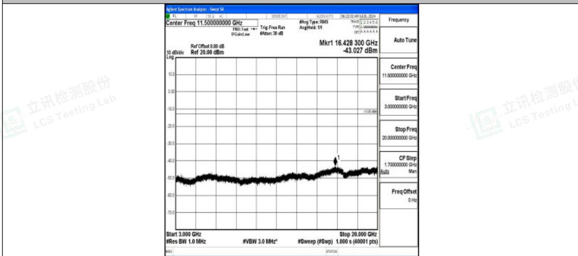
Band4-5MHz-16QAM-20375-1RB#0-3000~20000-PASS
