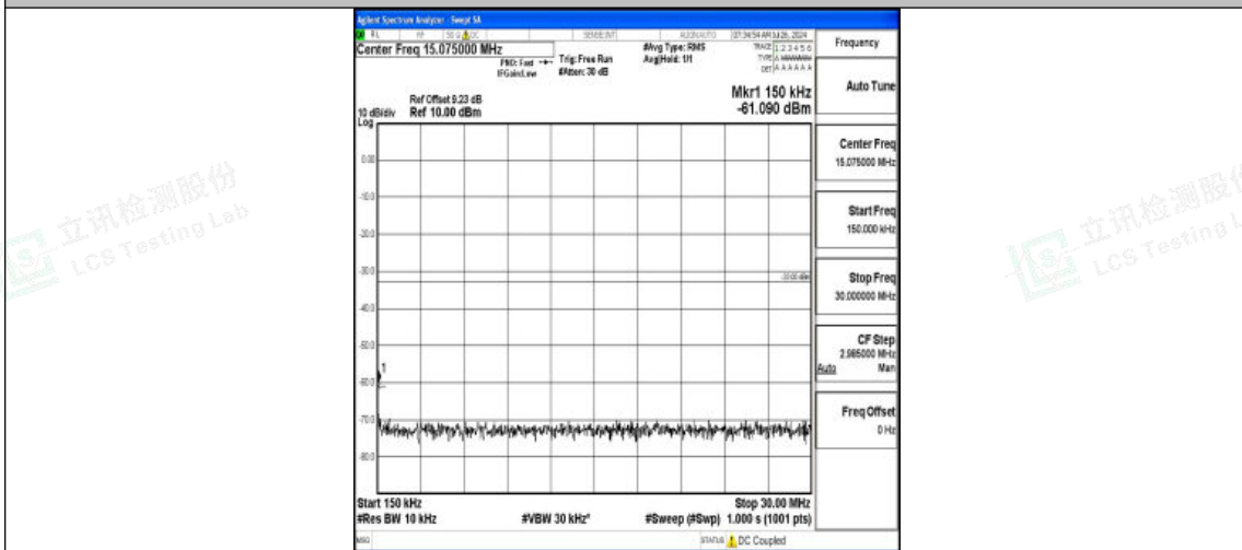
Band4-20MHz-QPSK-20175-1RB#0-0.15~30-PASS
