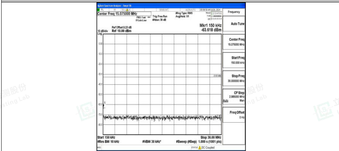
Band4-3MHz-16QAM-20175-1RB#0-0.15~30-PASS
