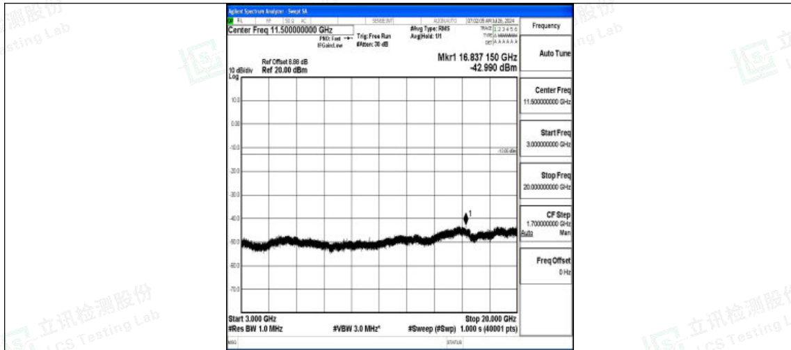
Band4-15MHz-16QAM-20025-1RB#0-3000~20000-PASS
