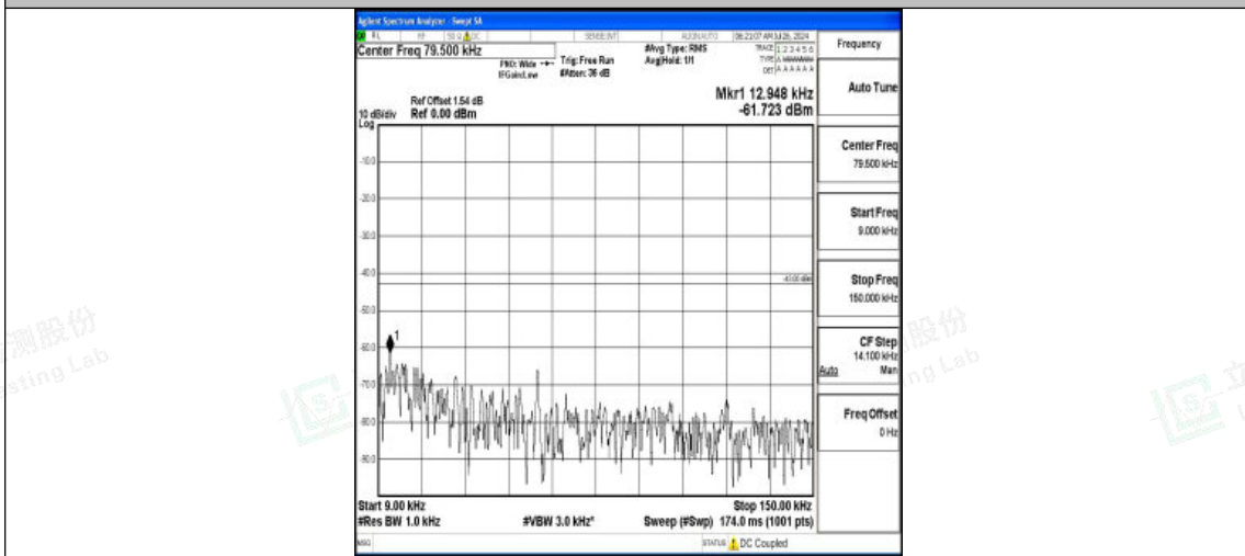
Band4-5MHz-16QAM-20375-1RB#0-0.009~0.15-PASS
