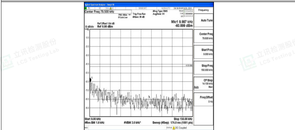
Band4-10MHz-16QAM-20000-1RB#0-0.009~0.15-PASS
