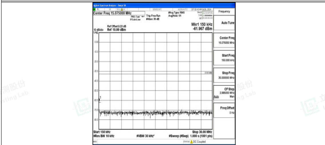
Band4-20MHz-QPSK-20050-1RB#0-0.15~30-PASS
