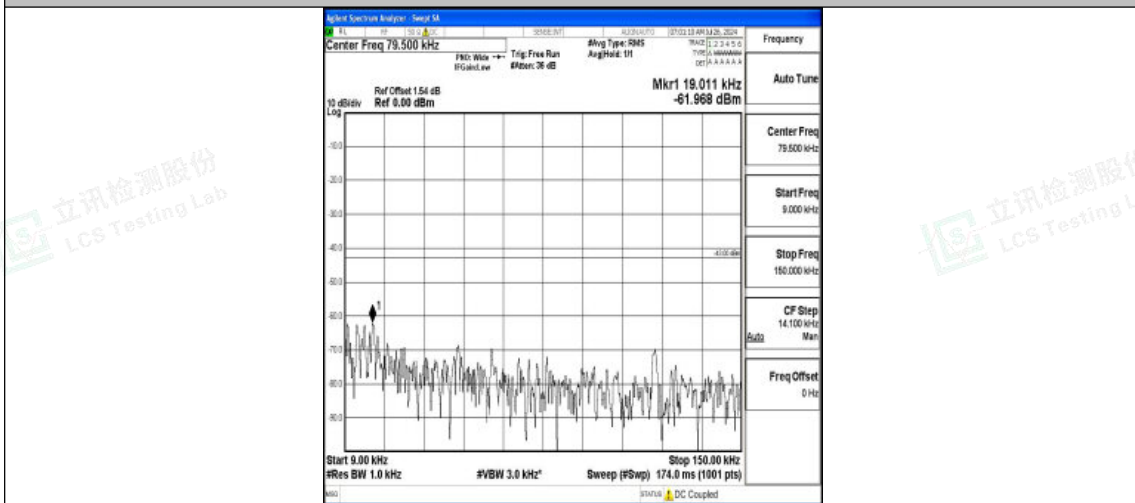
Band4-15MHz-16QAM-20025-1RB#0-0.009~0.15-PASS
