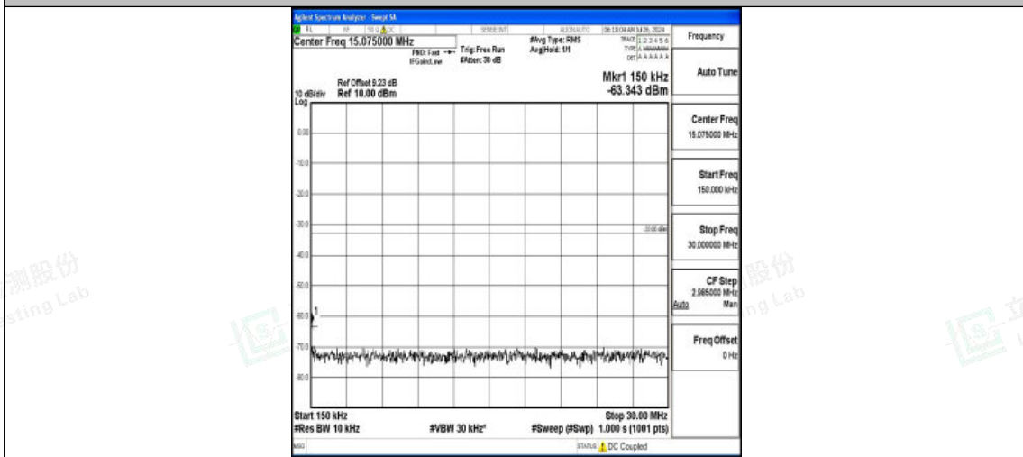
Band4-5MHz-16QAM-20175-1RB#0-0.15~30-PASS
