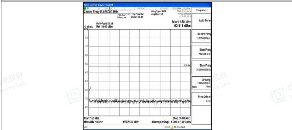
Band2-3MHz-16QAM-18900-1RB#0-0.15~30-PASS
