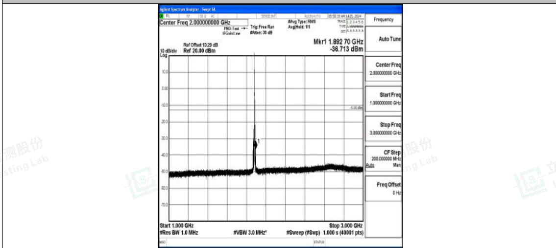
Band2-5MHz-QPSK-18900-1RB#0-1000~3000-PASS
