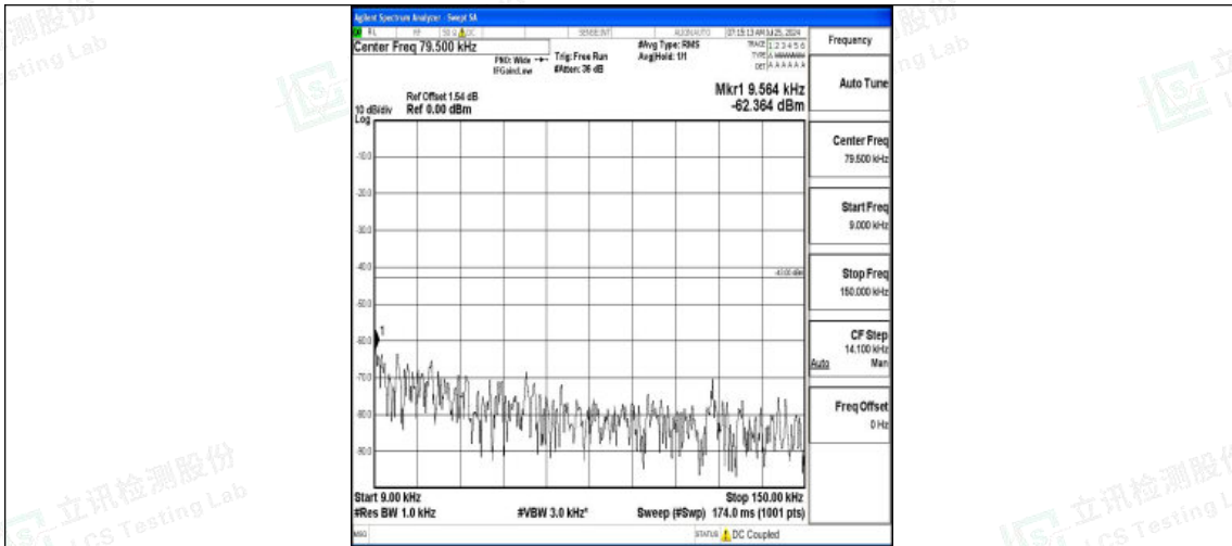
Band2-20MHz-16QAM-18900-1RB#0-0.009~0.15-PASS
