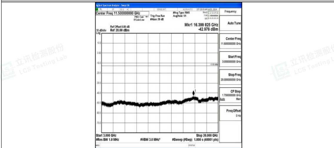
Band2-20MHz-QPSK-18900-1RB#0-3000~20000-PASS
