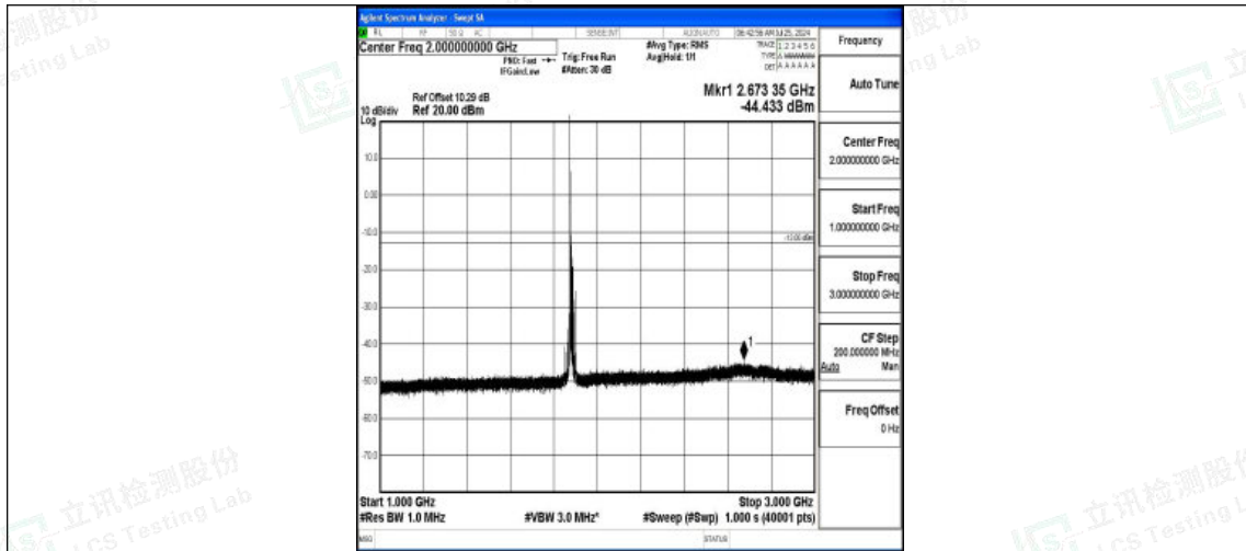
Band2-15MHz-16QAM-18900-1RB#0-1000~3000-PASS
