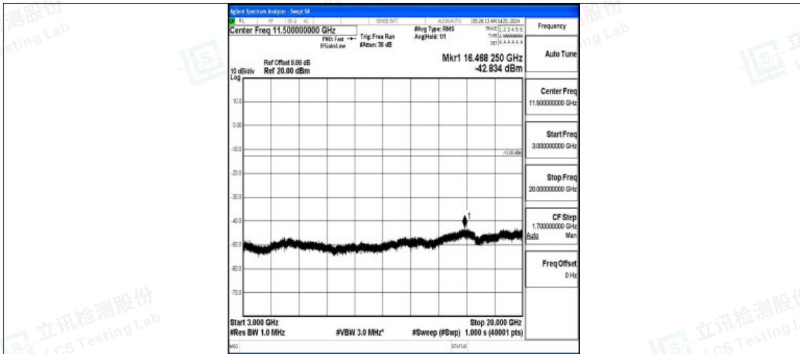
Band2-3MHz-16QAM-18615-1RB#0-3000~20000-PASS
