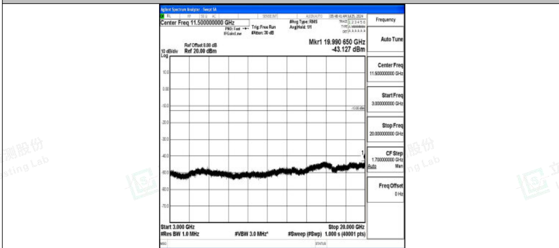
Band2-5MHz-QPSK-18625-1RB#0-3000~20000-PASS
