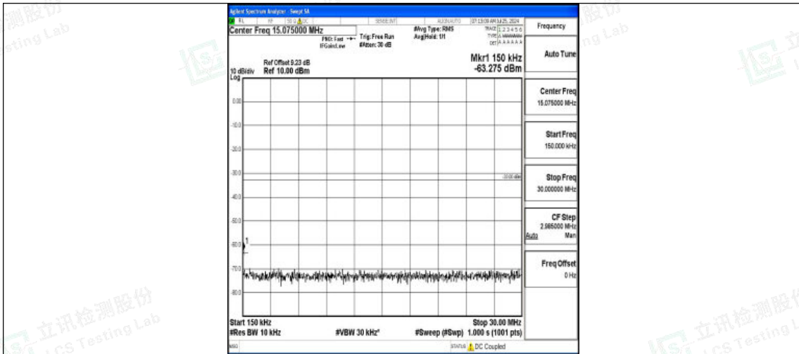
Band2-20MHz-16QAM-18700-1RB#0-0.15~30-PASS
