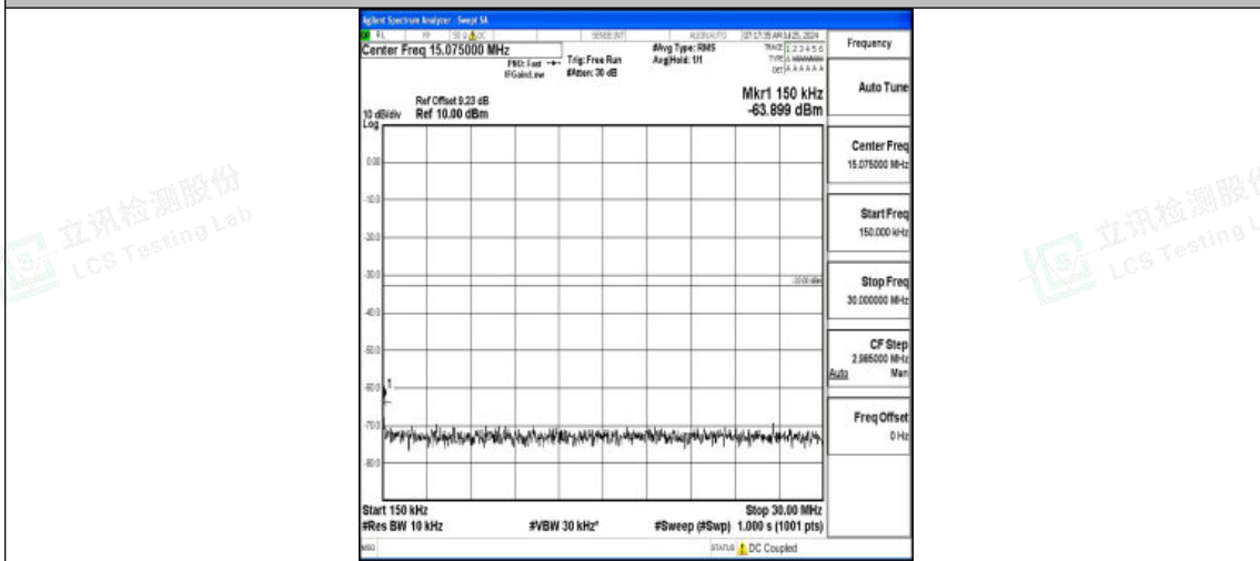
Band2-20MHz-16QAM-19100-1RB#0-0.15~30-PASS
