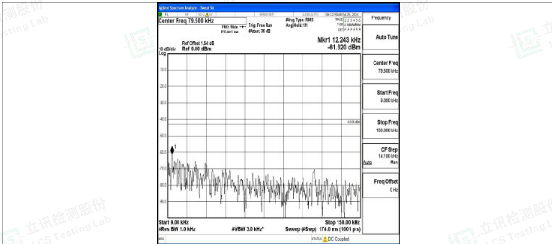
Band2-10MHz-16QAM-18900-1RB#0-0.009~0.15-PASS
