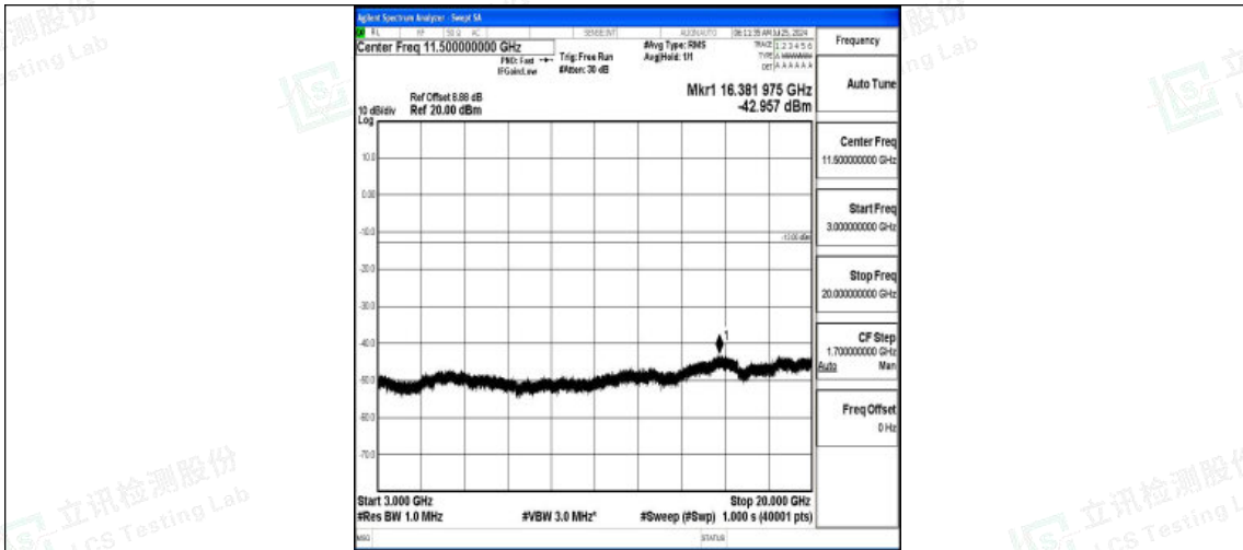
Band2-10MHz-16QAM-18650-1RB#0-3000~20000-PASS
