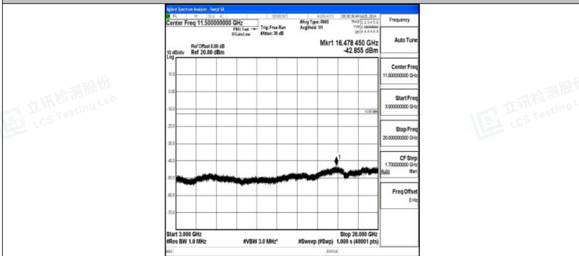
Band2-3MHz-16QAM-19185-1RB#0-3000~20000-PASS
