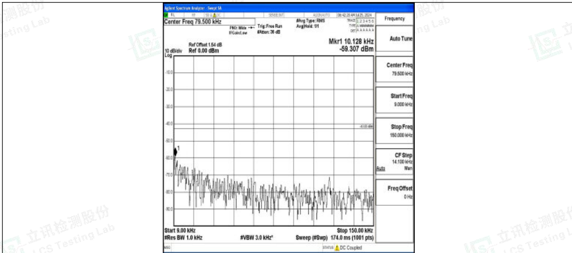
Band2-15MHz-16QAM-18900-1RB#0-0.009~0.15-PASS
