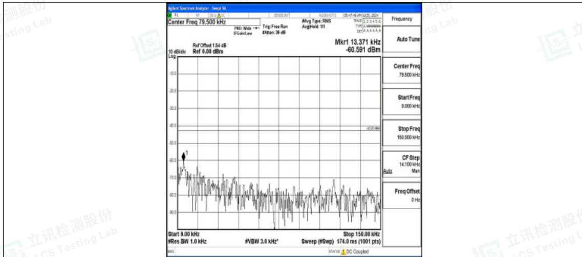
Band2-5MHz-QPSK-18625-1RB#0-0.009~0.15-PASS
