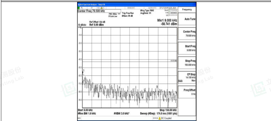
Band2-20MHz-16QAM-19100-1RB#0-0.009~0.15-PASS
