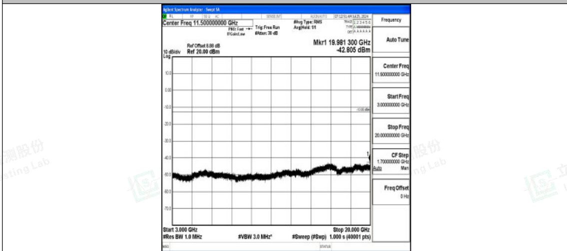
Band2-20MHz-QPSK-18700-1RB#0-3000~20000-PASS
