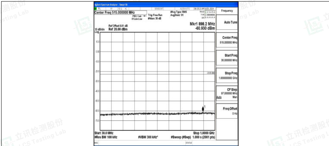
Band2-10MHz-16QAM-19150-1RB#0-30~1000-PASS
