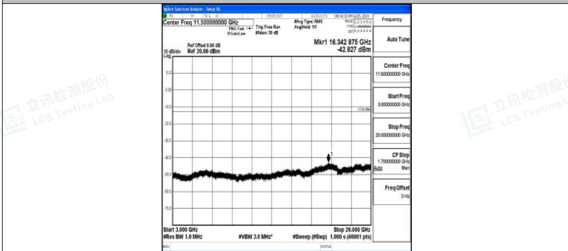
Band2-15MHz-QPSK-18900-1RB#0-3000~20000-PASS
