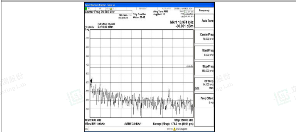
Band2-5MHz-16QAM-19175-1RB#0-0.009~0.15-PASS
