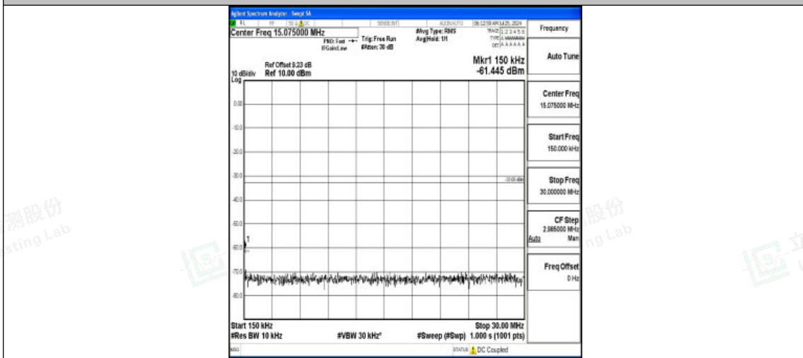
Band2-10MHz-16QAM-18900-1RB#0-0.15~30-PASS
