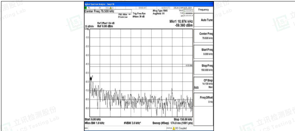
Band2-3MHz-QPSK-18615-1RB#0-0.009~0.15-PASS
