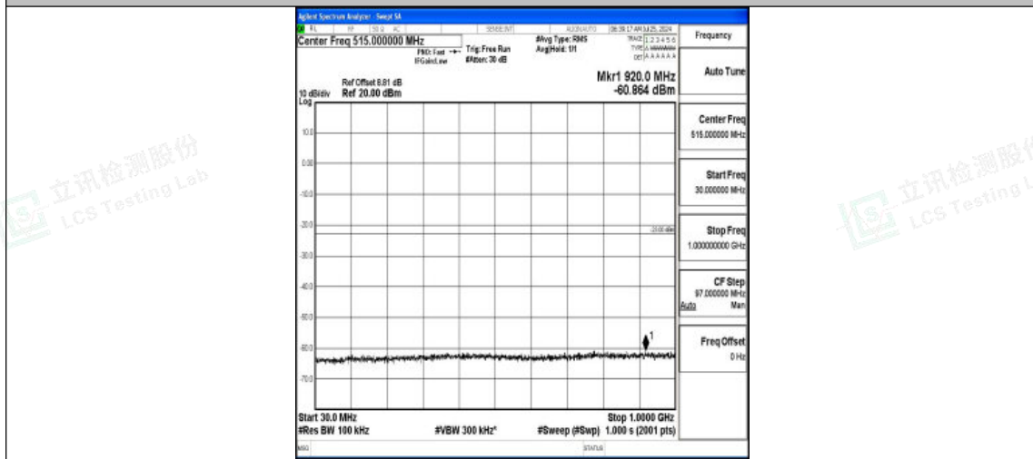
Band2-15MHz-QPSK-18675-1RB#0-30~1000-PASS
