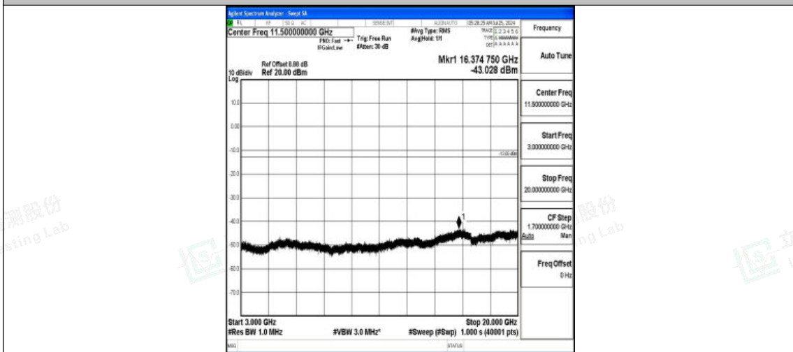
Band2-3MHz-16QAM-18900-1RB#0-3000~20000-PASS
