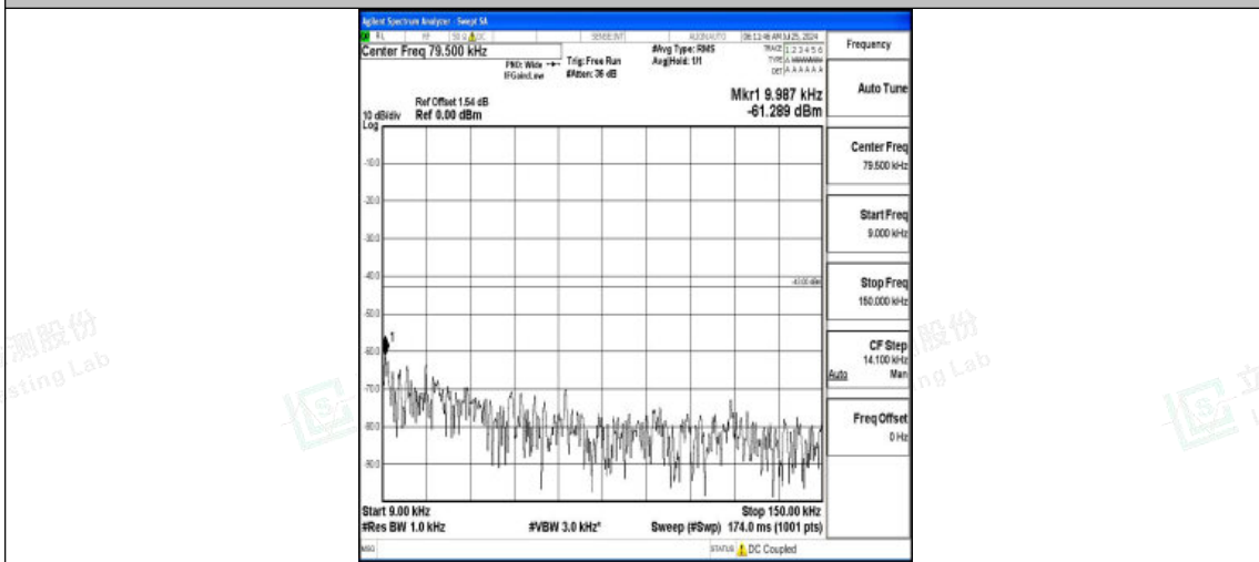
Band2-10MHz-QPSK-18900-1RB#0-0.009~0.15-PASS
