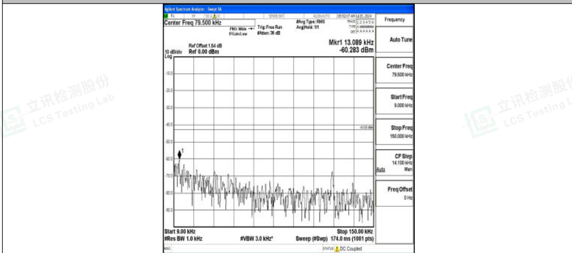
Band2-5MHz-QPSK-19175-1RB#0-0.009~0.15-PASS
