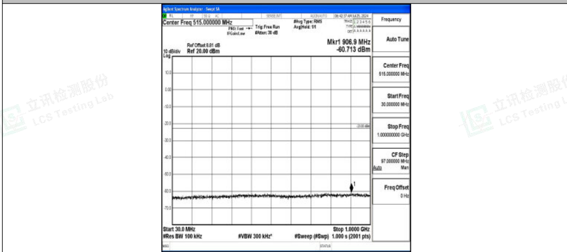
Band2-15MHz-16QAM-18900-1RB#0-30~1000-PASS
