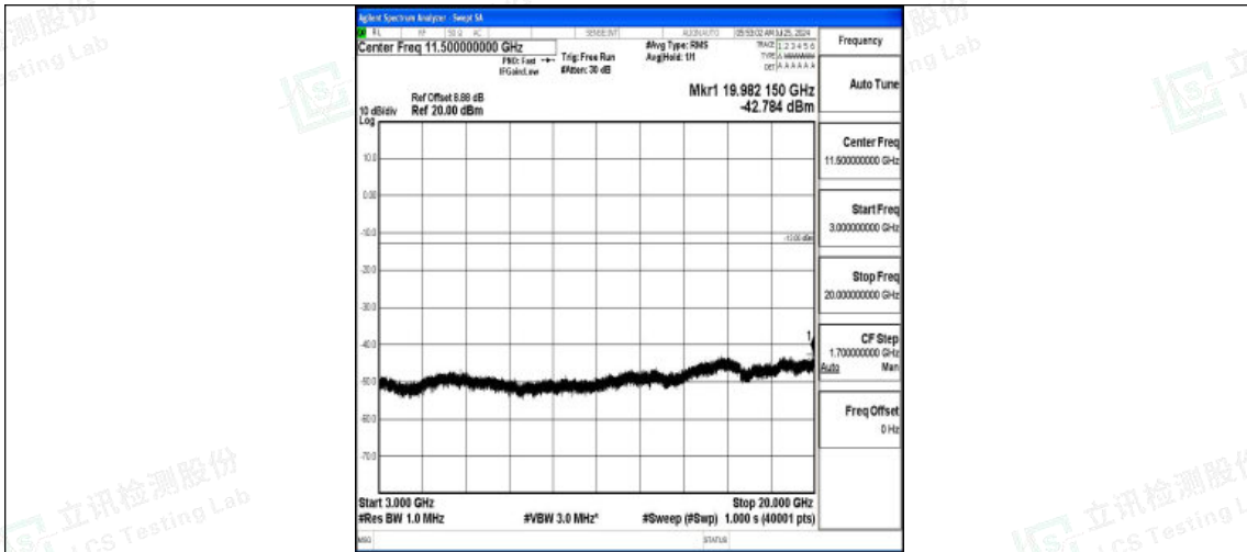
Band2-5MHz-QPSK-19175-1RB#0-3000~20000-PASS
