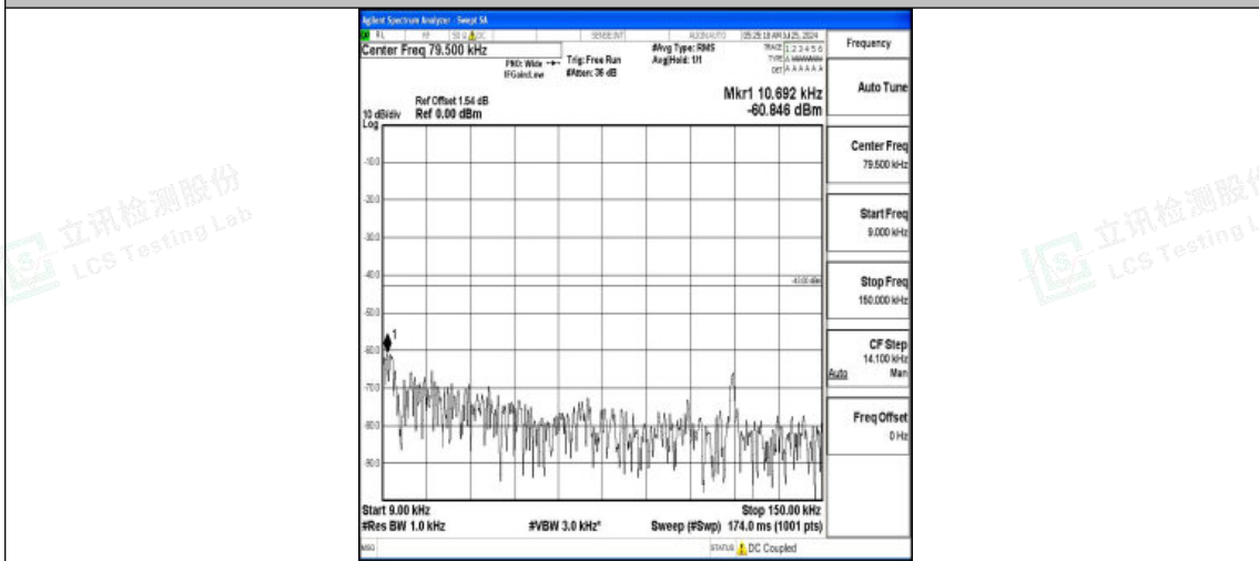
Band2-3MHz-16QAM-18615-1RB#0-0.009~0.15-PASS
