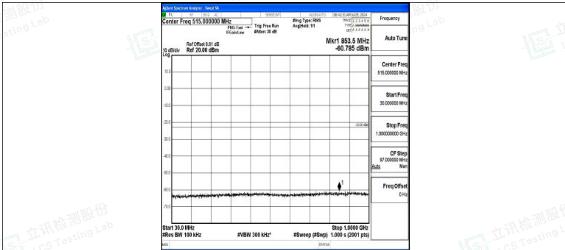
Band2-15MHz-QPSK-18900-1RB#0-30~1000-PASS
