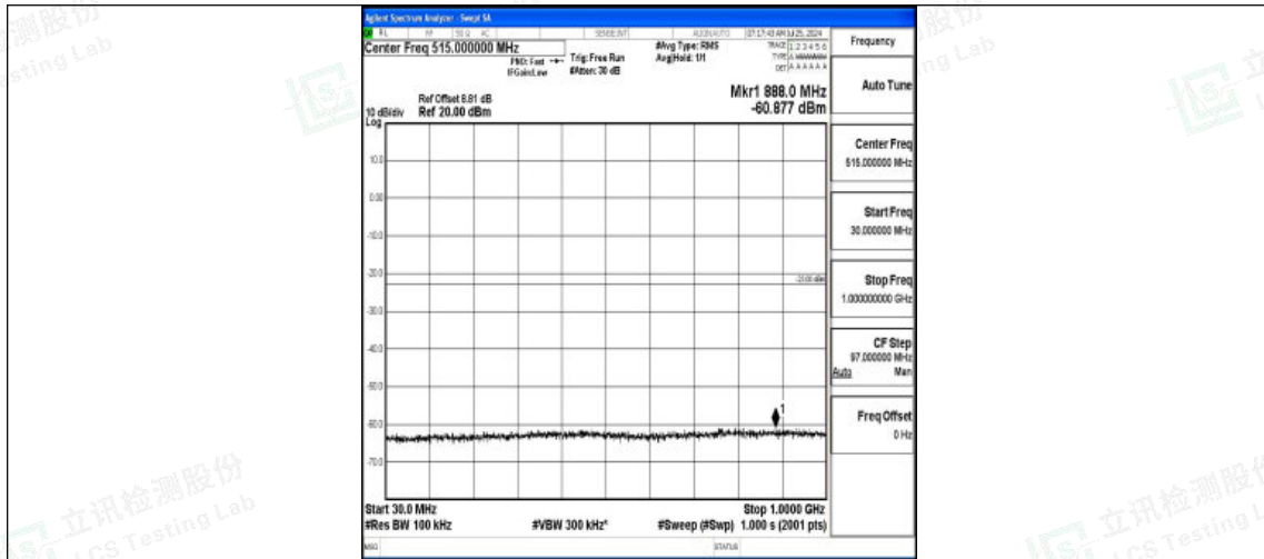
Band2-20MHz-16QAM-19100-1RB#0-30~1000-PASS
