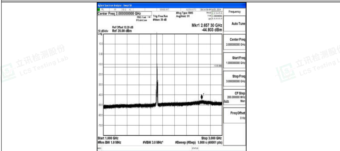
Band2-10MHz-QPSK-19150-1RB#0-1000~3000-PASS
