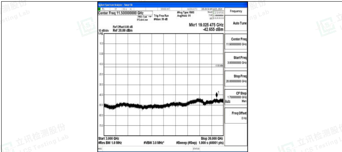
Band2-3MHz-QPSK-19185-1RB#0-3000~20000-PASS
