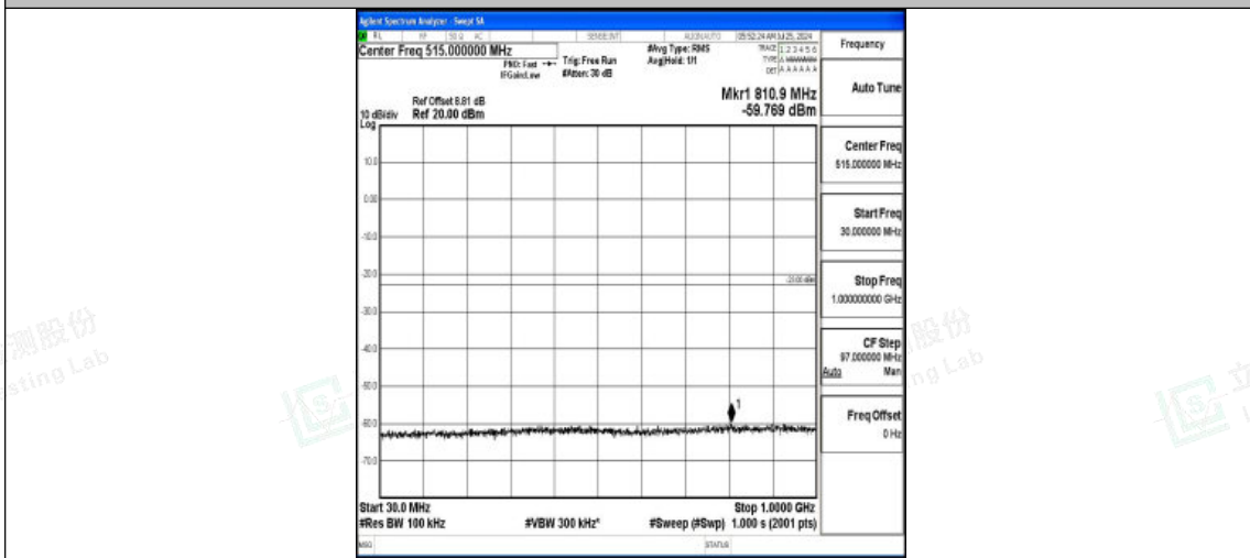
Band2-5MHz-QPSK-19175-1RB#0-30~1000-PASS
