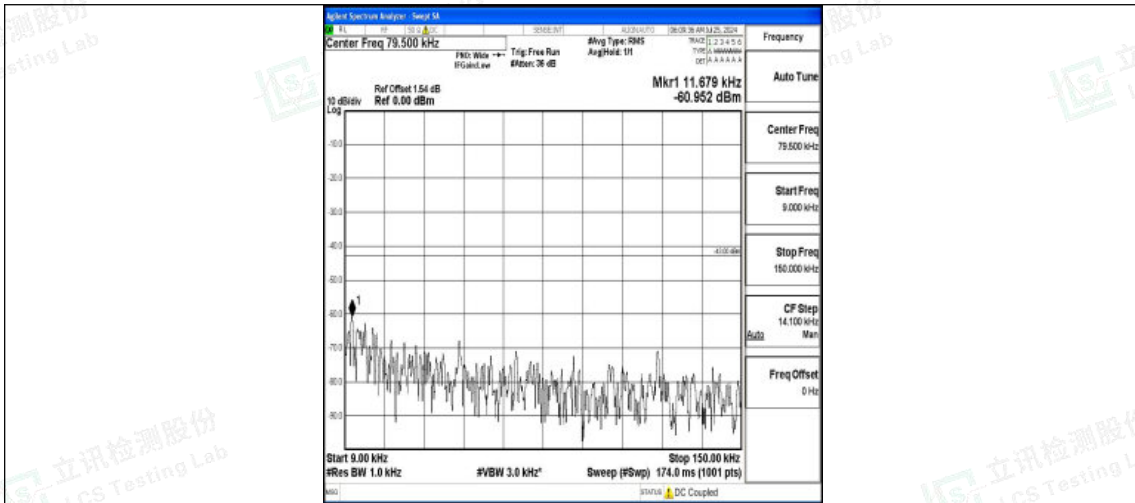
Band2-10MHz-QPSK-18650-1RB#0-0.009~0.15-PASS
