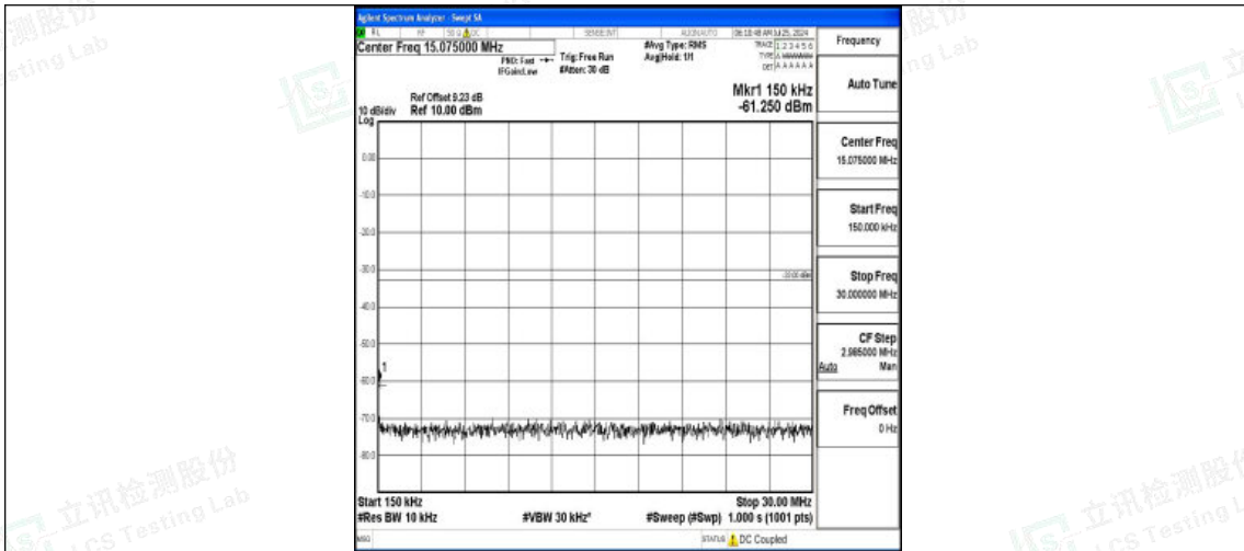
Band2-10MHz-16QAM-18650-1RB#0-0.15~30-PASS
