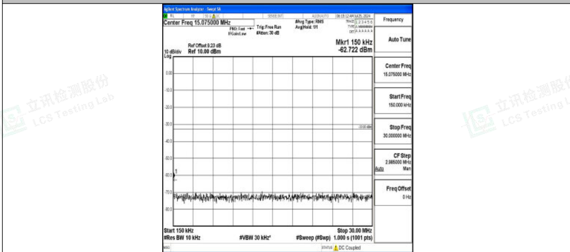
Band2-10MHz-16QAM-19150-1RB#0-0.15~30-PASS
