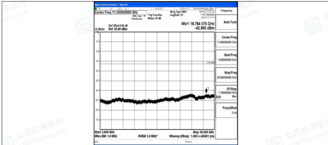
Band2-15MHz-16QAM-18675-1RB#0-3000~20000-PASS
