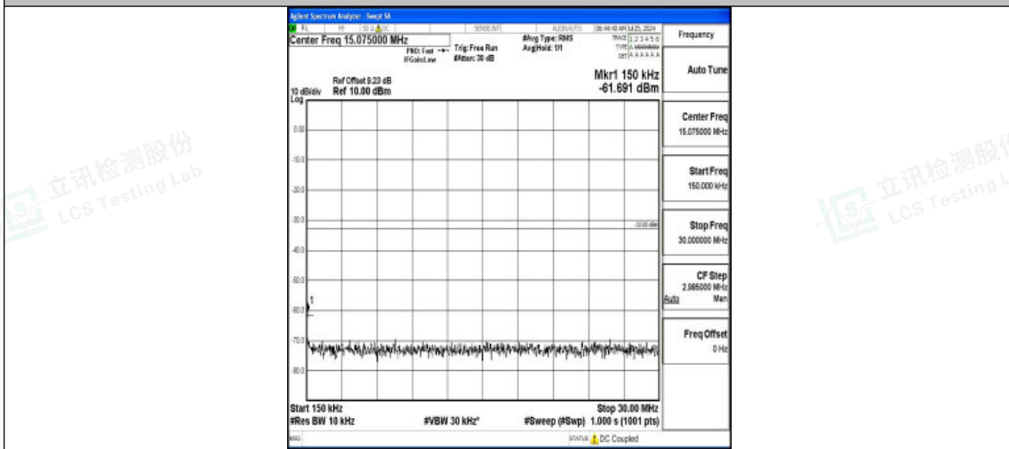
Band2-15MHz-16QAM-19125-1RB#0-0.15~30-PASS
