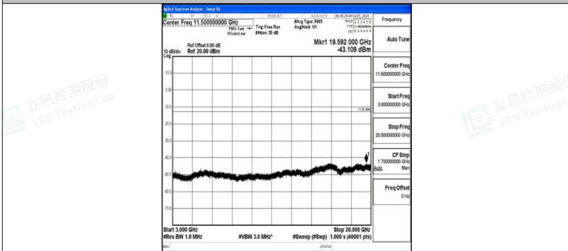
Band2-15MHz-16QAM-19125-1RB#0-3000~20000-PASS
