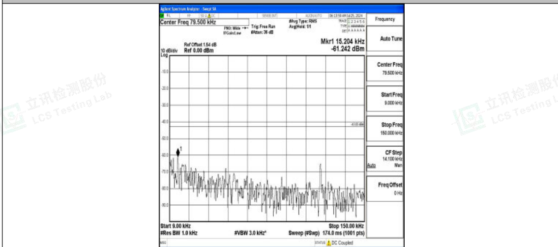
Band2-10MHz-QPSK-19150-1RB#0-0.009~0.15-PASS
