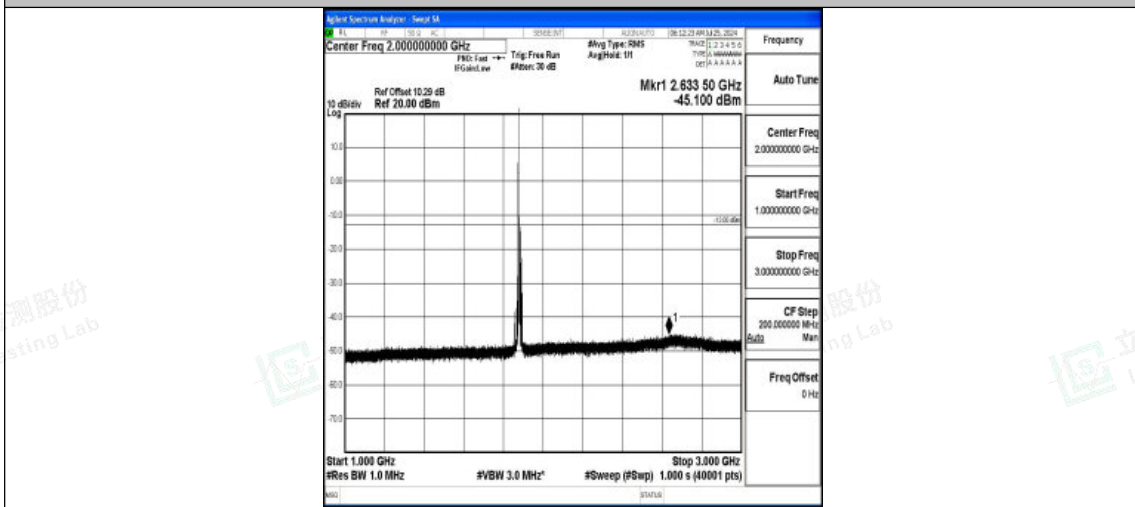
Band2-10MHz-QPSK-18900-1RB#0-1000~3000-PASS
