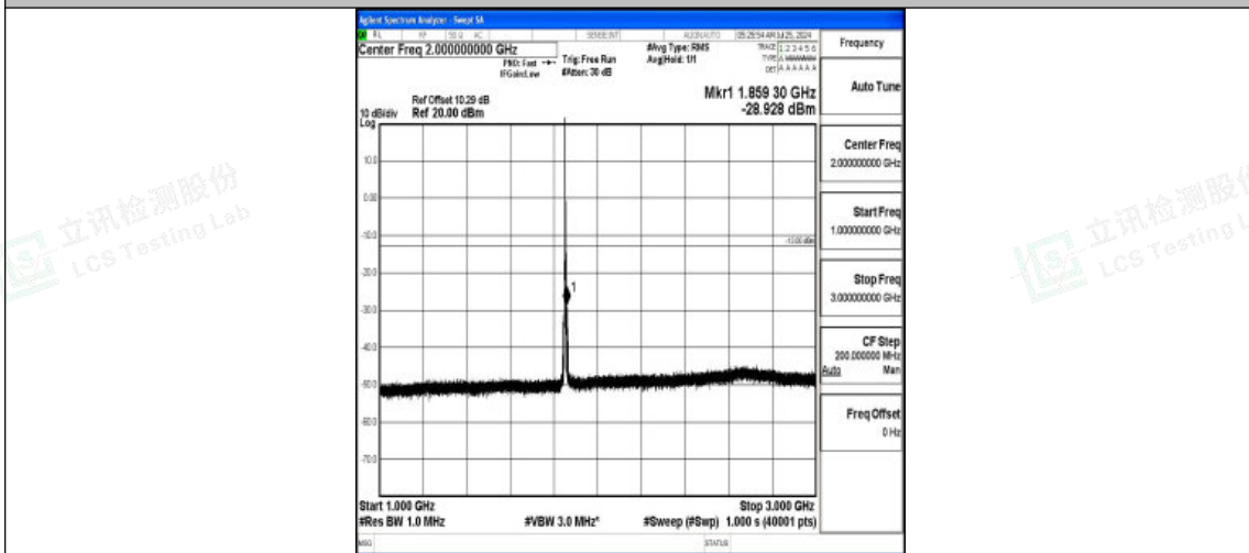
Band2-3MHz-16QAM-18615-1RB#0-1000~3000-PASS
