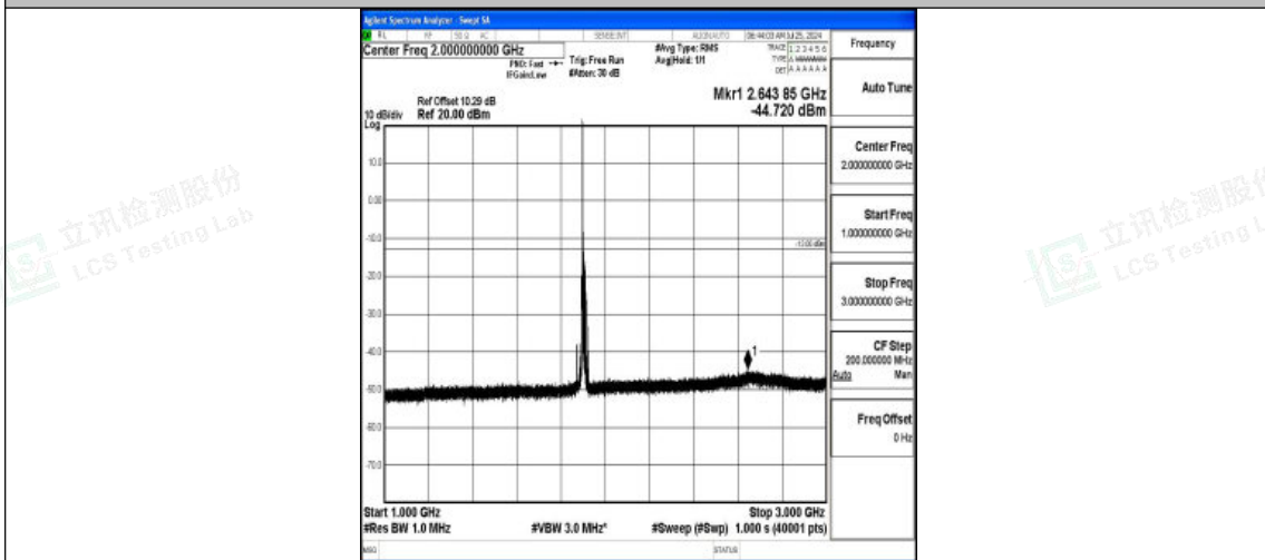
Band2-15MHz-QPSK-19125-1RB#0-1000~3000-PASS
