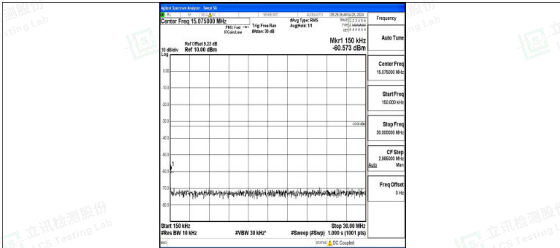
Band2-3MHz-16QAM-18615-1RB#0-0.15~30-PASS
