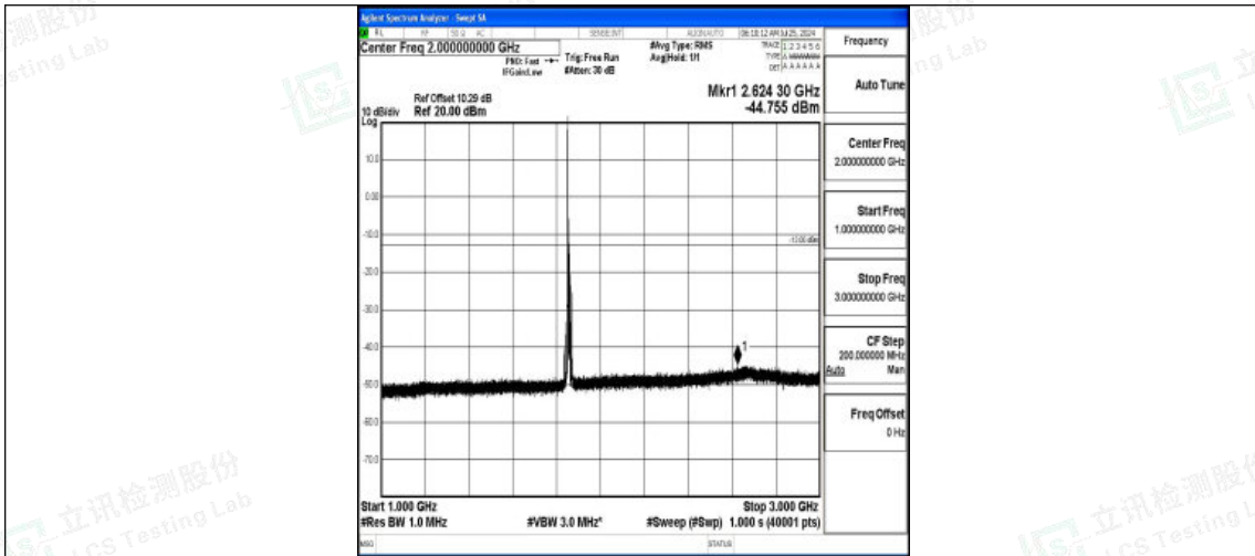
Band2-10MHz-QPSK-18650-1RB#0-1000~3000-PASS
