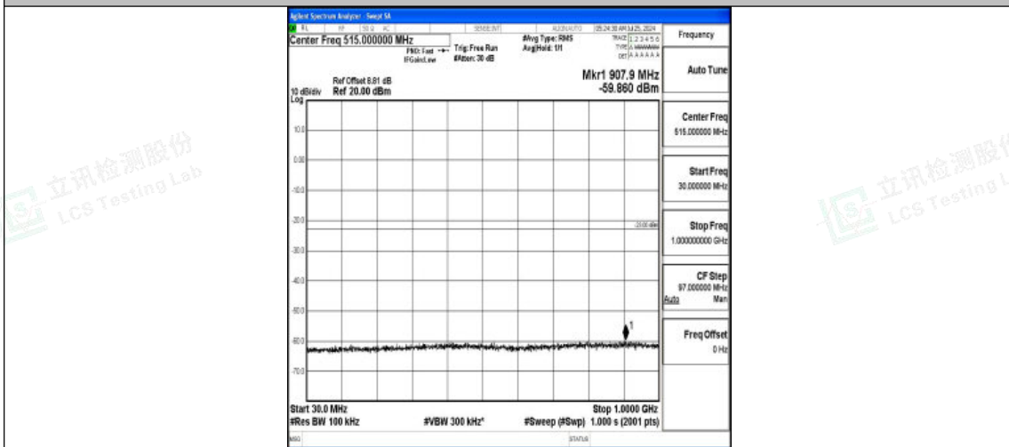
Band2-3MHz-QPSK-18615-1RB#0-30~1000-PASS
