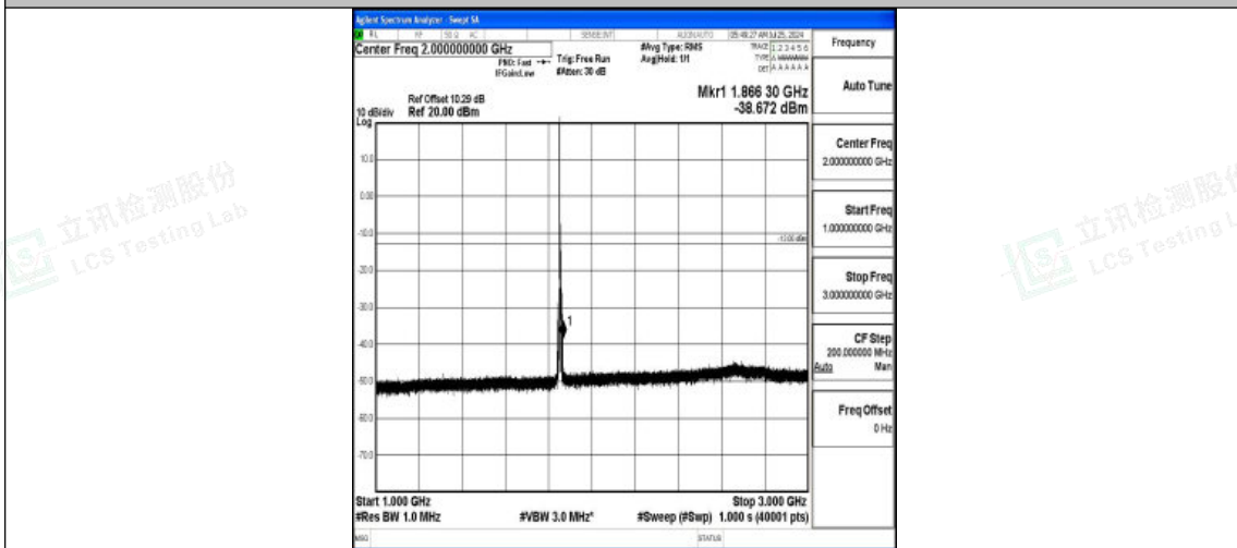
Band2-5MHz-16QAM-18625-1RB#0-1000~3000-PASS
