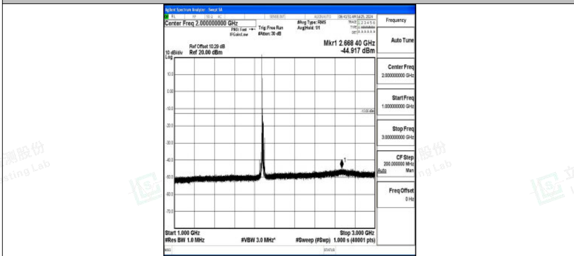
Band2-15MHz-QPSK-18900-1RB#0-1000~3000-PASS
