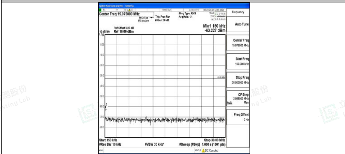
Band2-3MHz-QPSK-18615-1RB#0-0.15~30-PASS
