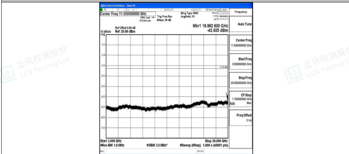
Band2-5MHz-16QAM-19175-1RB#0-3000~20000-PASS
