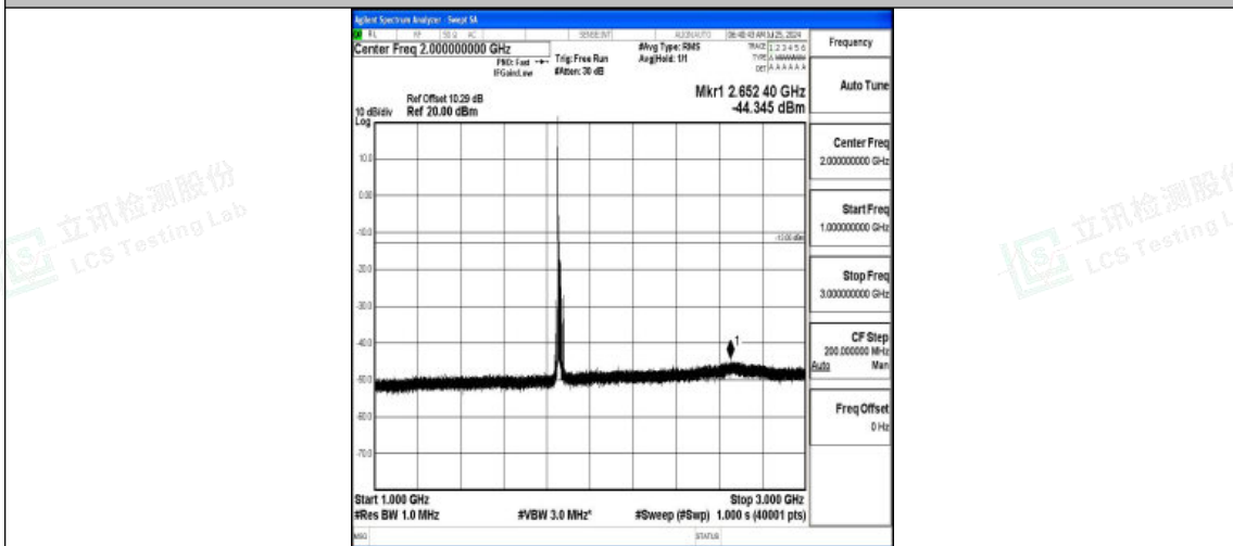
Band2-15MHz-16QAM-18675-1RB#0-1000~3000-PASS
