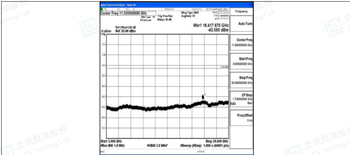
Band2-20MHz-QPSK-19100-1RB#0-3000~20000-PASS
