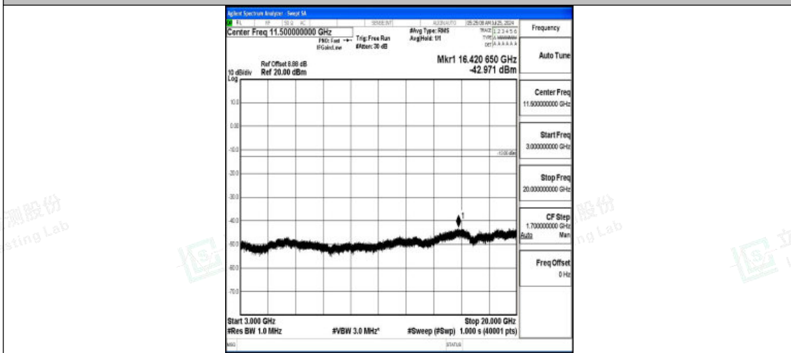
Band2-3MHz-QPSK-18615-1RB#0-3000~20000-PASS
