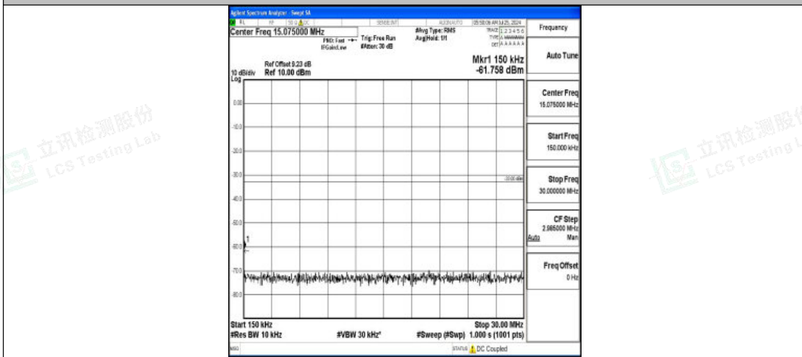
Band2-5MHz-QPSK-18900-1RB#0-0.15~30-PASS
