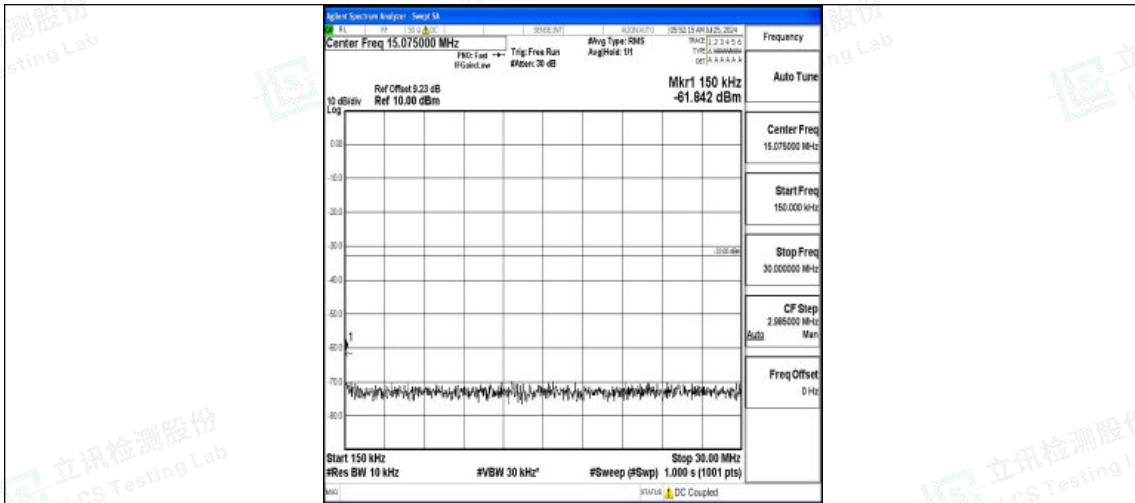
Band2-5MHz-QPSK-19175-1RB#0-0.15~30-PASS
