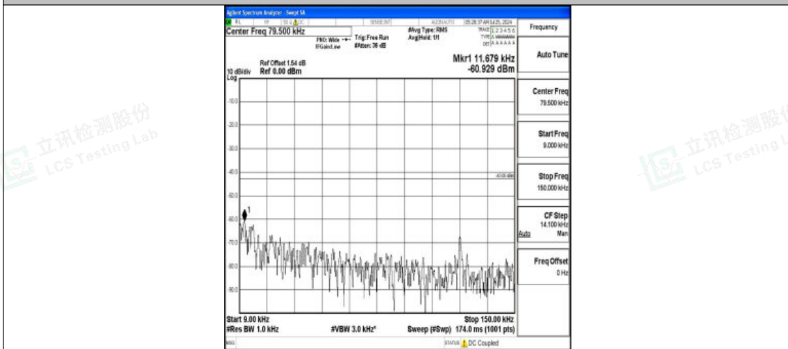
Band2-3MHz-QPSK-19185-1RB#0-0.009~0.15-PASS
