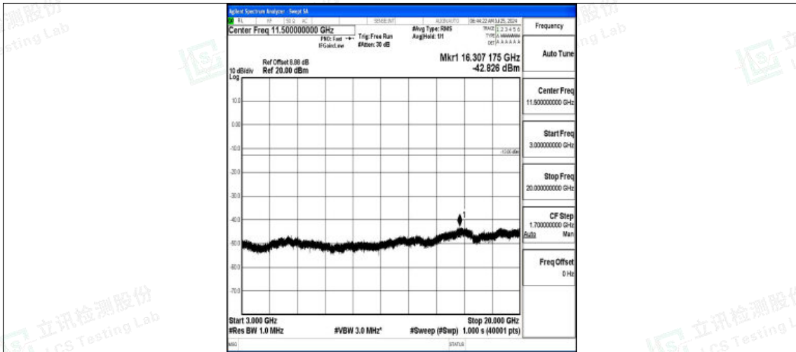
Band2-15MHz-QPSK-19125-1RB#0-3000~20000-PASS
