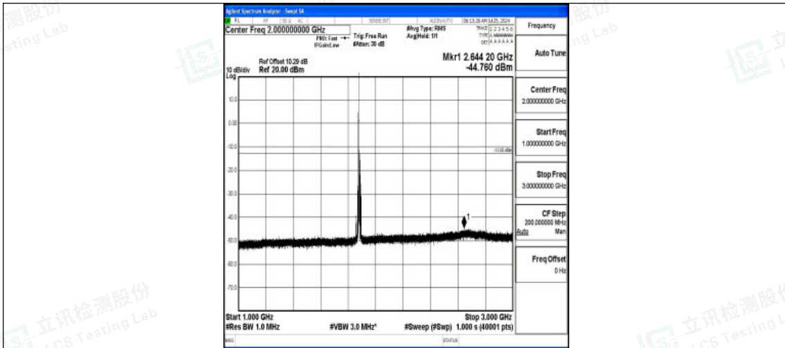
Band2-10MHz-16QAM-18900-1RB#0-1000~3000-PASS
