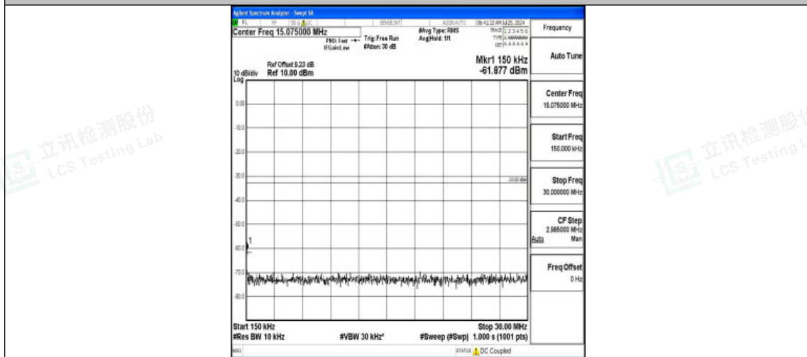
Band2-15MHz-QPSK-18900-1RB#0-0.15~30-PASS
