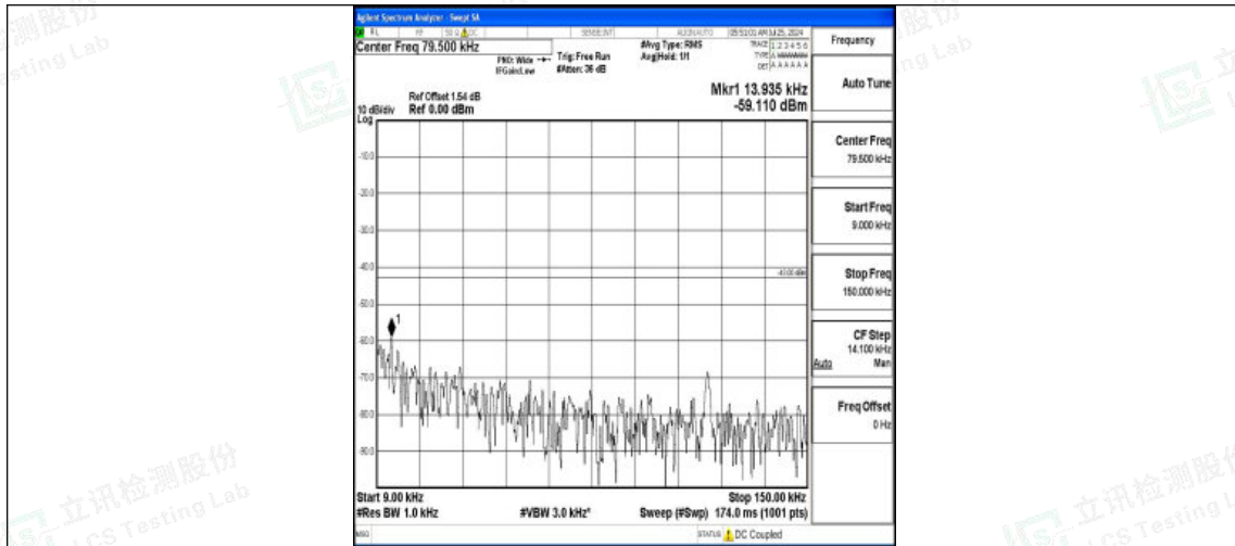
Band2-5MHz-16QAM-18900-1RB#0-0.009~0.15-PASS
