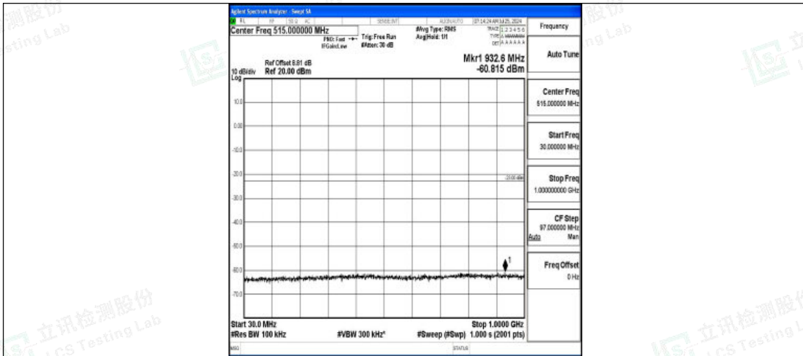
Band2-20MHz-QPSK-18900-1RB#0-30~1000-PASS
