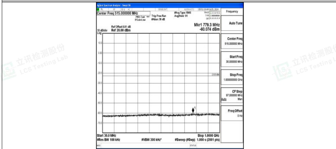
Band2-5MHz-16QAM-18900-1RB#0-30~1000-PASS
