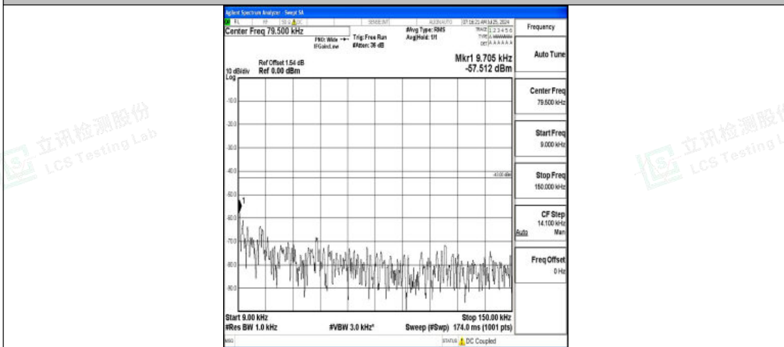
Band2-20MHz-QPSK-19100-1RB#0-0.009~0.15-PASS
