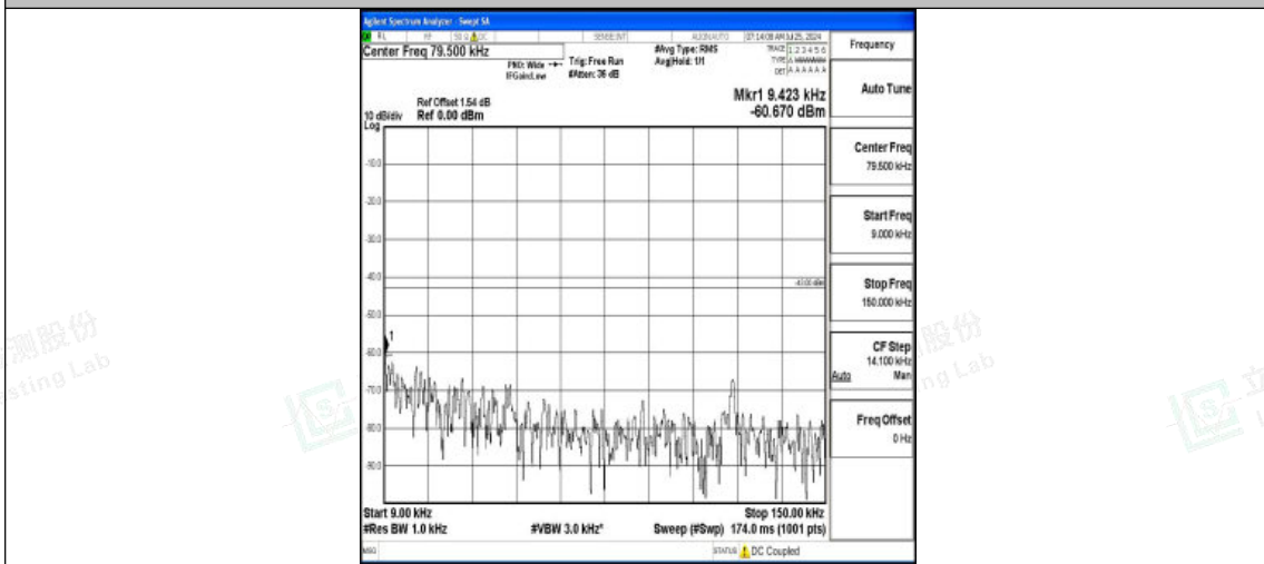
Band2-20MHz-QPSK-18900-1RB#0-0.009~0.15-PASS
