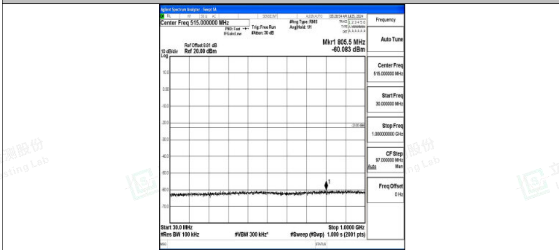
Band2-3MHz-QPSK-19185-1RB#0-30~1000-PASS
