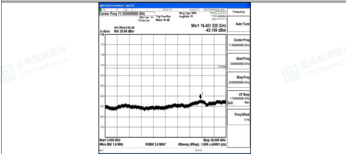
Band2-3MHz-QPSK-18900-1RB#0-3000~20000-PASS
