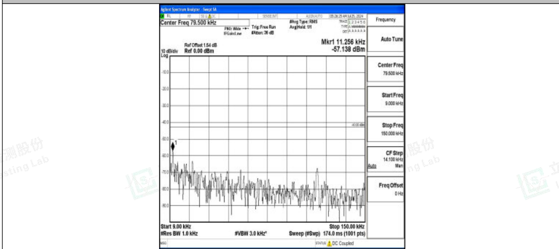
Band2-3MHz-QPSK-18900-1RB#0-0.009~0.15-PASS
