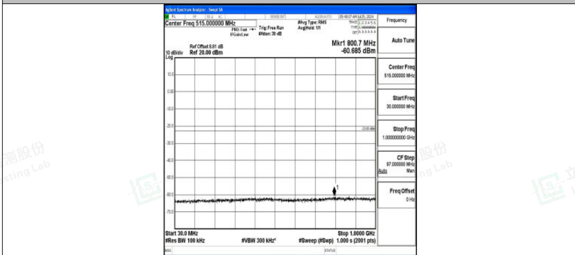
Band2-5MHz-16QAM-18625-1RB#0-30~1000-PASS
