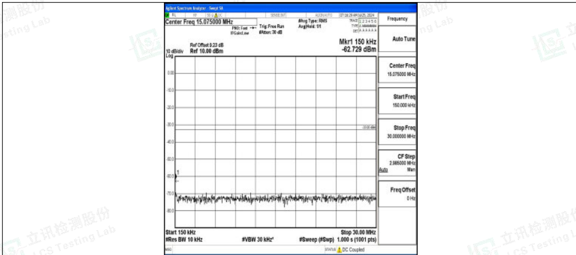
Band2-20MHz-QPSK-19100-1RB#0-0.15~30-PASS
