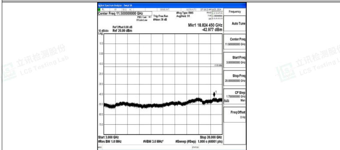
Band2-20MHz-16QAM-19100-1RB#0-3000~20000-PASS
