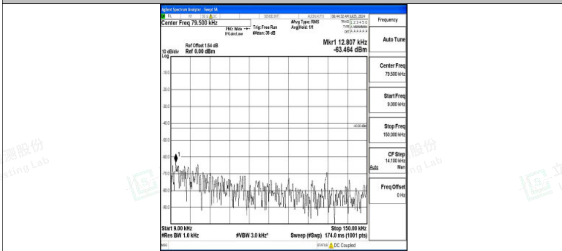
Band2-15MHz-16QAM-19125-1RB#0-0.009~0.15-PASS
