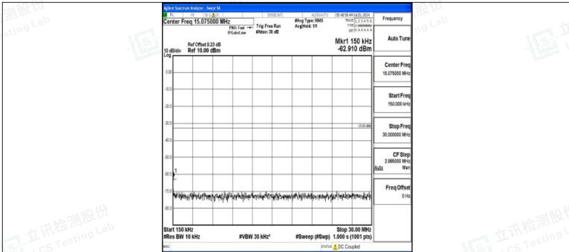
Band2-5MHz-16QAM-18625-1RB#0-0.15~30-PASS
