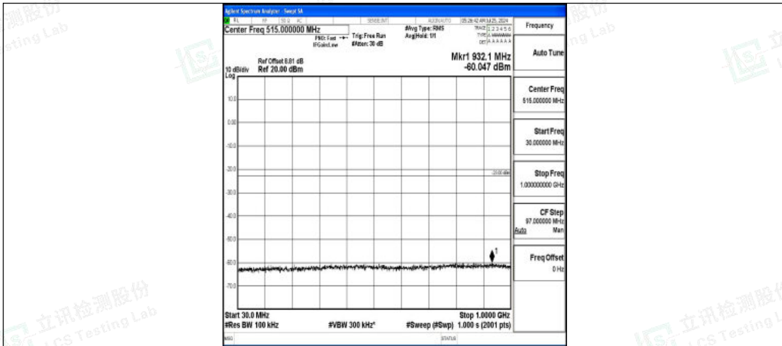
Band2-3MHz-QPSK-18900-1RB#0-30~1000-PASS
