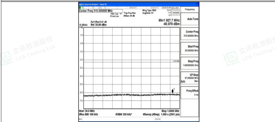
Band2-10MHz-QPSK-18650-1RB#0-30~1000-PASS
