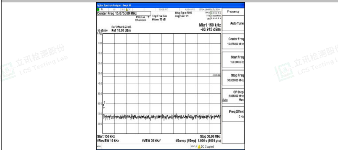
Band2-20MHz-QPSK-18900-1RB#0-0.15~30-PASS
