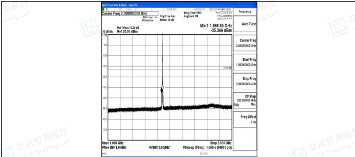
Band2-5MHz-16QAM-18900-1RB#0-1000~3000-PASS
