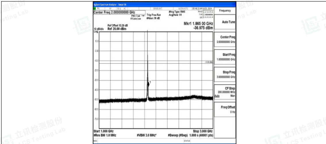
Band2-5MHz-QPSK-18625-1RB#0-1000~3000-PASS
