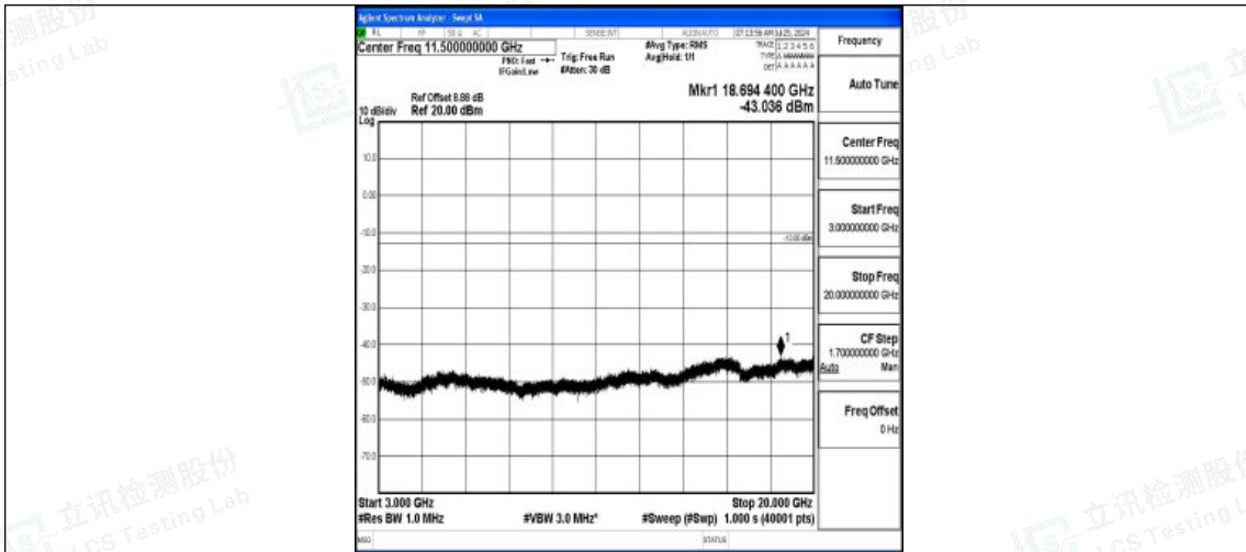
Band2-20MHz-16QAM-18700-1RB#0-3000~20000-PASS
