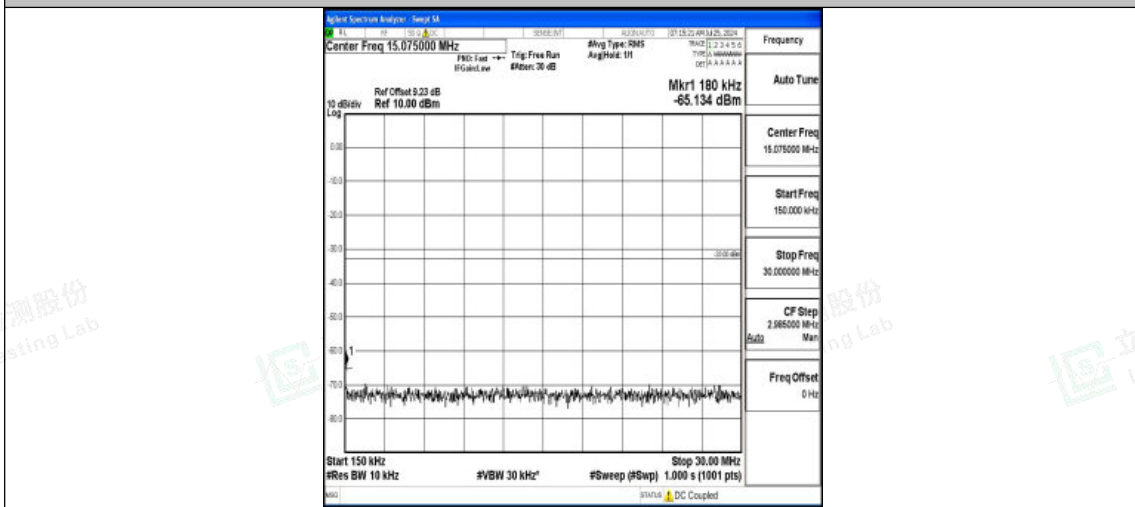
Band2-20MHz-16QAM-18900-1RB#0-0.15~30-PASS
