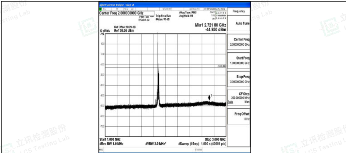
Band2-20MHz-16QAM-18900-1RB#0-1000~3000-PASS
