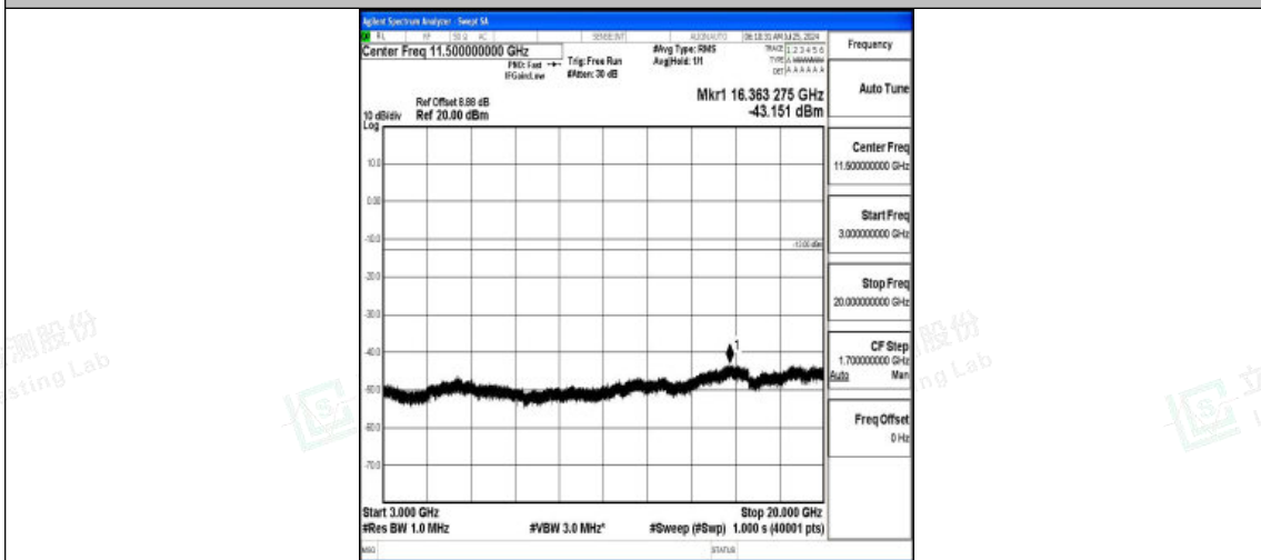
Band2-10MHz-QPSK-18650-1RB#0-3000~20000-PASS
