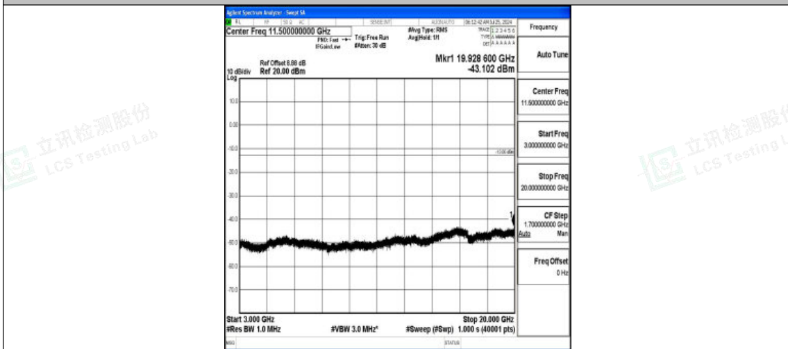
Band2-10MHz-QPSK-18900-1RB#0-3000~20000-PASS
