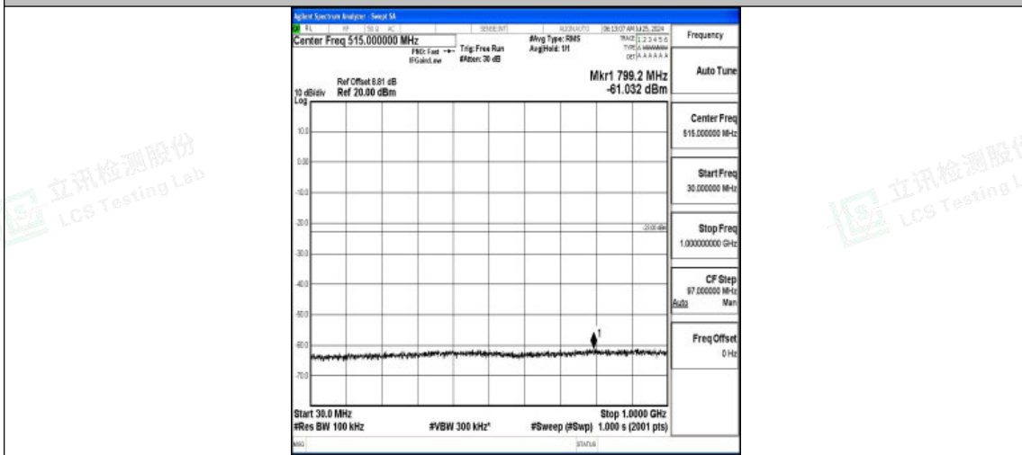
Band2-10MHz-16QAM-18900-1RB#0-30~1000-PASS
