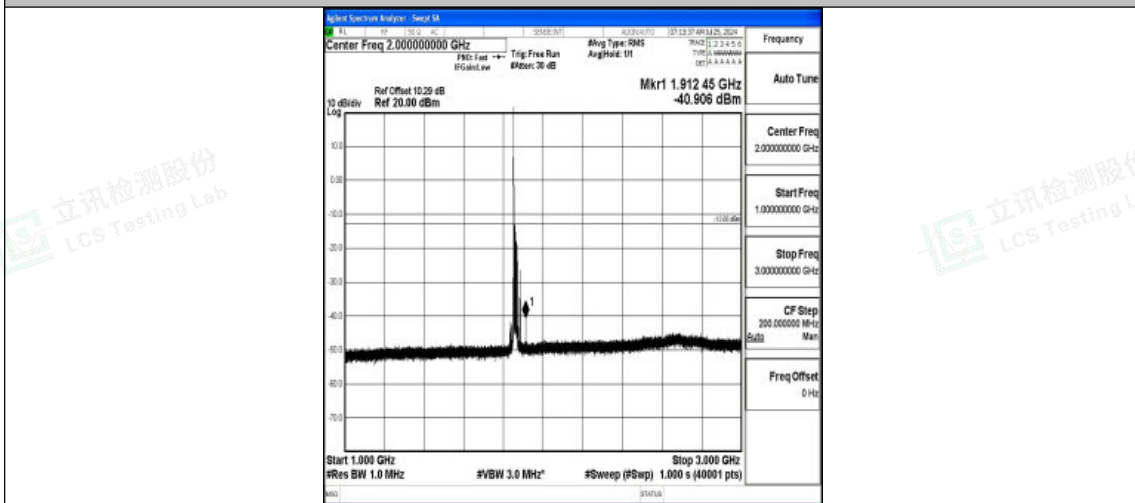
Band2-20MHz-16QAM-18700-1RB#0-1000~3000-PASS
