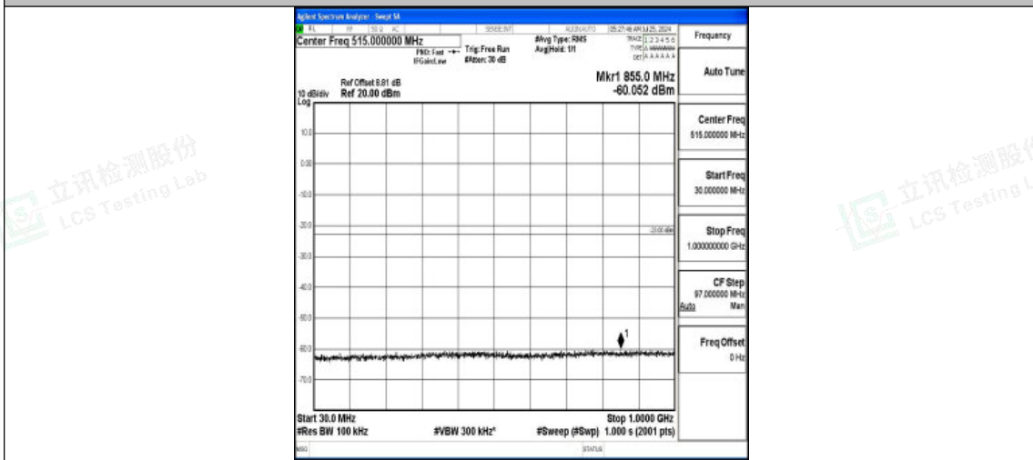
Band2-3MHz-16QAM-18900-1RB#0-30~1000-PASS
