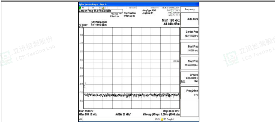
Band2-3MHz-QPSK-18900-1RB#0-0.15~30-PASS
