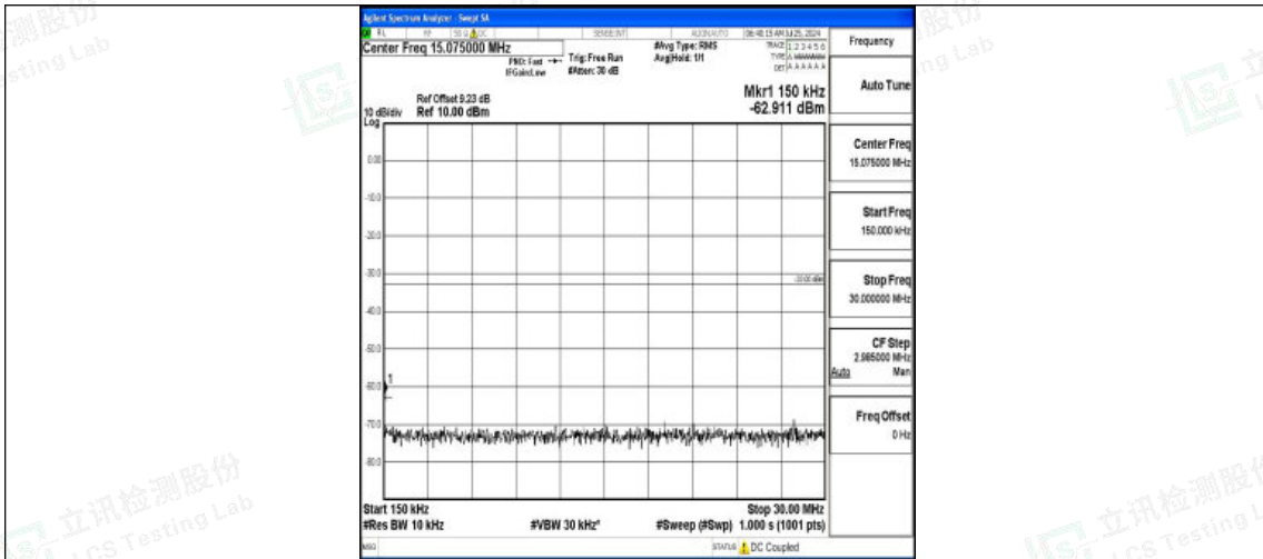
Band2-15MHz-16QAM-18675-1RB#0-0.15~30-PASS
