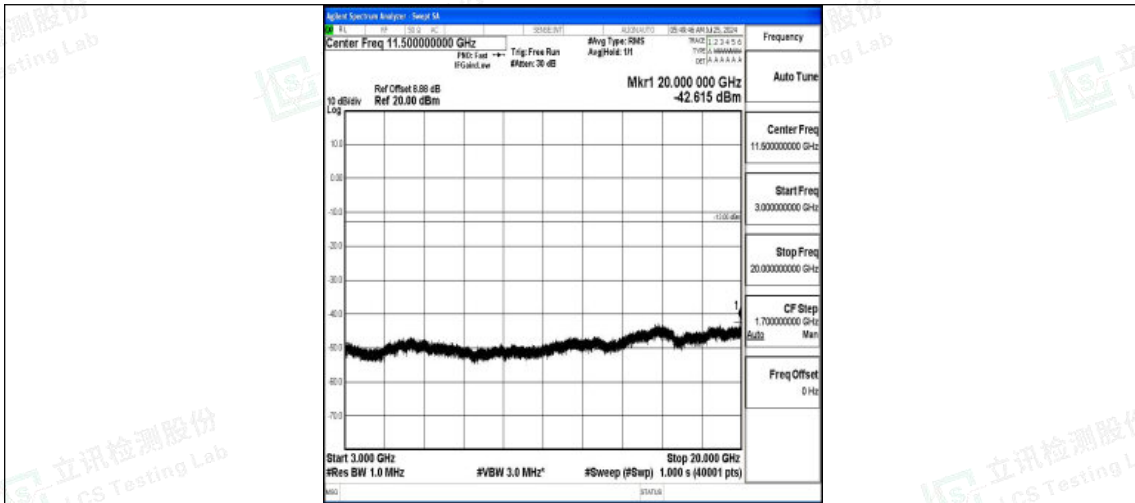
Band2-5MHz-16QAM-18625-1RB#0-3000~20000-PASS
