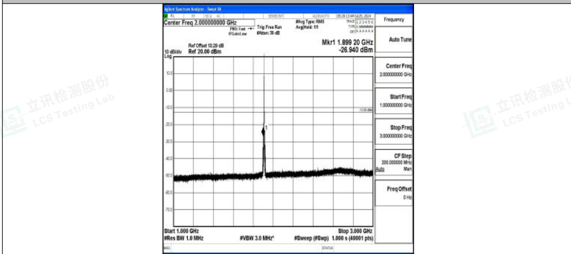
Band2-3MHz-QPSK-19185-1RB#0-1000~3000-PASS
