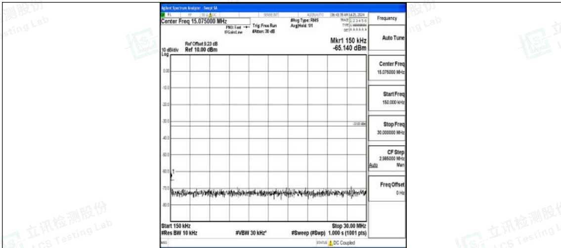
Band2-15MHz-QPSK-19125-1RB#0-0.15~30-PASS
