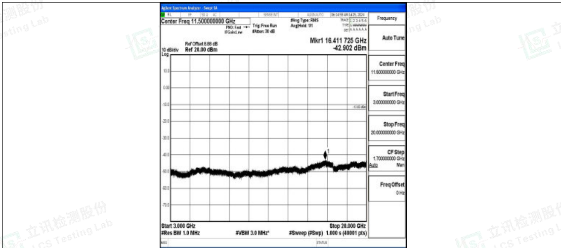
Band2-10MHz-QPSK-19150-1RB#0-3000~20000-PASS
