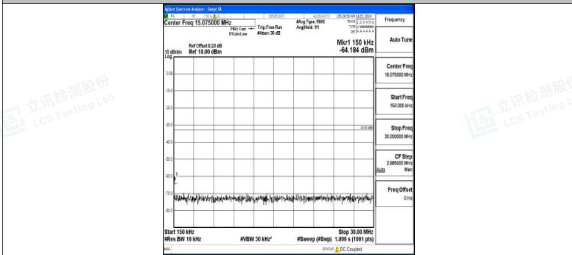
Band2-3MHz-16QAM-19185-1RB#0-0.15~30-PASS
