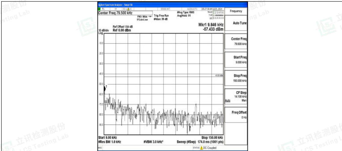
Band2-3MHz-16QAM-18900-1RB#0-0.009~0.15-PASS
