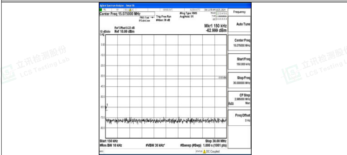
Band2-10MHz-QPSK-18900-1RB#0-0.15~30-PASS
