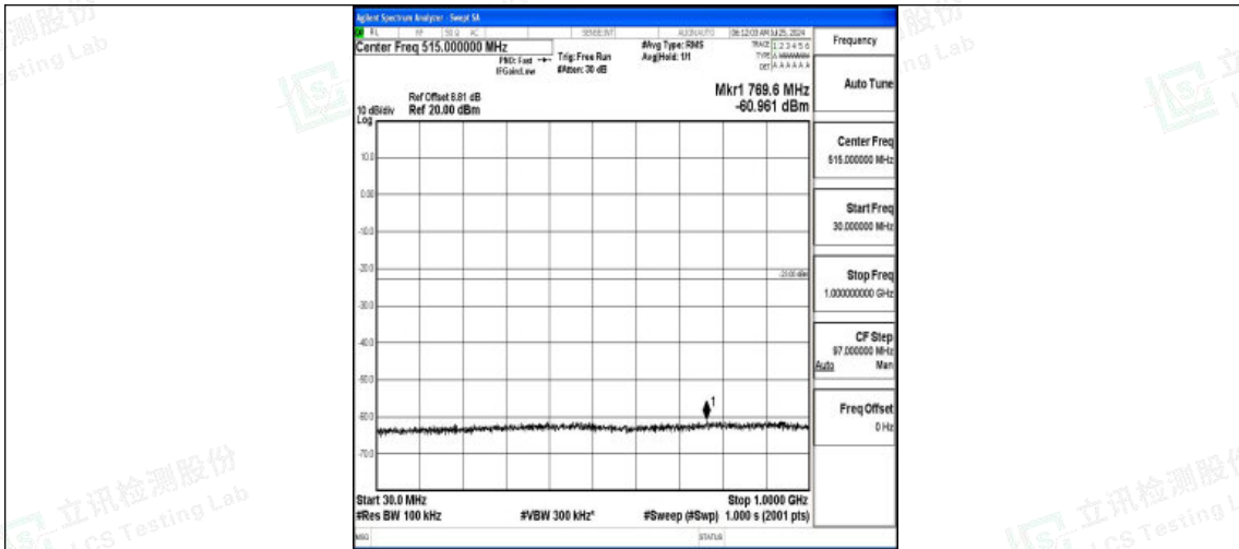
Band2-10MHz-QPSK-18900-1RB#0-30~1000-PASS
