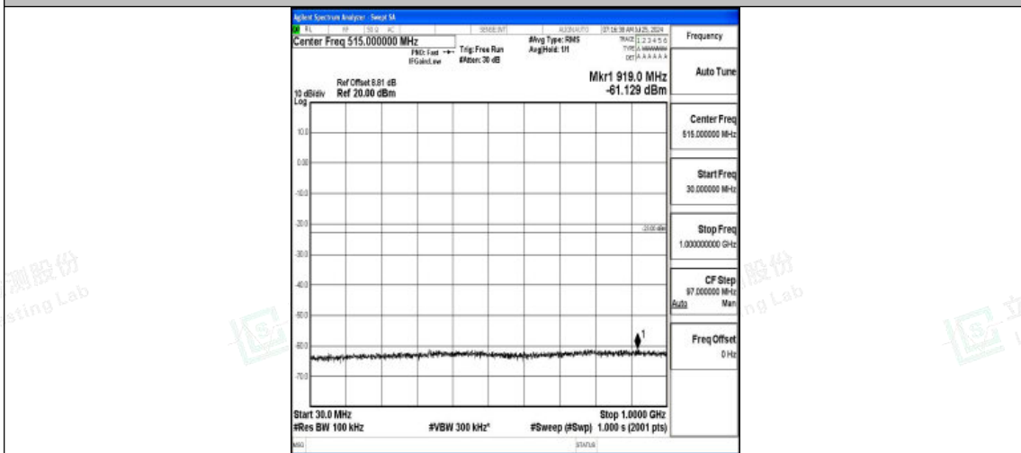
Band2-20MHz-QPSK-19100-1RB#0-30~1000-PASS
