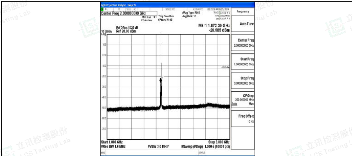
Band2-3MHz-16QAM-18900-1RB#0-1000~3000-PASS
