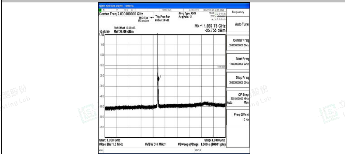
Band2-3MHz-QPSK-18900-1RB#0-1000~3000-PASS
