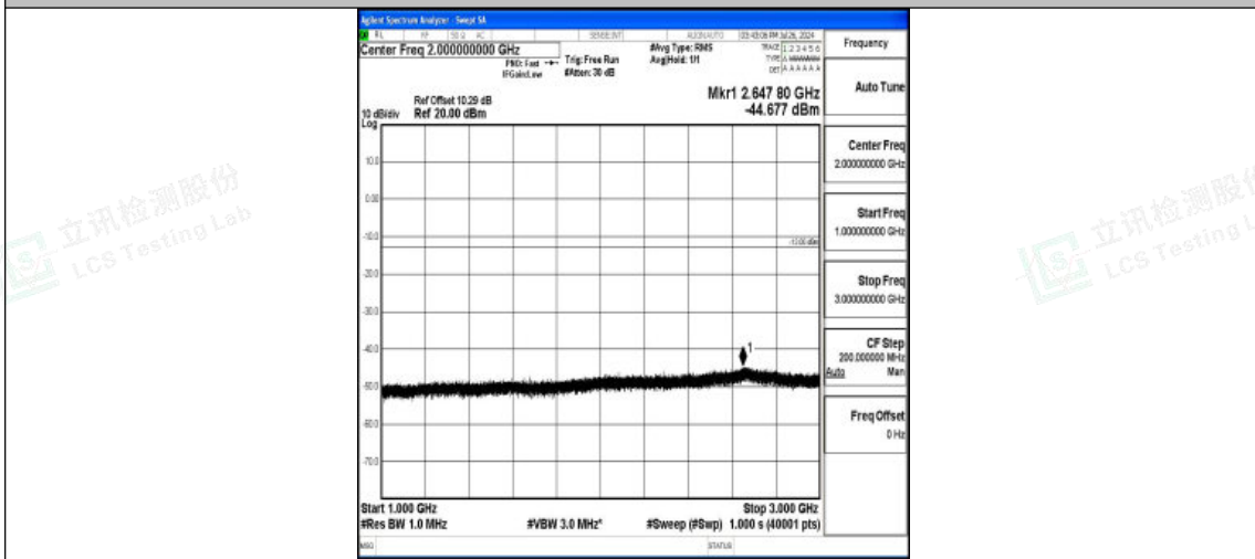
Band5-10MHz-QPSK-20600-1RB#0-1000~3000-PASS
