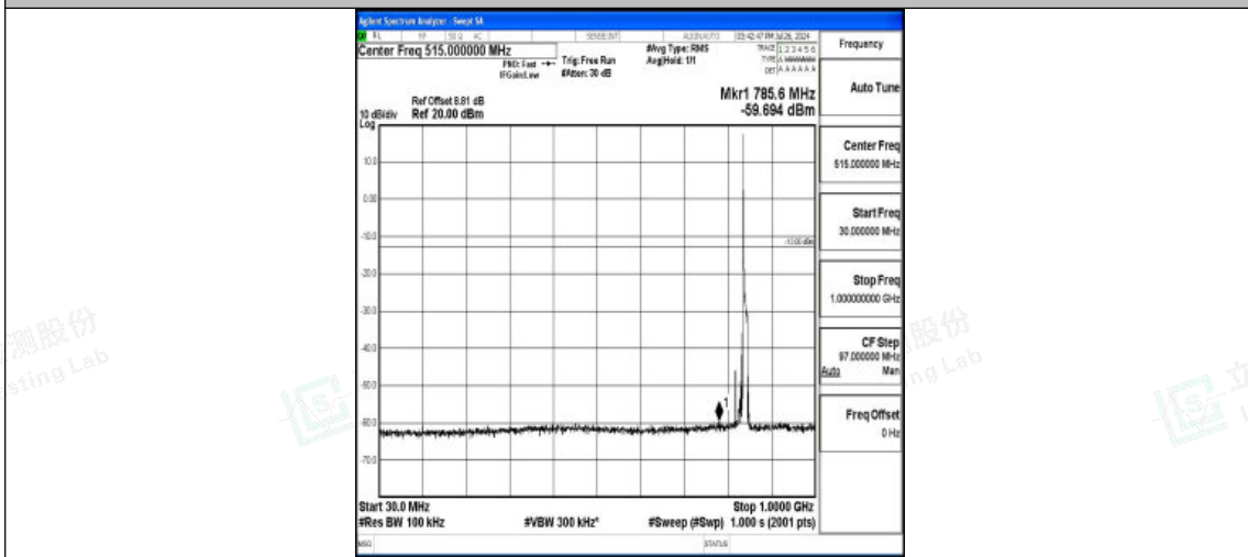
Band5-10MHz-QPSK-20600-1RB#0-30~1000-PASS
