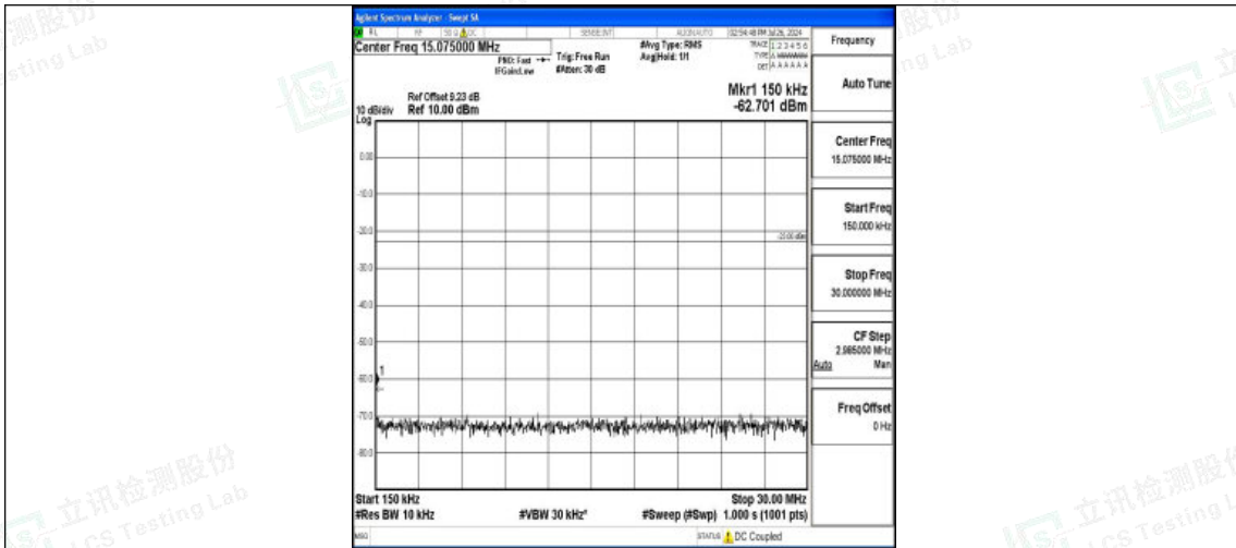
Band5-3MHz-16QAM-20415-1RB#0-0.15~30-PASS
