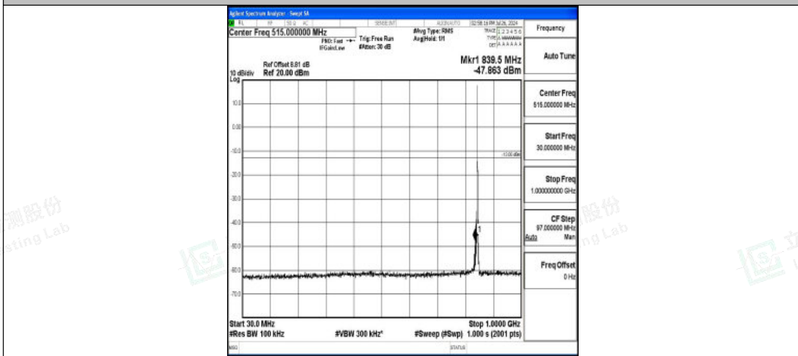
Band5-3MHz-QPSK-20635-1RB#0-30~1000-PASS
