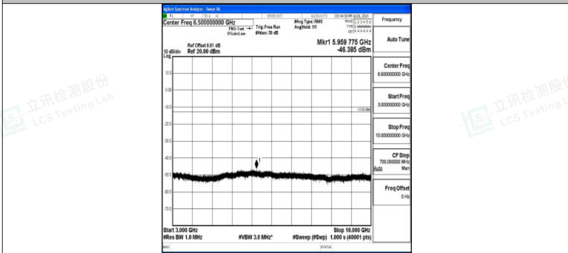
Band5-10MHz-16QAM-20600-1RB#0-3000~10000-PASS
