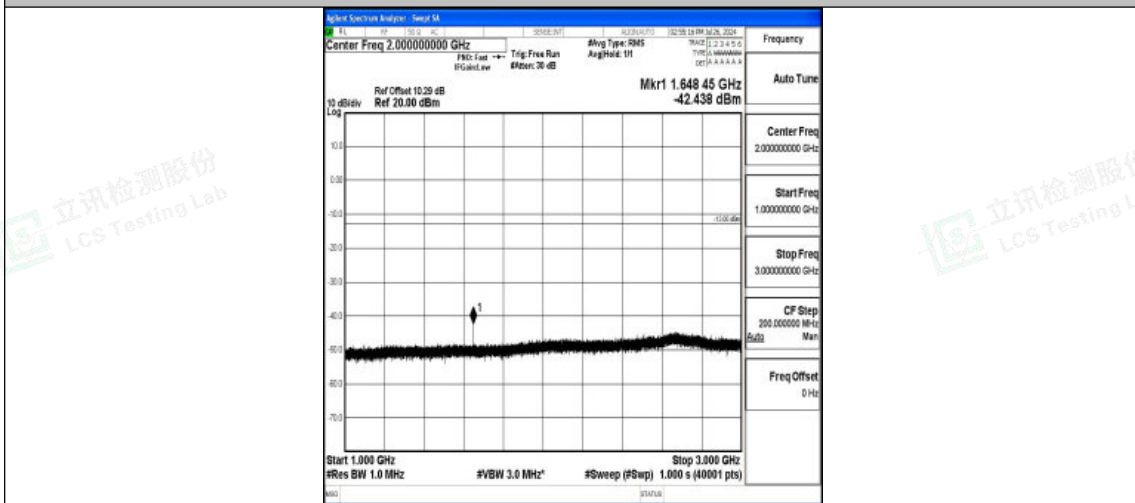
Band5-3MHz-16QAM-20415-1RB#0-1000~3000-PASS
