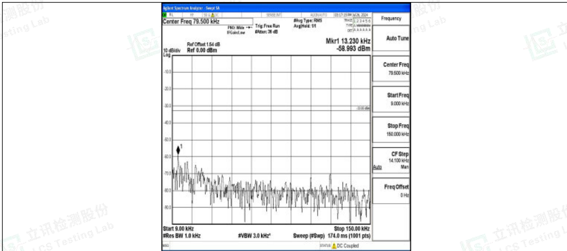
Band5-5MHz-QPSK-20425-1RB#0-0.15-PASS
