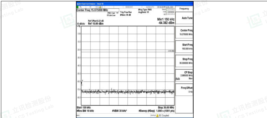
Band5-5MHz-16QAM-20425-1RB#0-0.15~30-PASS
