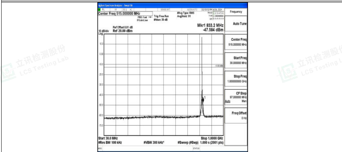
Band5-3MHz-QPSK-20415-1RB#0-30~1000-PASS
