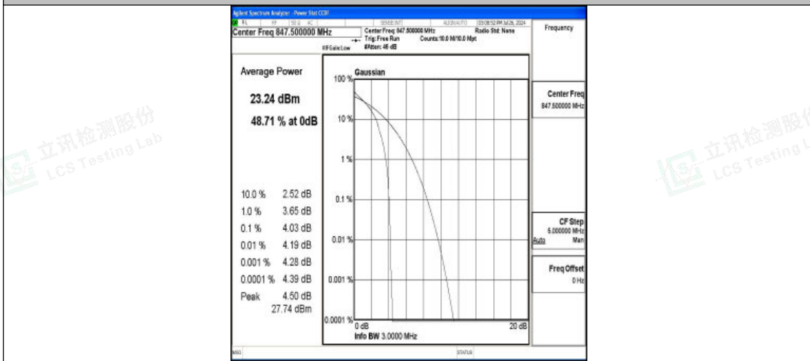
Band5-3MHz-QPSK-20635-1RB#0-PASS
