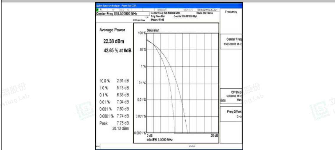
Band5-3MHz-16QAM-20525-15RB#0-PASS
