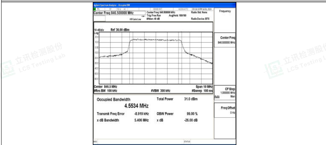
Band5-5MHz-16QAM-20625-25RB#0-PASS
