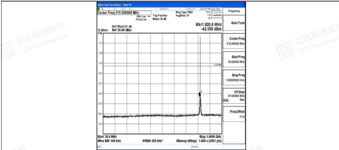
Band5-1.4MHz-QPSK-20407-1RB#0-30~1000-PASS
