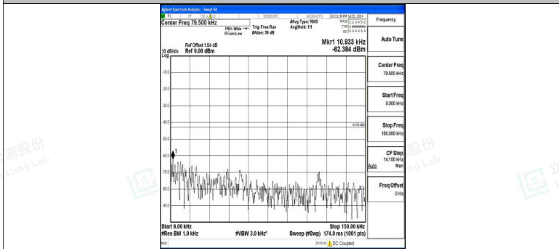
Band4-20MHz-16QAM-20300-1RB#0-0.009~0.15-PASS
