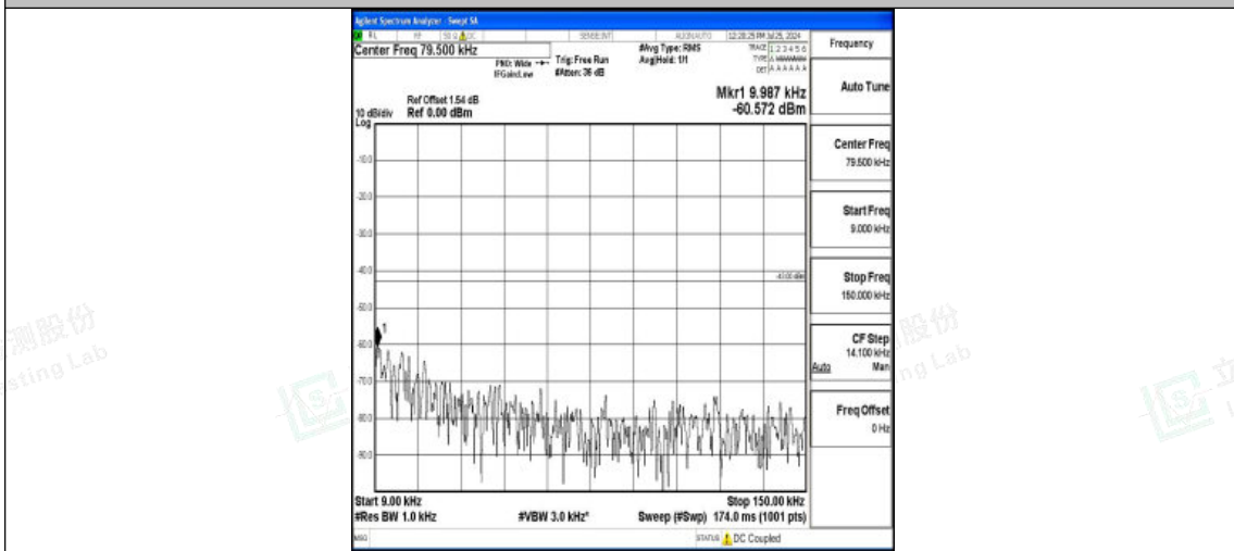
Band4-3MHz-QPSK-20175-1RB#0-0.009~0.15-PASS
