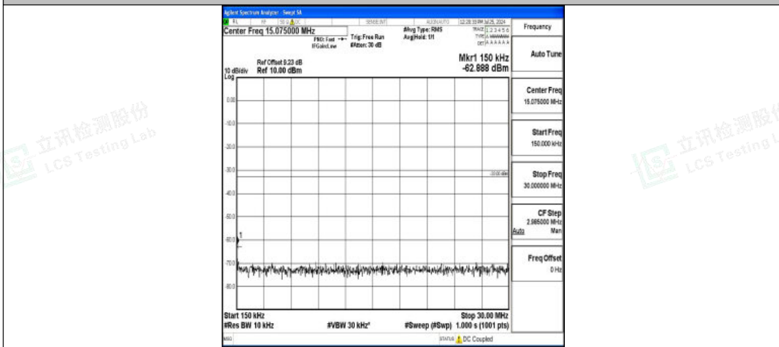
Band4-3MHz-QPSK-20175-1RB#0-0.15~30-PASS
