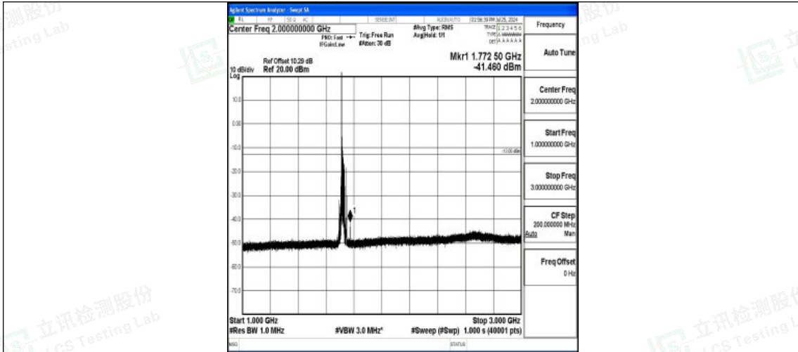
Band4-20MHz-QPSK-20050-1RB#0-1000~3000-PASS
