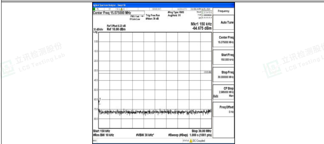
Band4-20MHz-QPSK-20175-1RB#0-0.15~30-PASS
