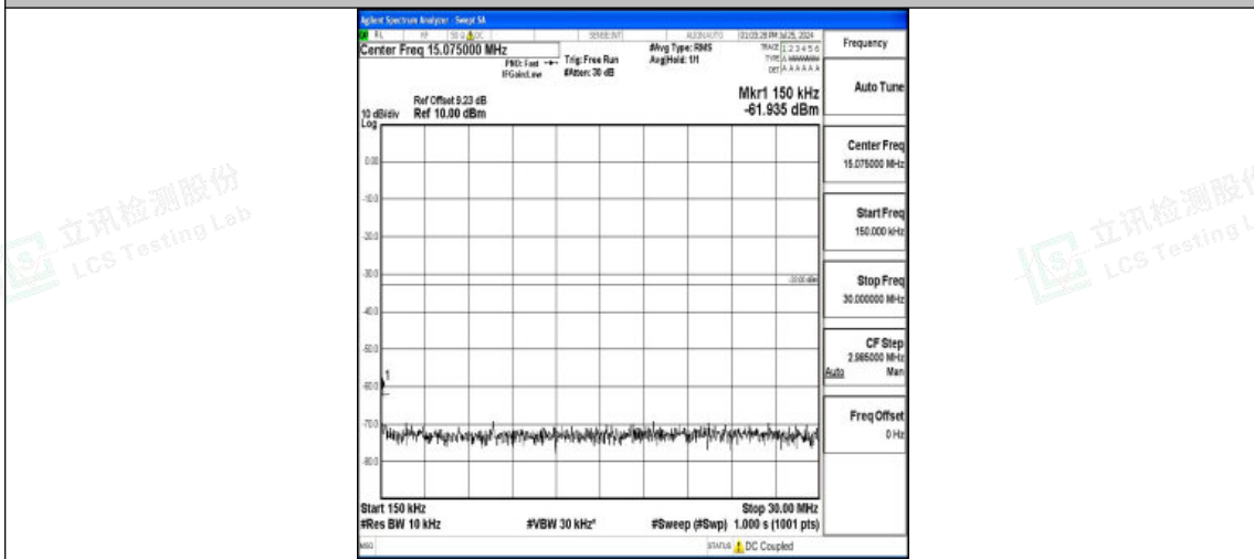
Band4-10MHz-16QAM-20350-1RB#0-0.15~30-PASS
