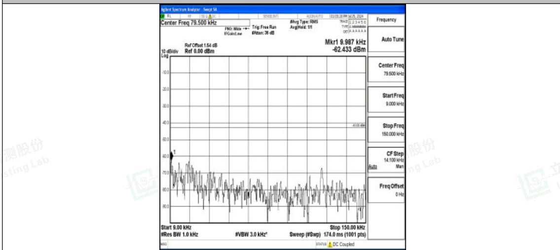
Band4-10MHz-16QAM-20350-1RB#0-0.009~0.15-PASS
