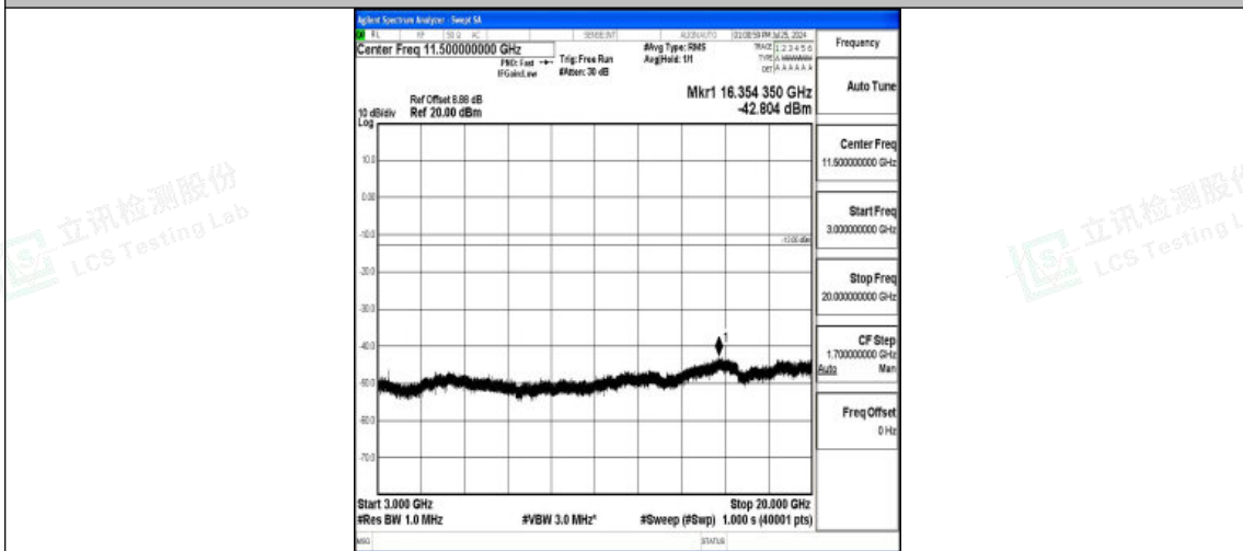
Band4-10MHz-QPSK-20175-1RB#0-3000~20000-PASS
