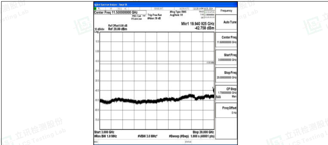
Band4-3MHz-16QAM-19965-1RB#0-3000~20000-PASS
