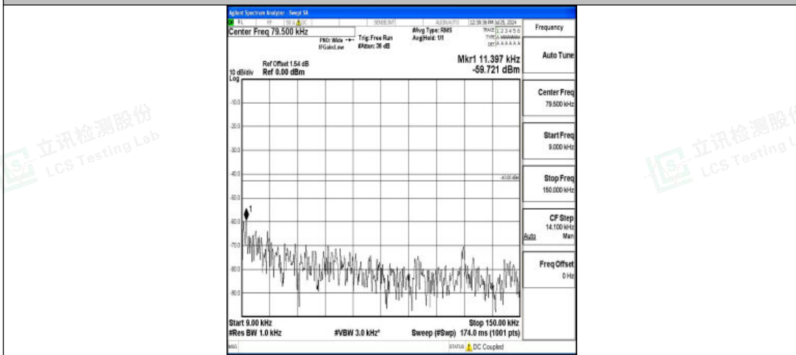
Band4-5MHz-16QAM-19975-1RB#0-0.009~0.15-PASS
