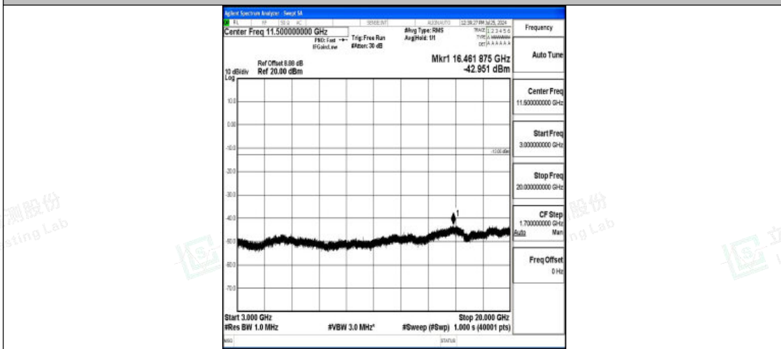
Band4-5MHz-QPSK-19975-1RB#0-3000~20000-PASS
