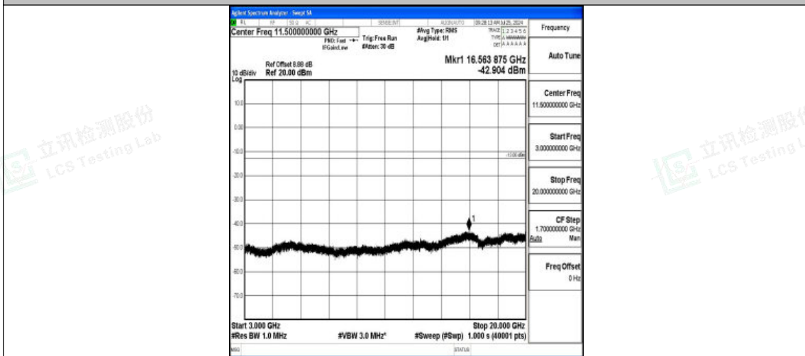
Band2-3MHz-QPSK-18900-1RB#0-3000~20000-PASS
