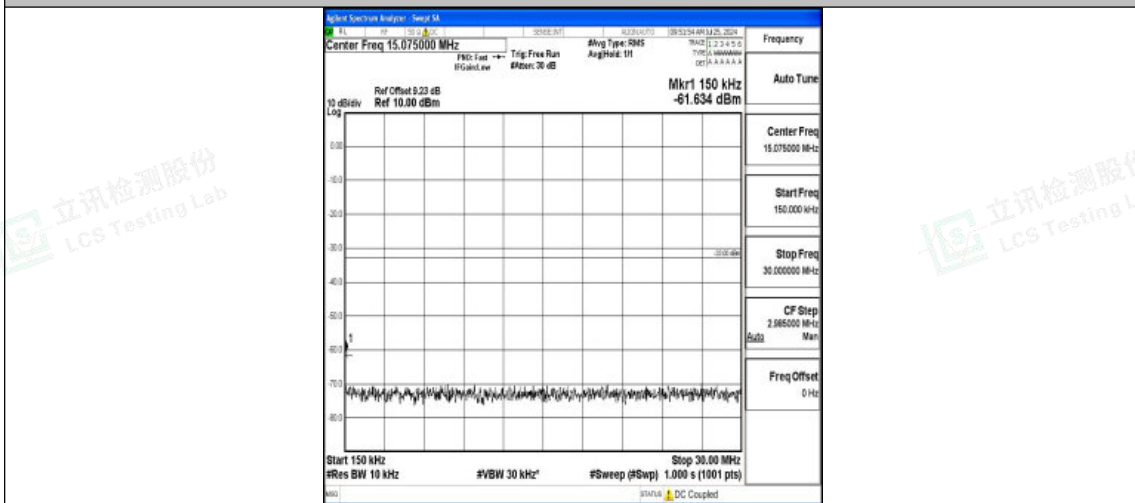
Band2-5MHz-16QAM-19175-1RB#0-0.15~30-PASS
