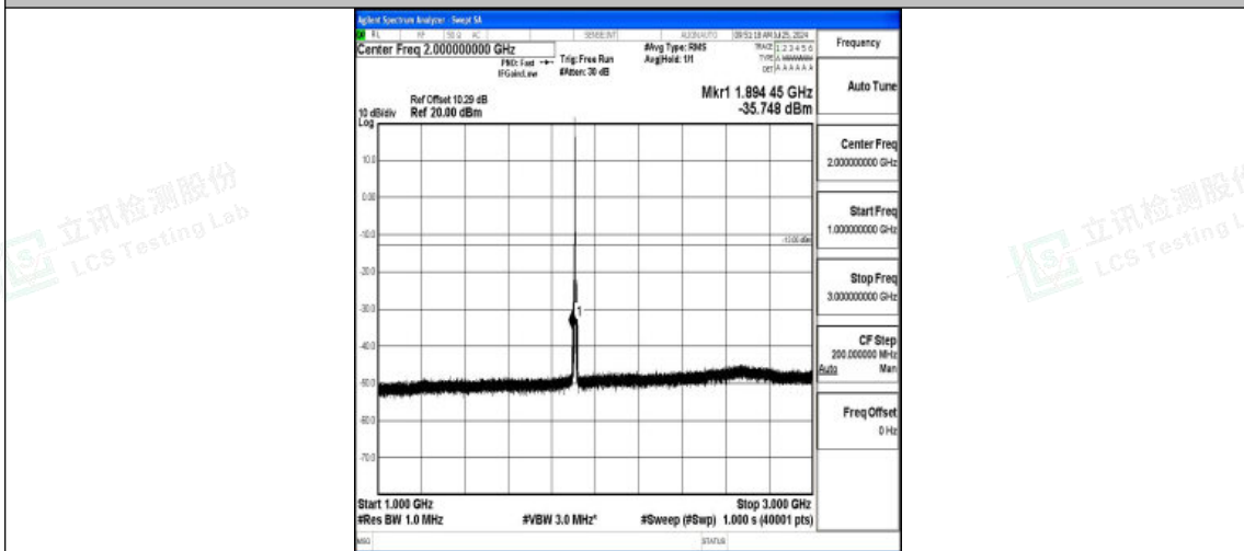
Band2-5MHz-QPSK-19175-1RB#0-1000~3000-PASS
