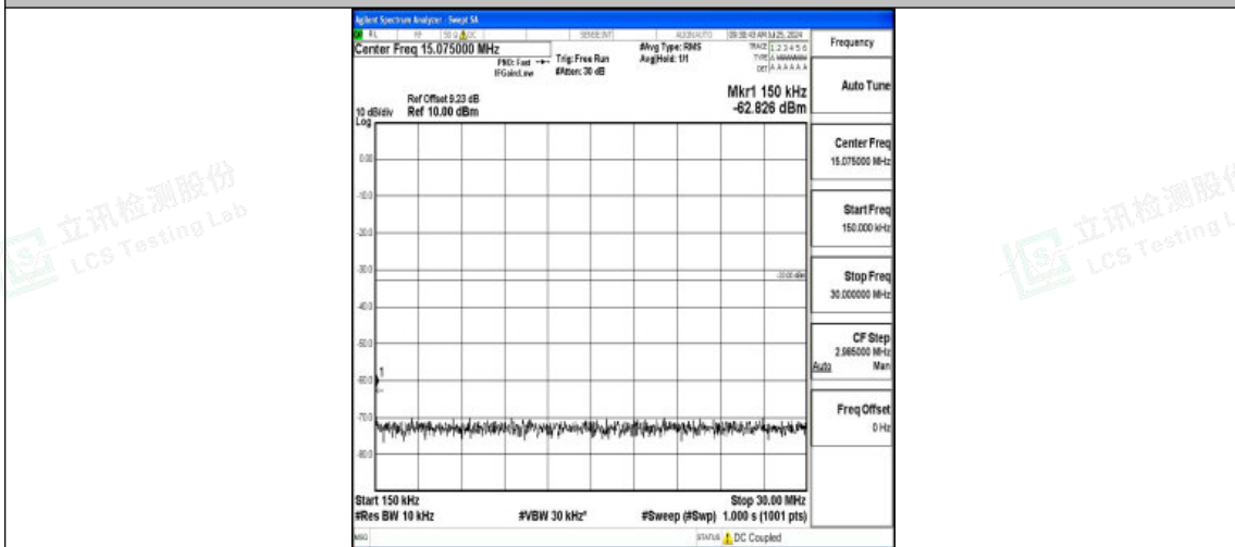
Band2-3MHz-16QAM-19185-1RB#0-0.15~30-PASS
