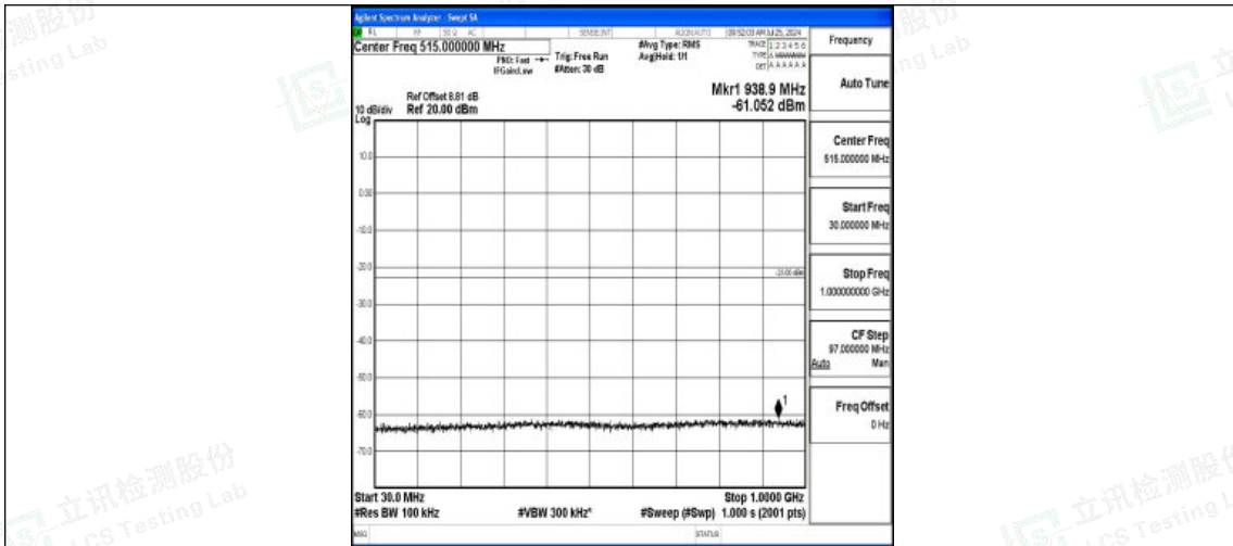
Band2-5MHz-16QAM-19175-1RB#0-30~1000-PASS
