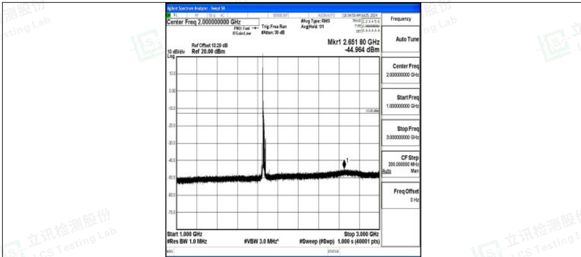
Band2-15MHz-QPSK-18675-1RB#0-1000~3000-PASS
