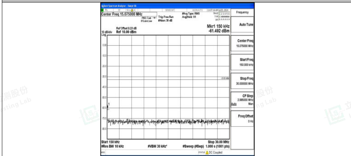
Band2-20MHz-QPSK-18700-1RB#0-0.15~30-PASS
