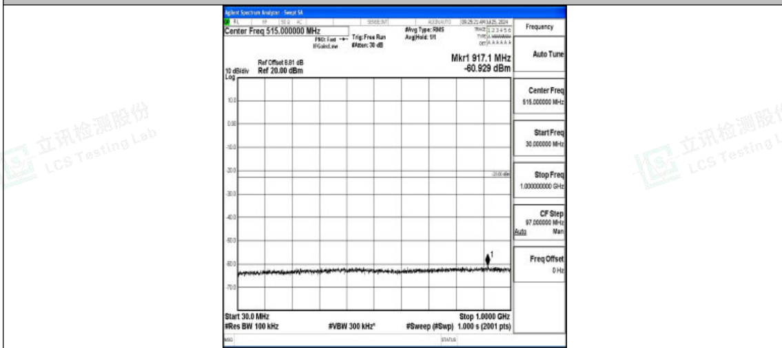
Band2-3MHz-QPSK-18615-1RB#0-30~1000-PASS
