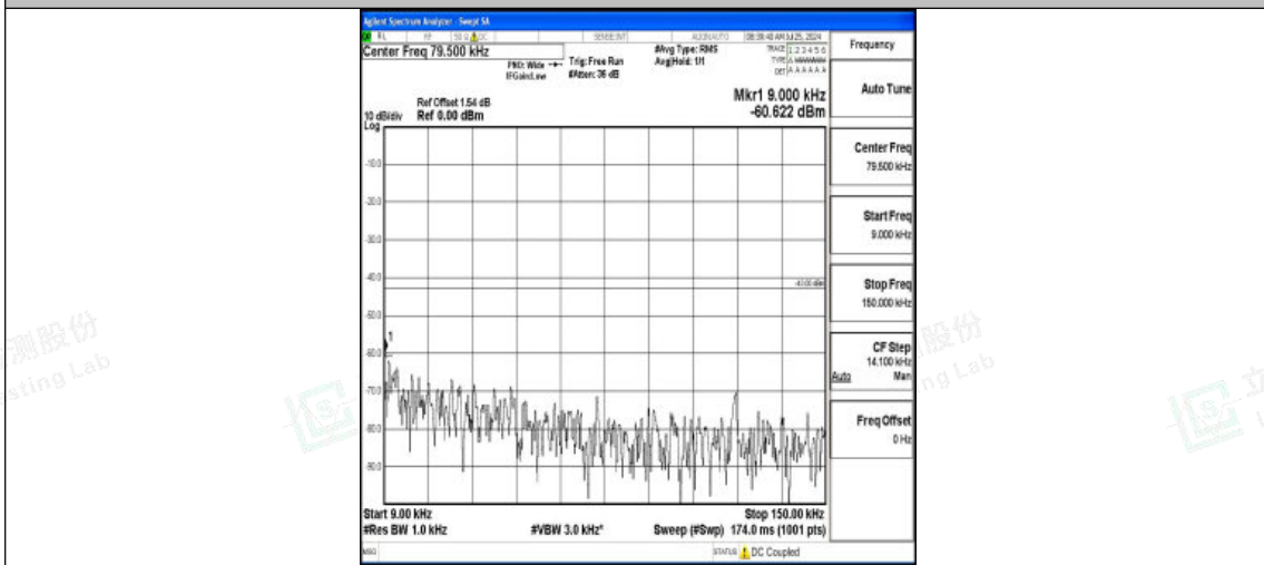
Band2-1.4MHz-16QAM-19193-1RB#0-0.009~0.15-PASS
