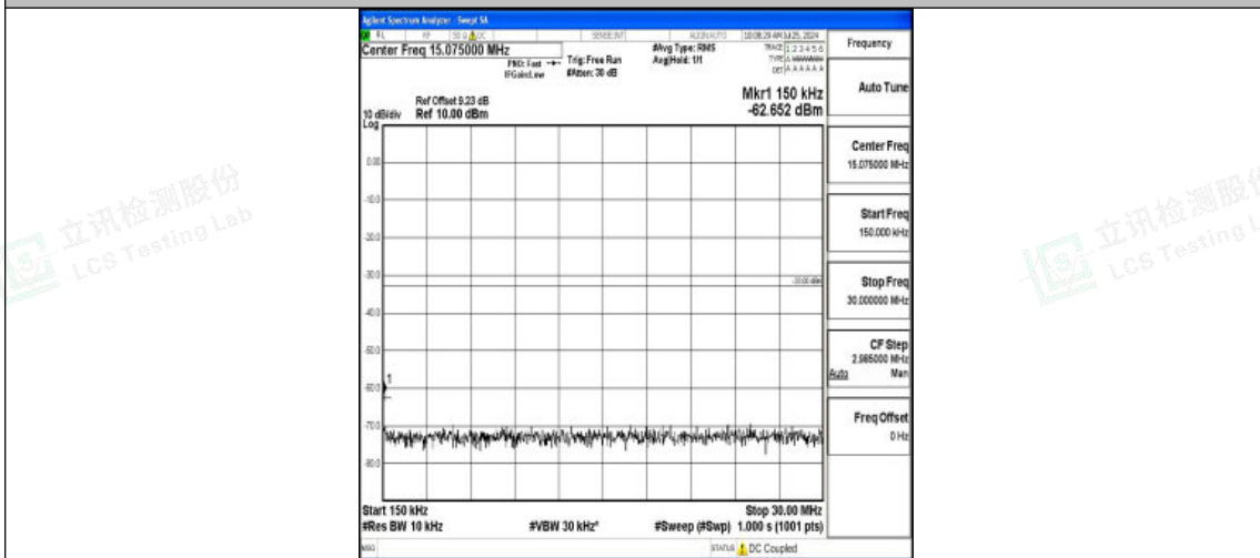
Band2-10MHz-QPSK-18900-1RB#0-0.15~30-PASS
